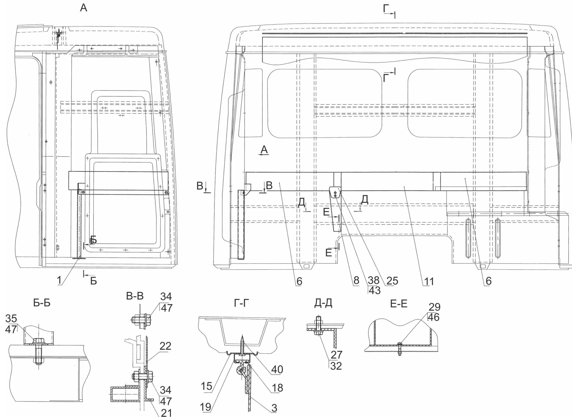
Fig. 255 Installation of a berths 5440-8200010
