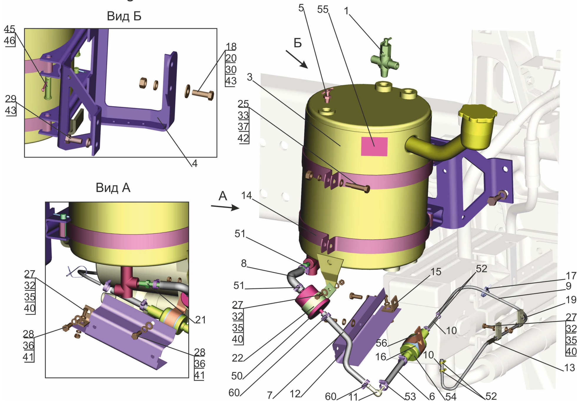
Fig. 7 Fuel lines of heater 544019-1015004
