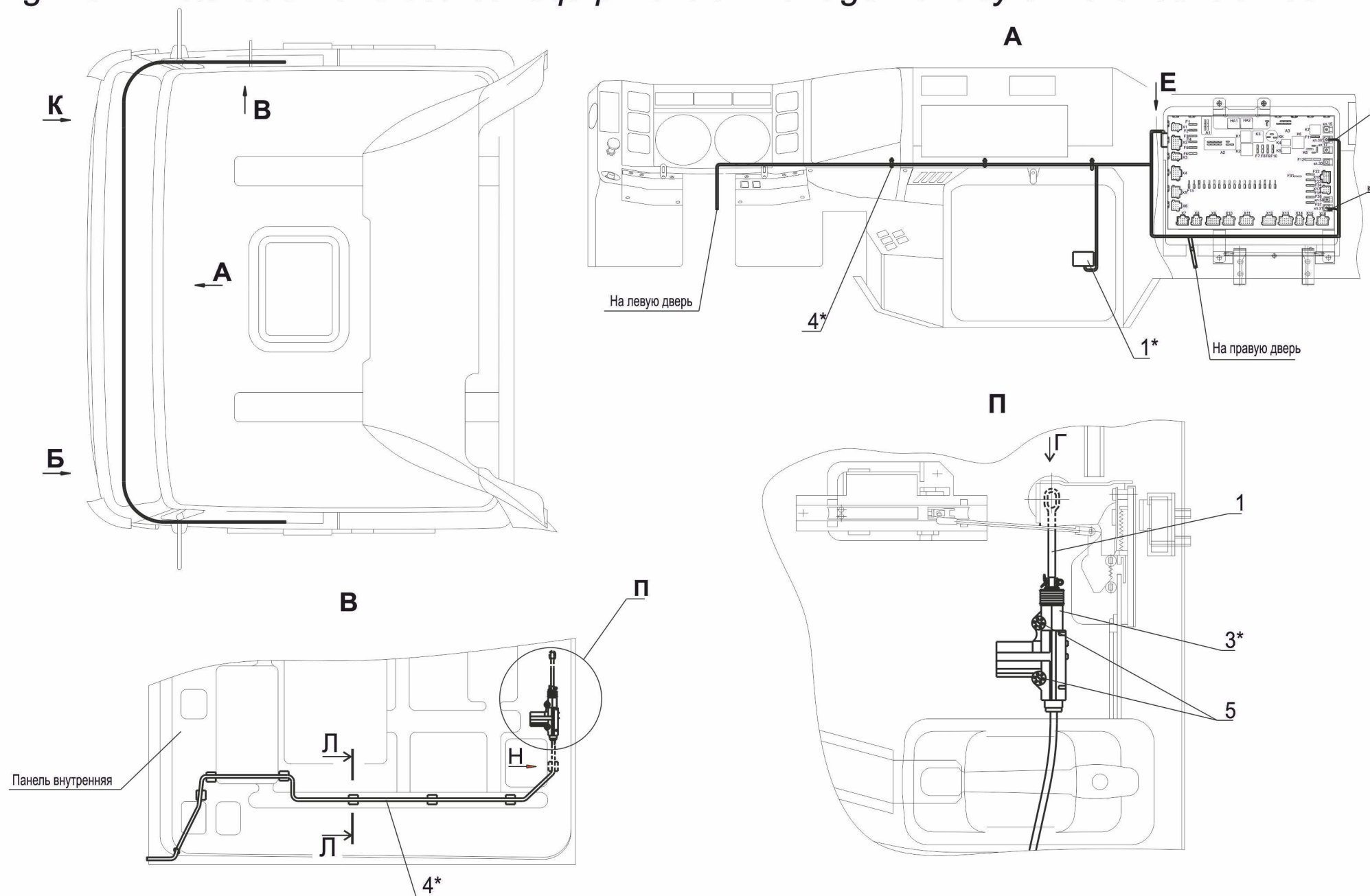
Fig. 191 Installation of electrical equipment of management by drive of central lock
