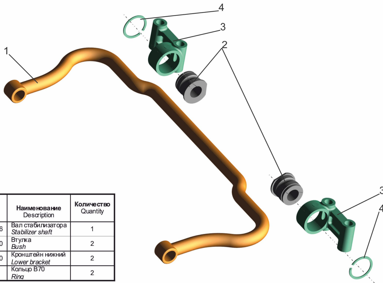
Fig. 110 Stabilizer shaft with brackets 6430-2906006
