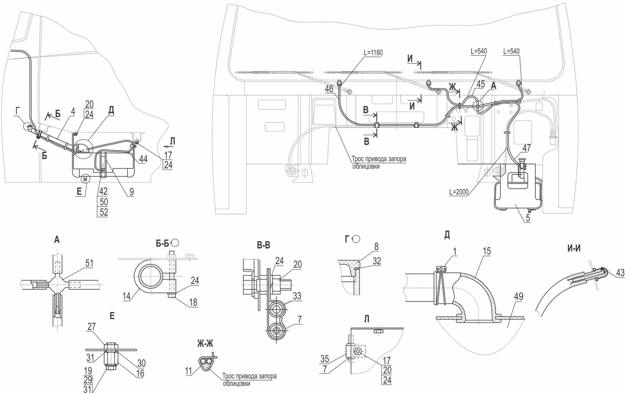
Fig. 235 Installation of washer 6430-5200008
