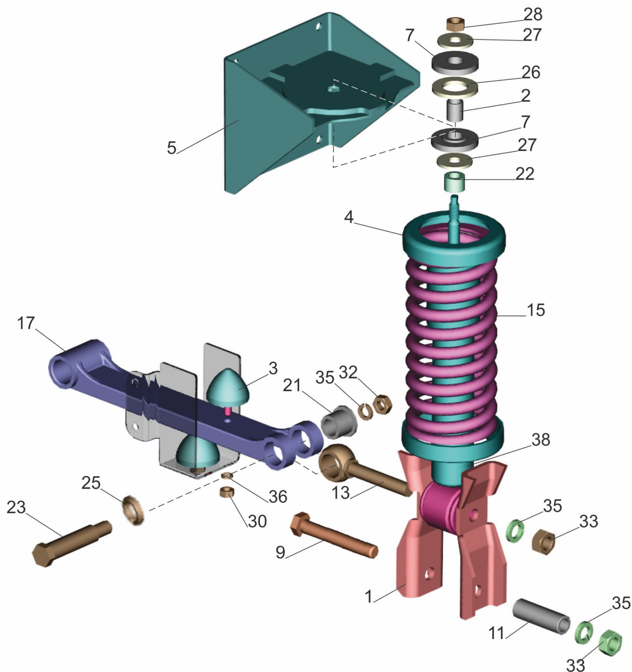
Fig.224 Cab rear springing 6501-5001802-010
