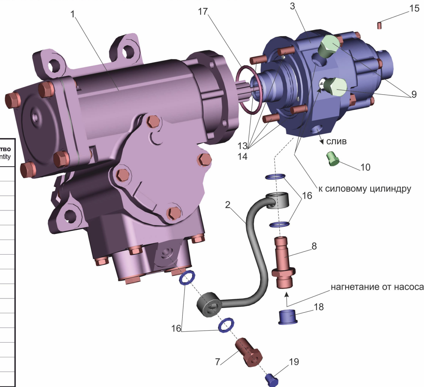
Fig. 144 Steer with the allocator 64221-3400010-10
