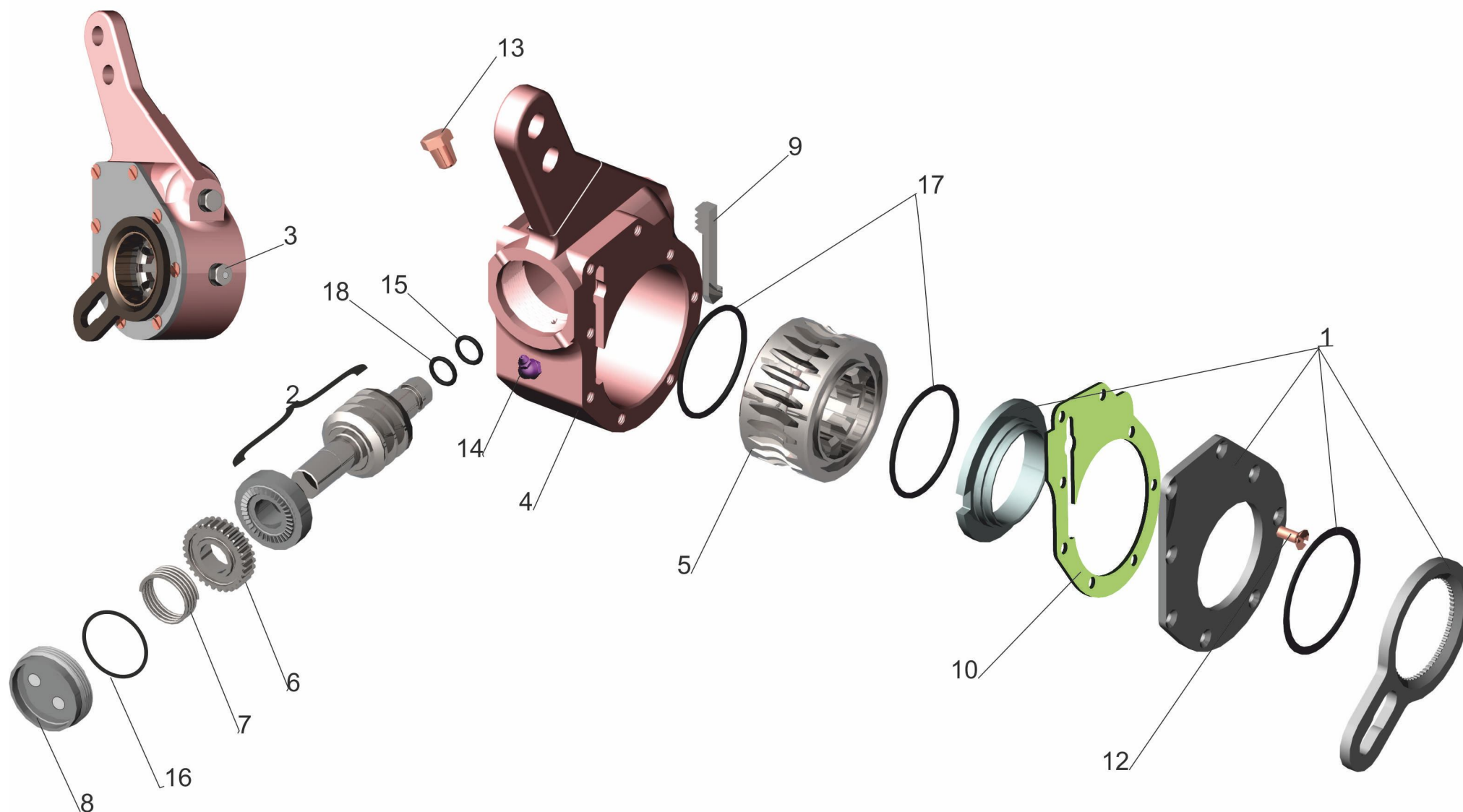
Fig. 134 Adjusting lever 103-3501136-10
