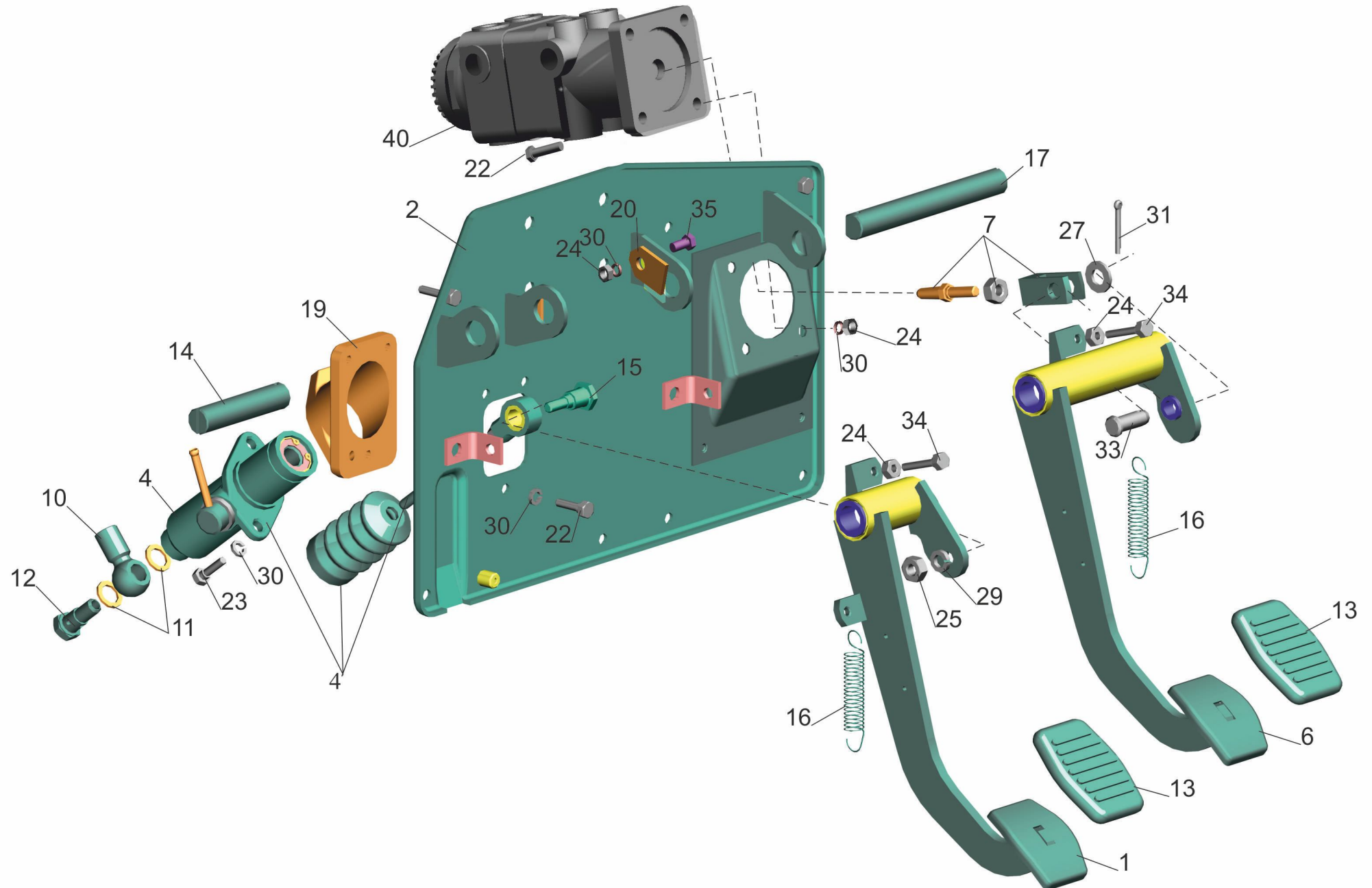
Fig. 35 Clutch and brake control unit 555035-1602004-010
