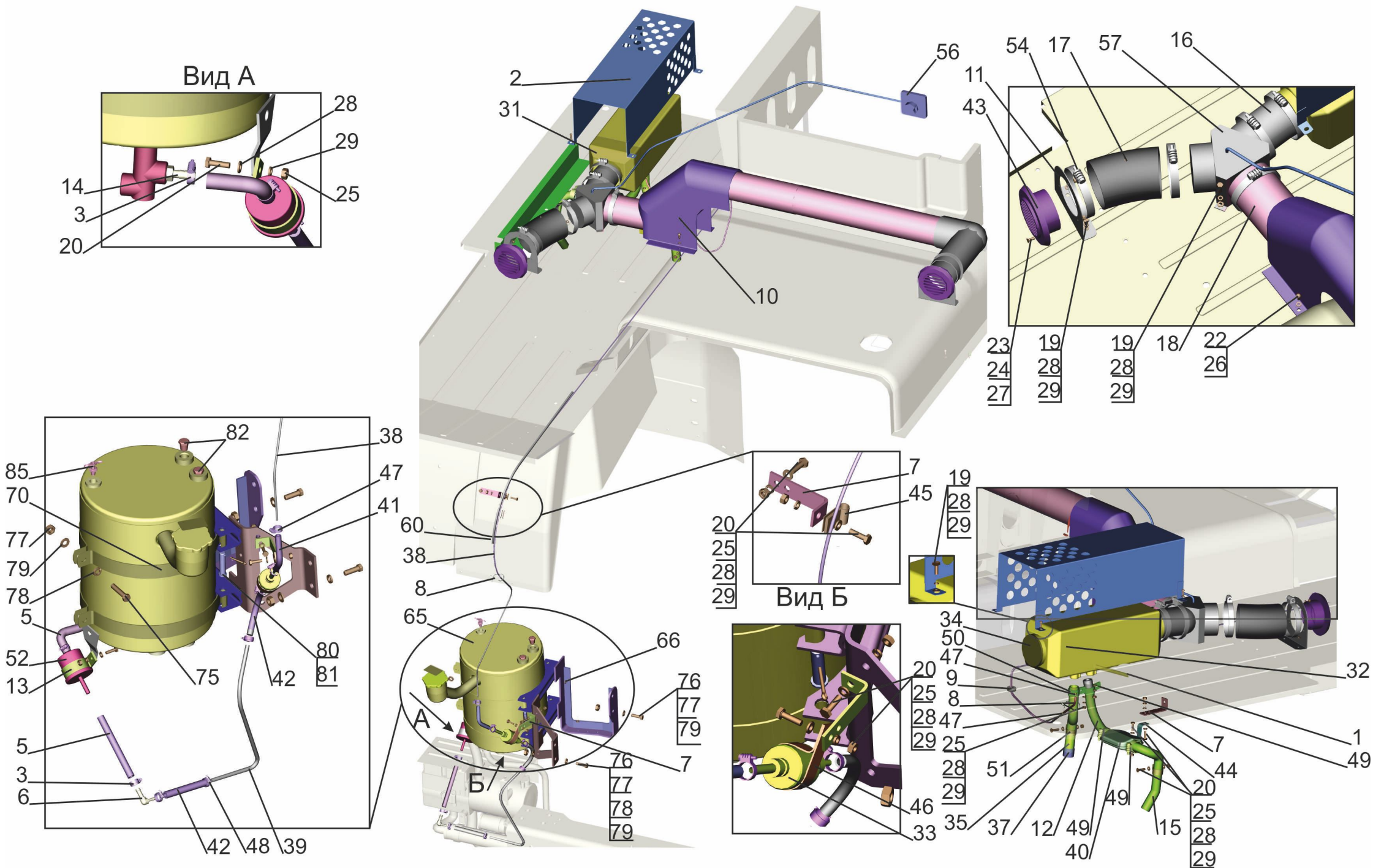
Fig. 289 Installation of the independent air heater 544019-8100002-010
