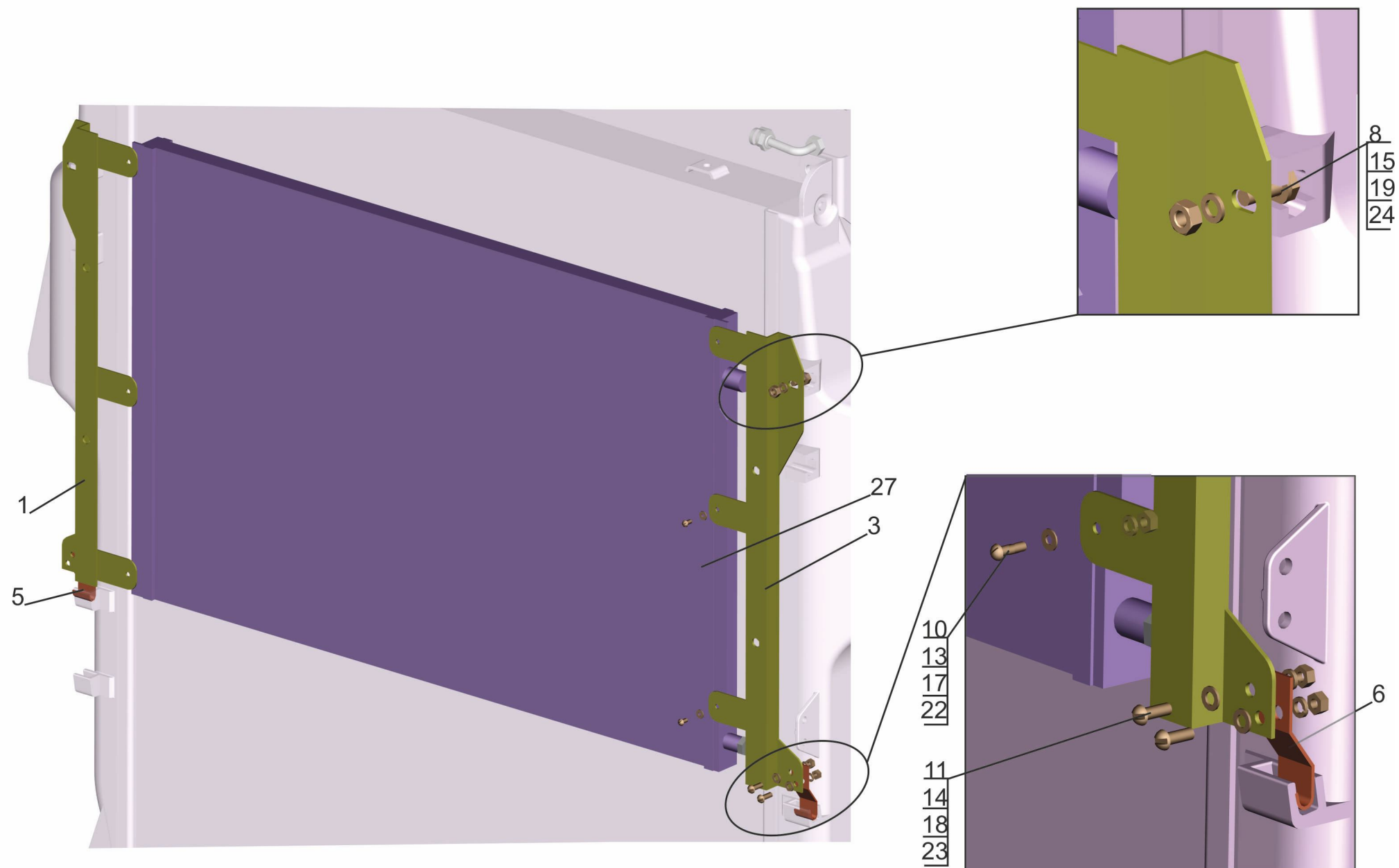
Fig. 297 Installation of capacitor 544019-8100034
