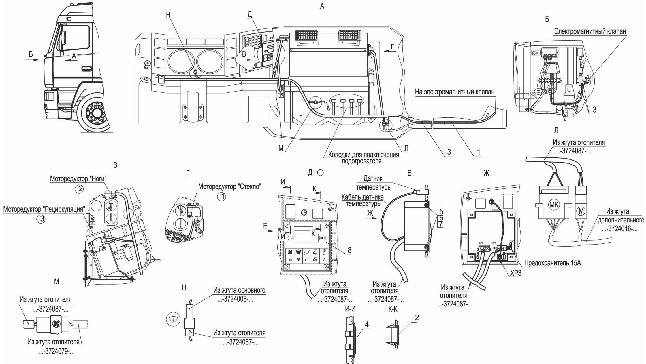
Fig. 288 Installation of an electric equipment of management microclimate 5440-3700103-010
