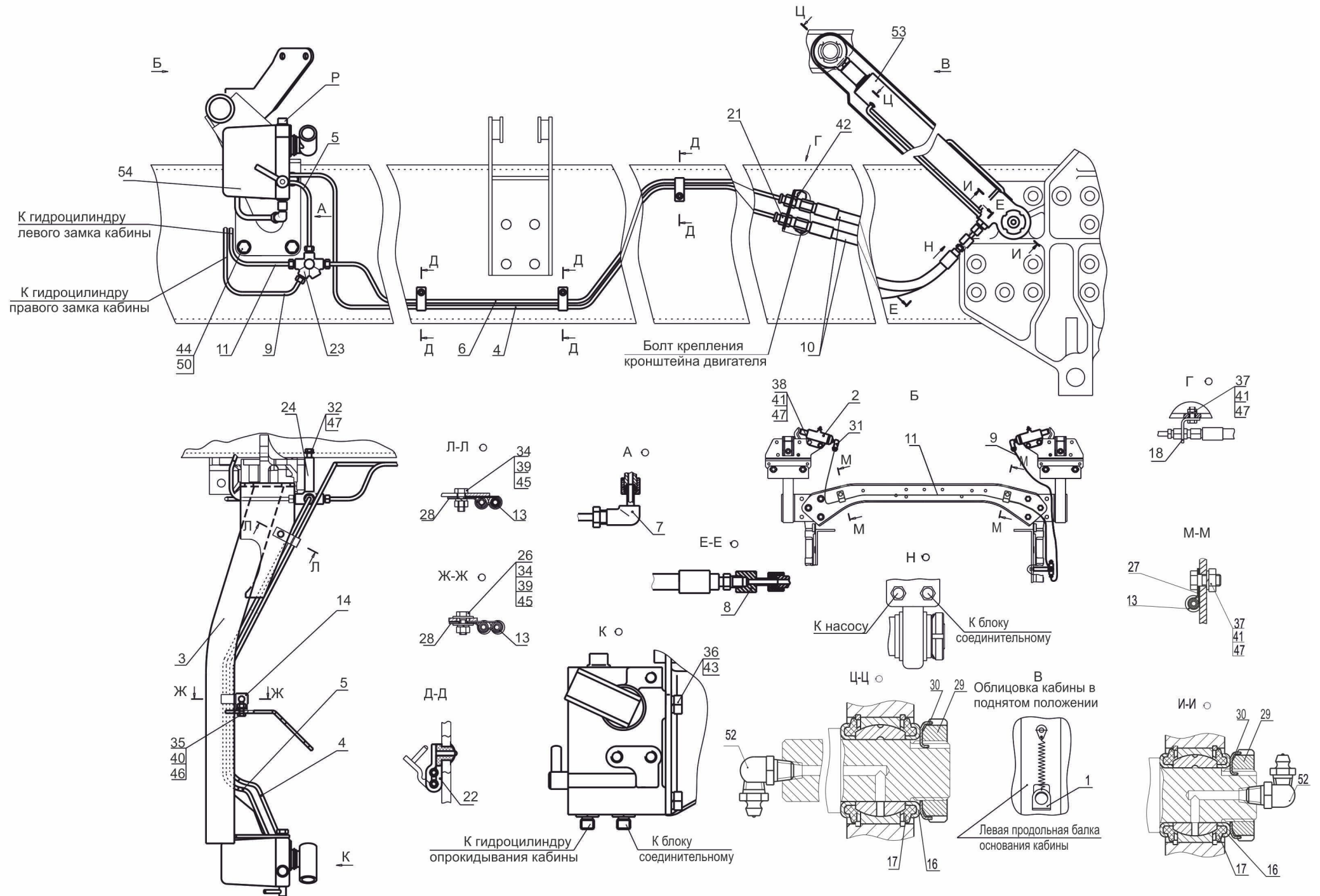
Fig. 269 Installation cab tilting mechanism 544019-5000040-011
