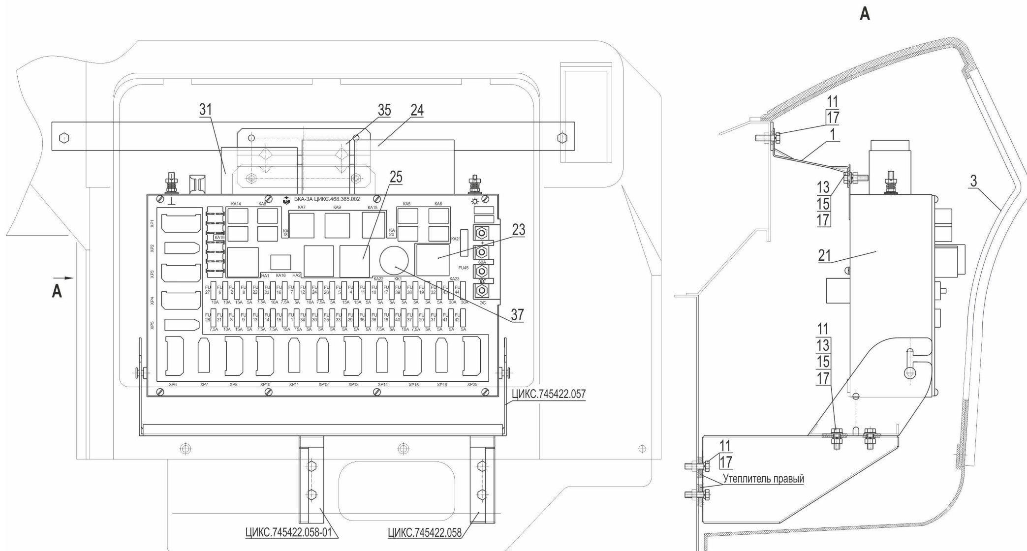
Рис. 207 Установка БКА-N3 544019-3700110-001 Fig.207 Installation of switchgear unit 544019-3700110-001
