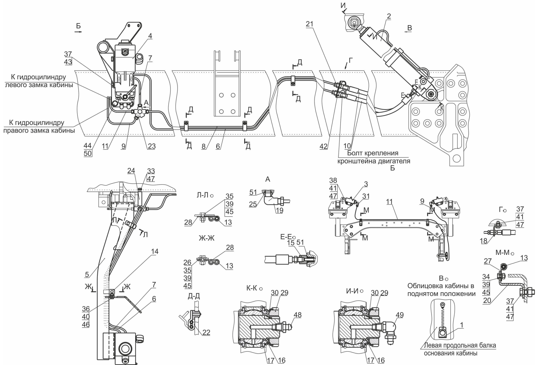
Fig. 267 Cab tilting mechanism 544019-5000040
