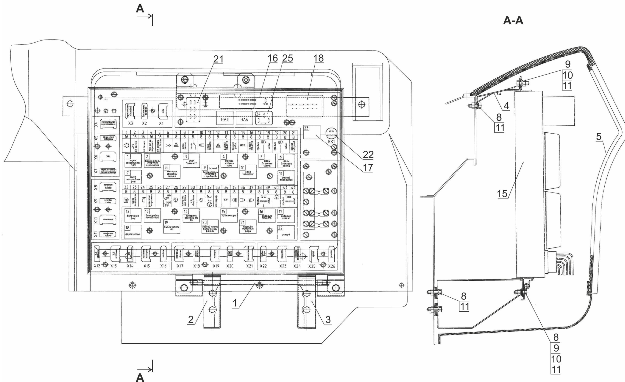
Рис. 206 Установка БКА-N3 544019-3700110 Fig.206 Installation of switchgear unit 544019-3700110
