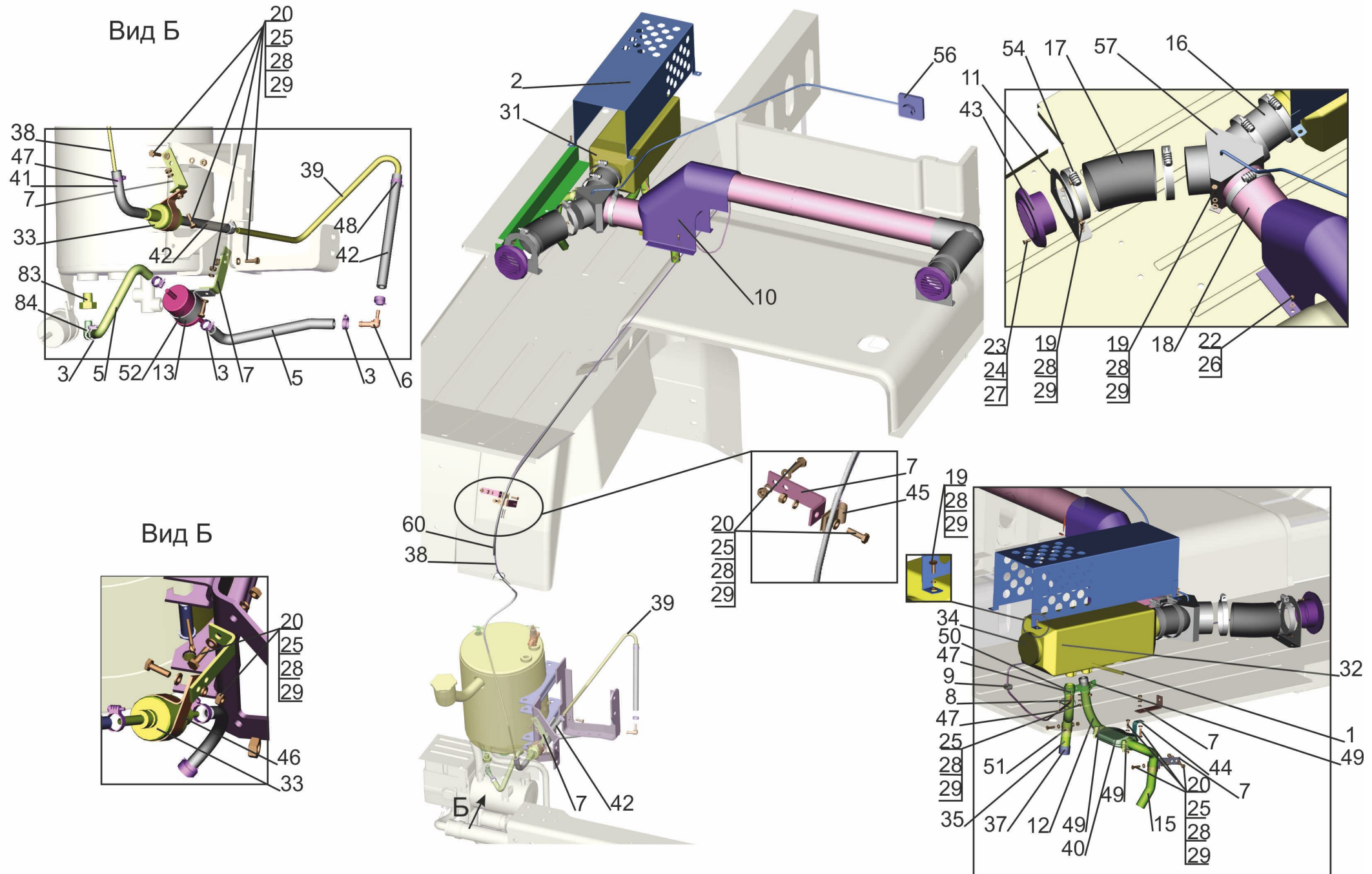
Fig. 291 Installation of the independent air heater 6430-8100002
