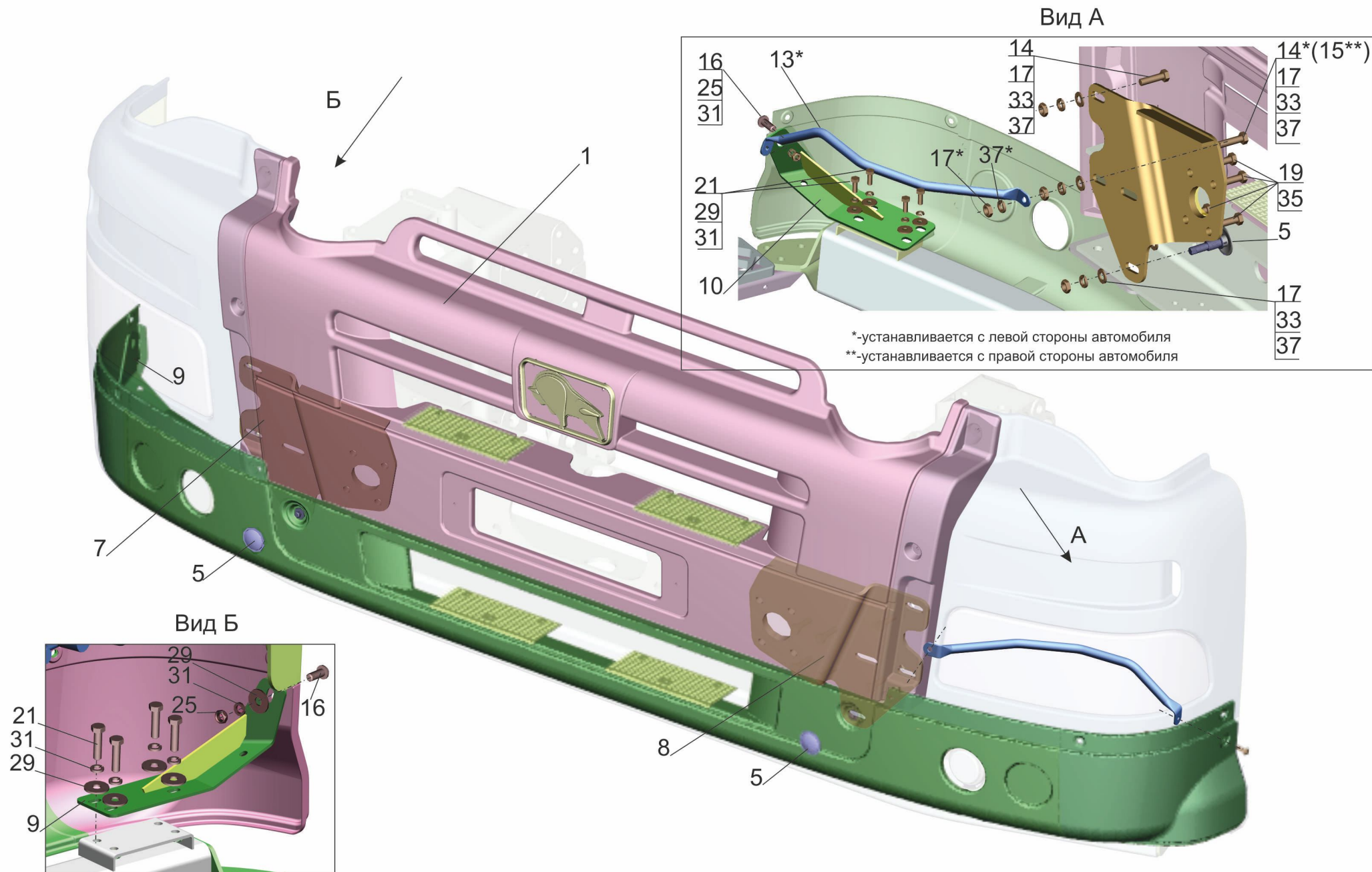
Fig. 97 Installation front bumper
