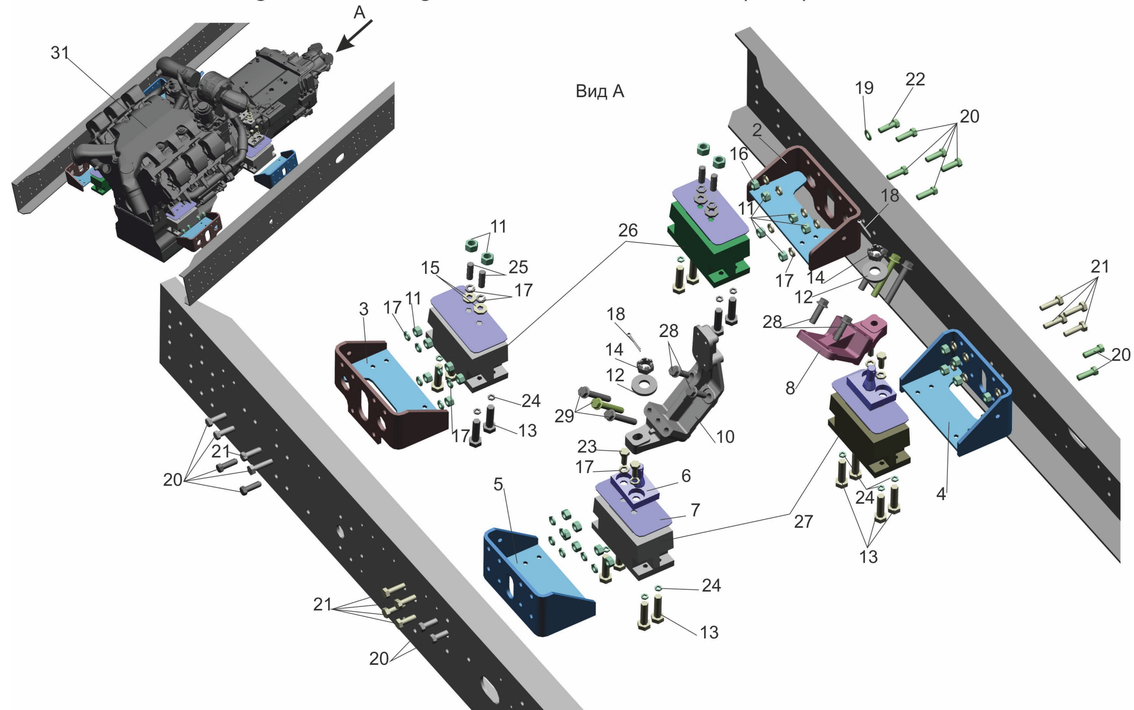
Fig. 2 Mounting diesel 544018-1001002, (-010)
