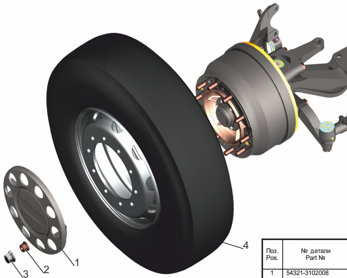
Fig. 139 Installation of front wheels
