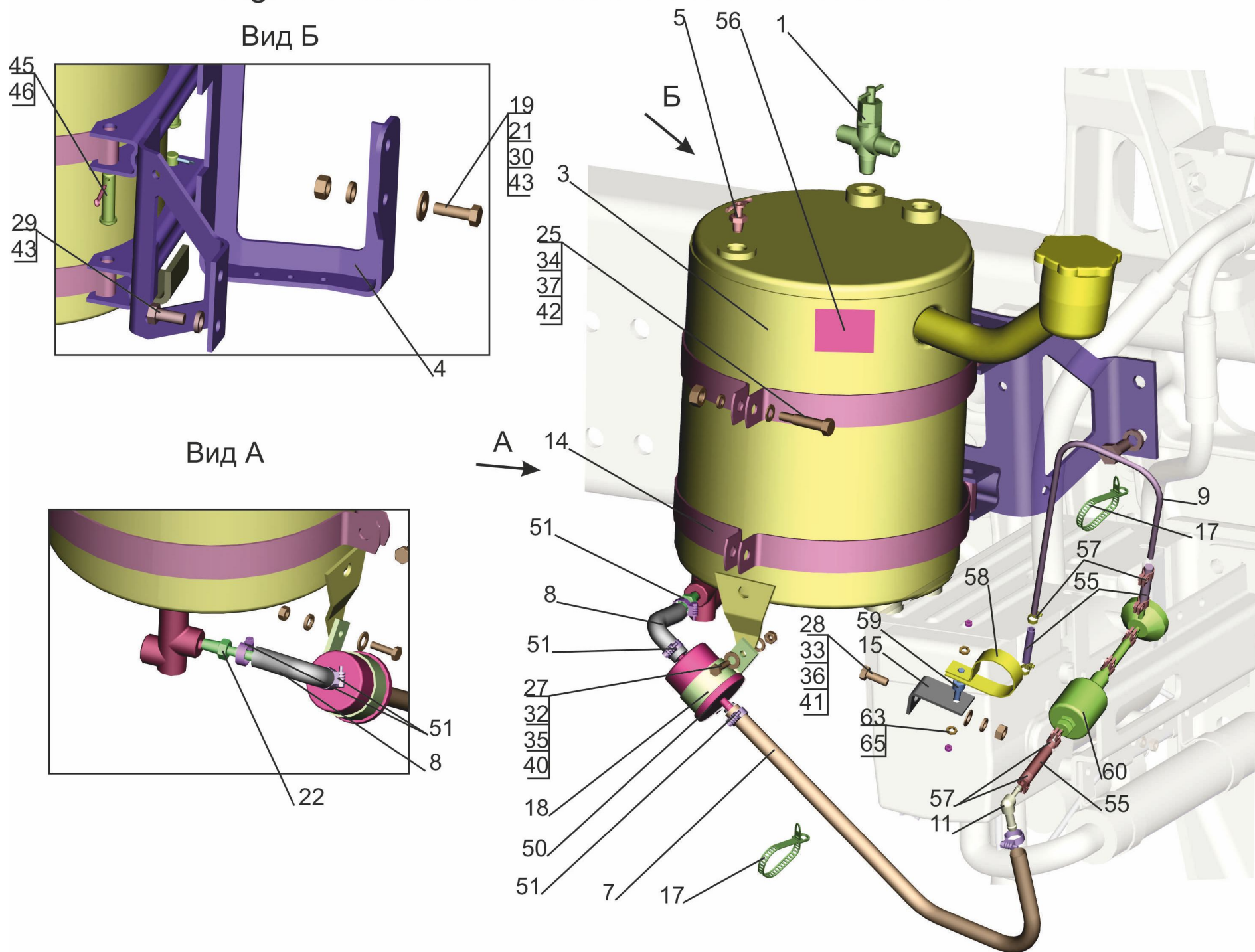
Fig. 8 Fuel lines of heater 544019-1015004-010
