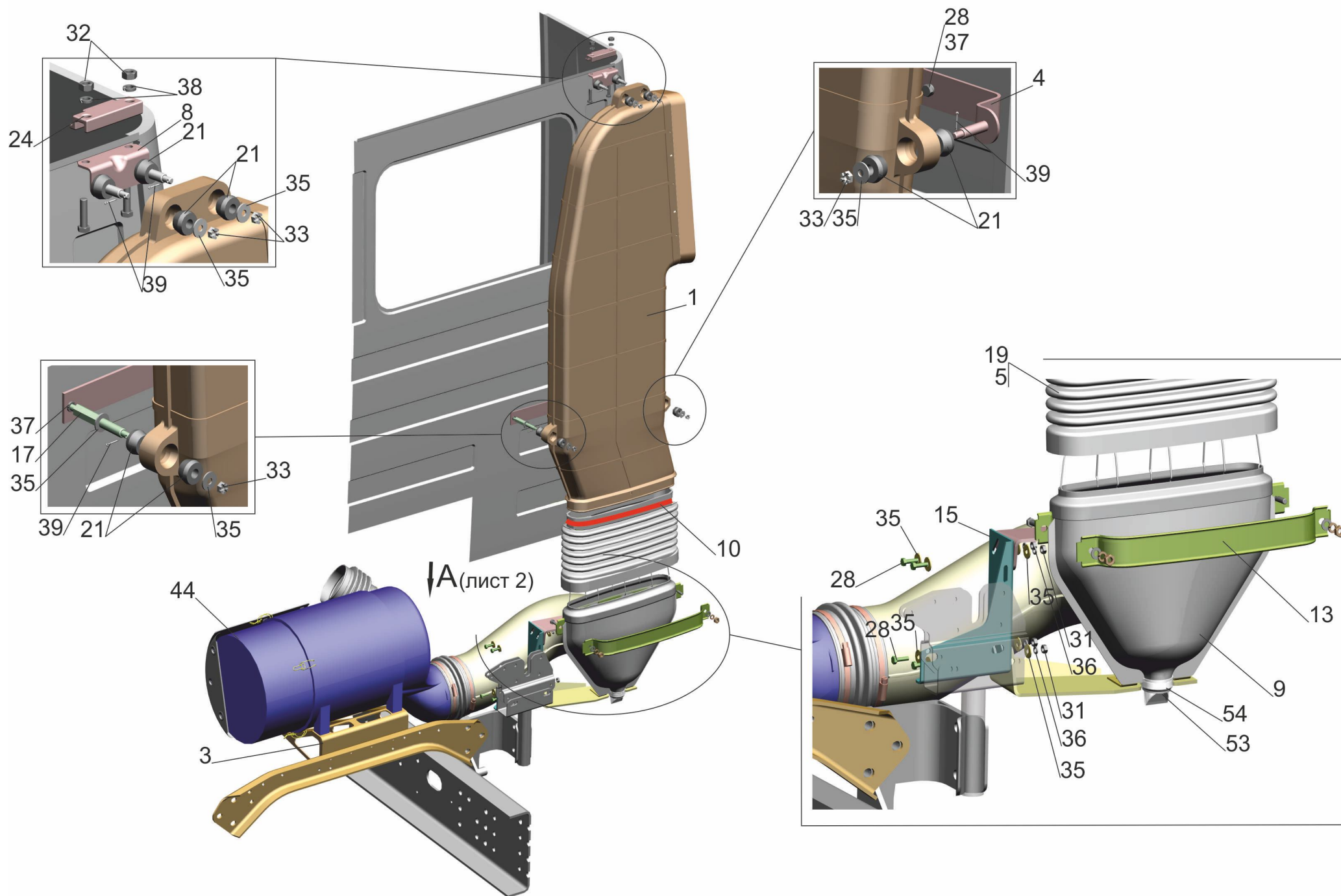
Fig. 23 Air filter mounting 544018-1109002 (page 1)
