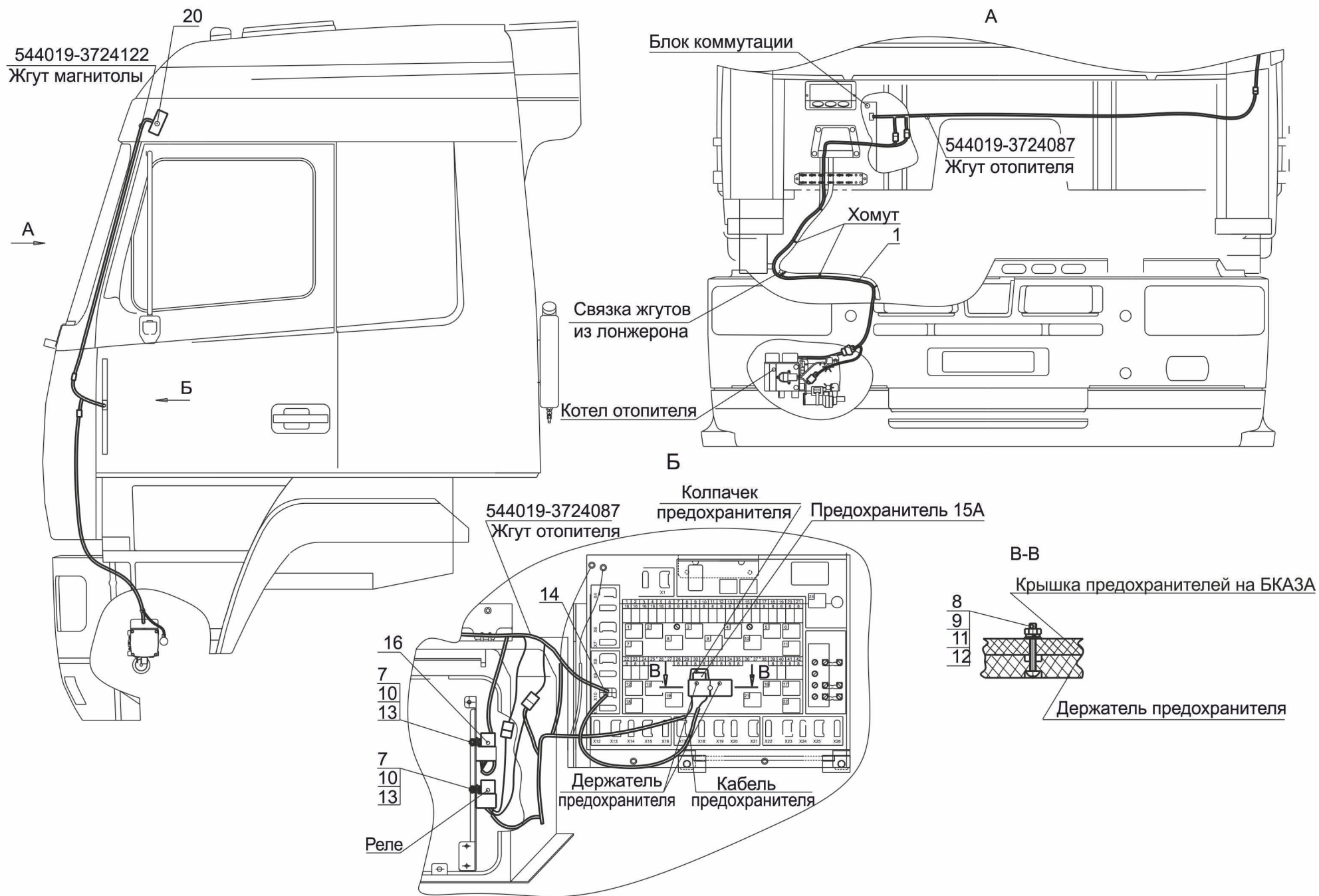
Fig. 10 Mounting of electrical equipment heater 544019-3700085
