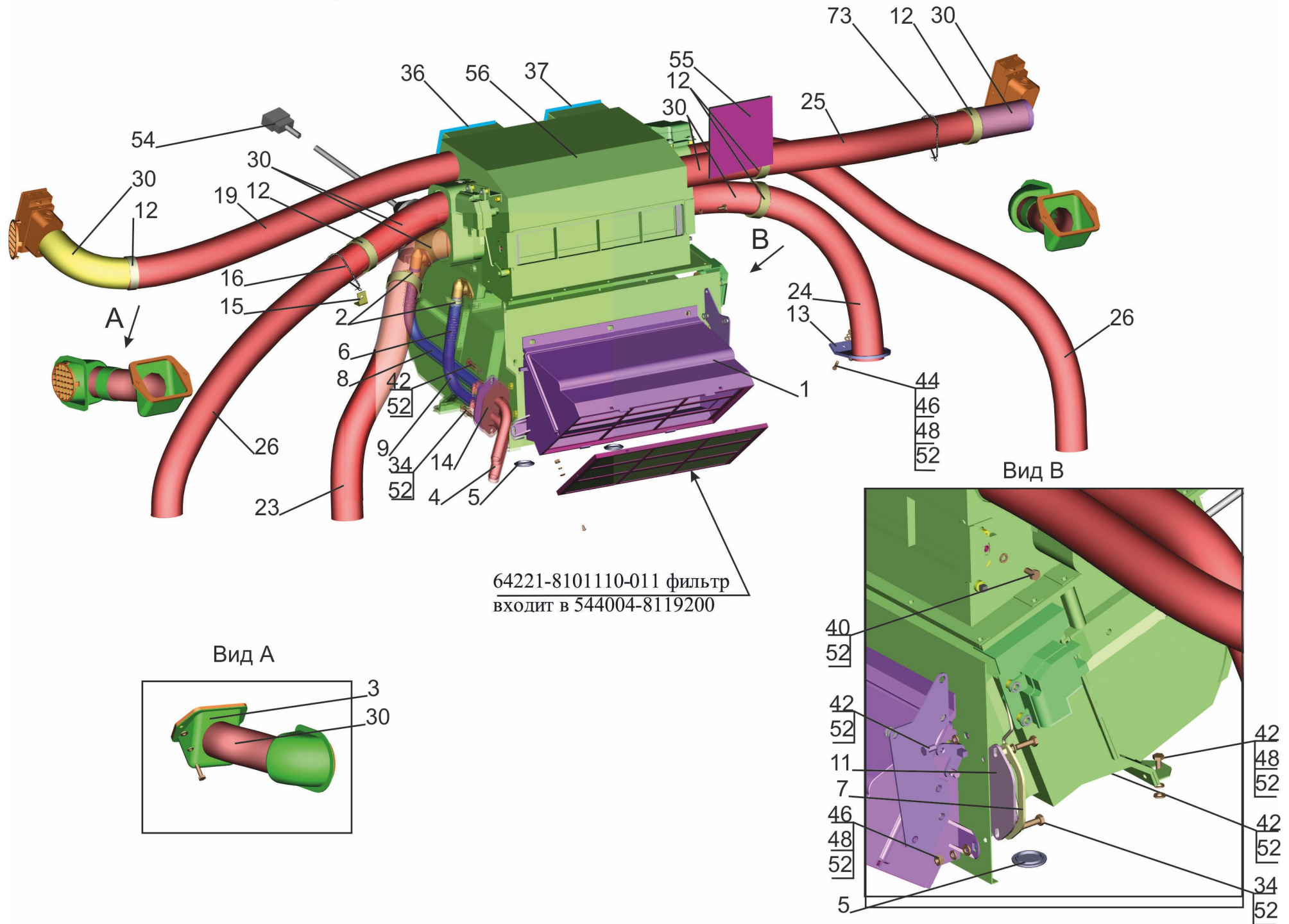
Fig. 275 Installation of heater 643008-8100001
