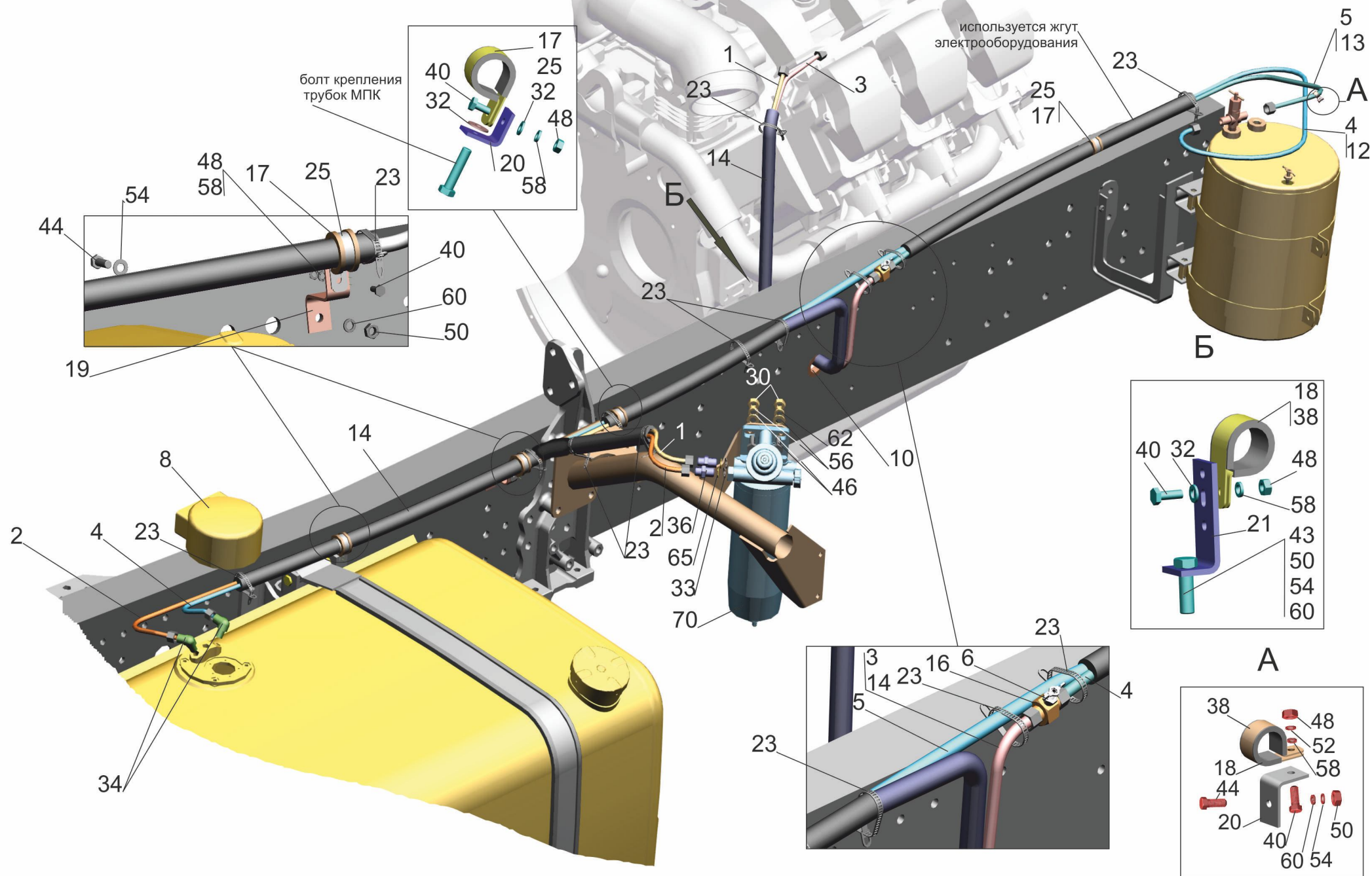
Fig. 20 Mounting of fuel lines 650119-1104002
