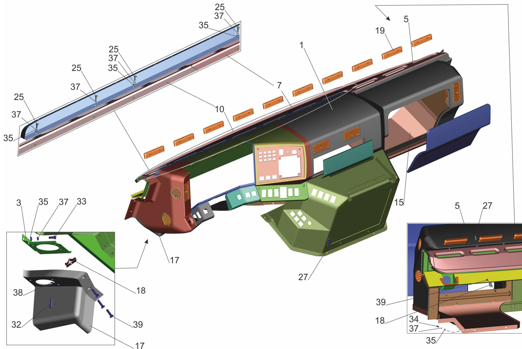
Fig. 237 Installing of instrument panel 6430-5300014-020.
