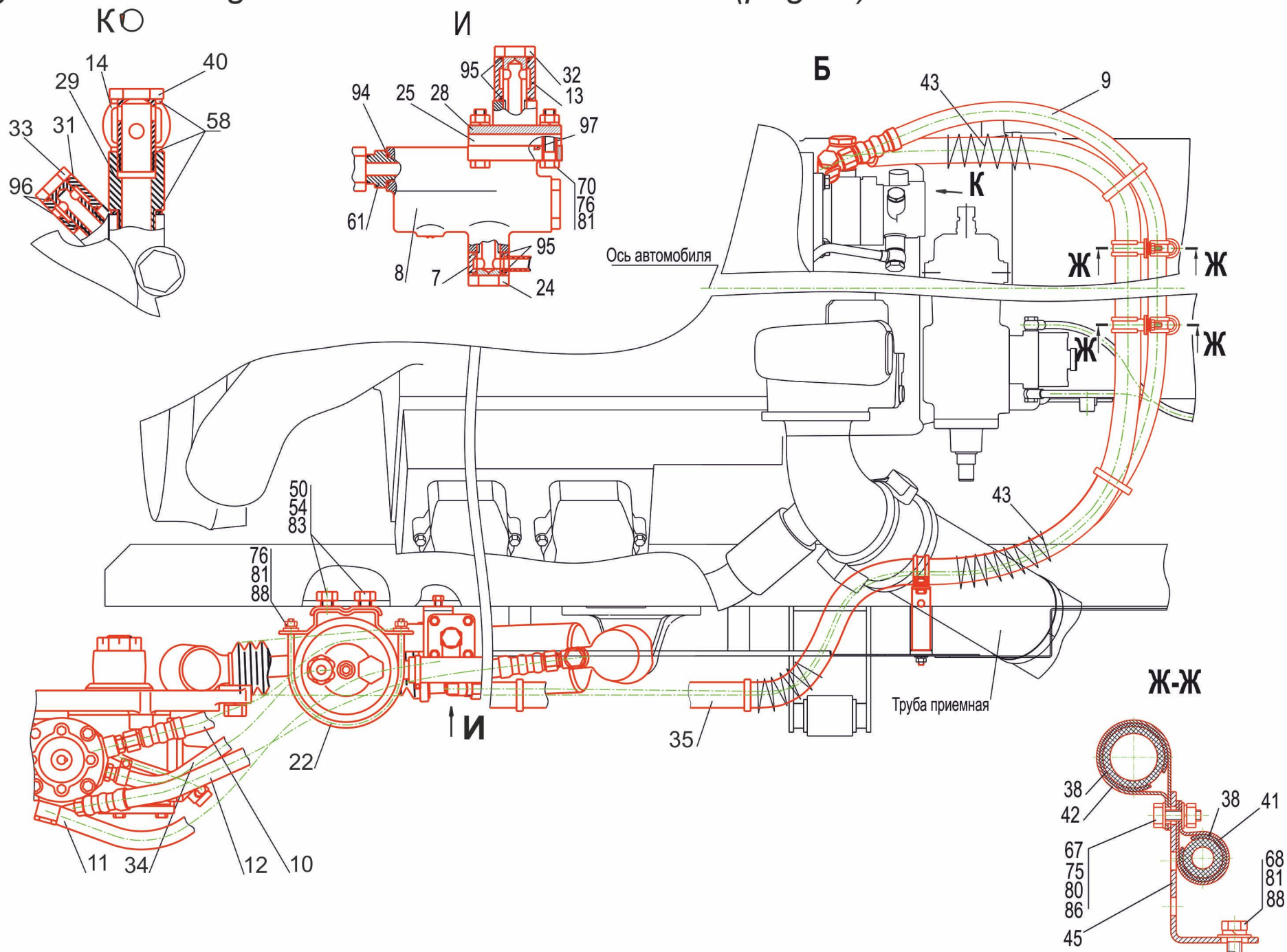
Fig. 142 Steering installation 6310E9-3400001 (page 2)
