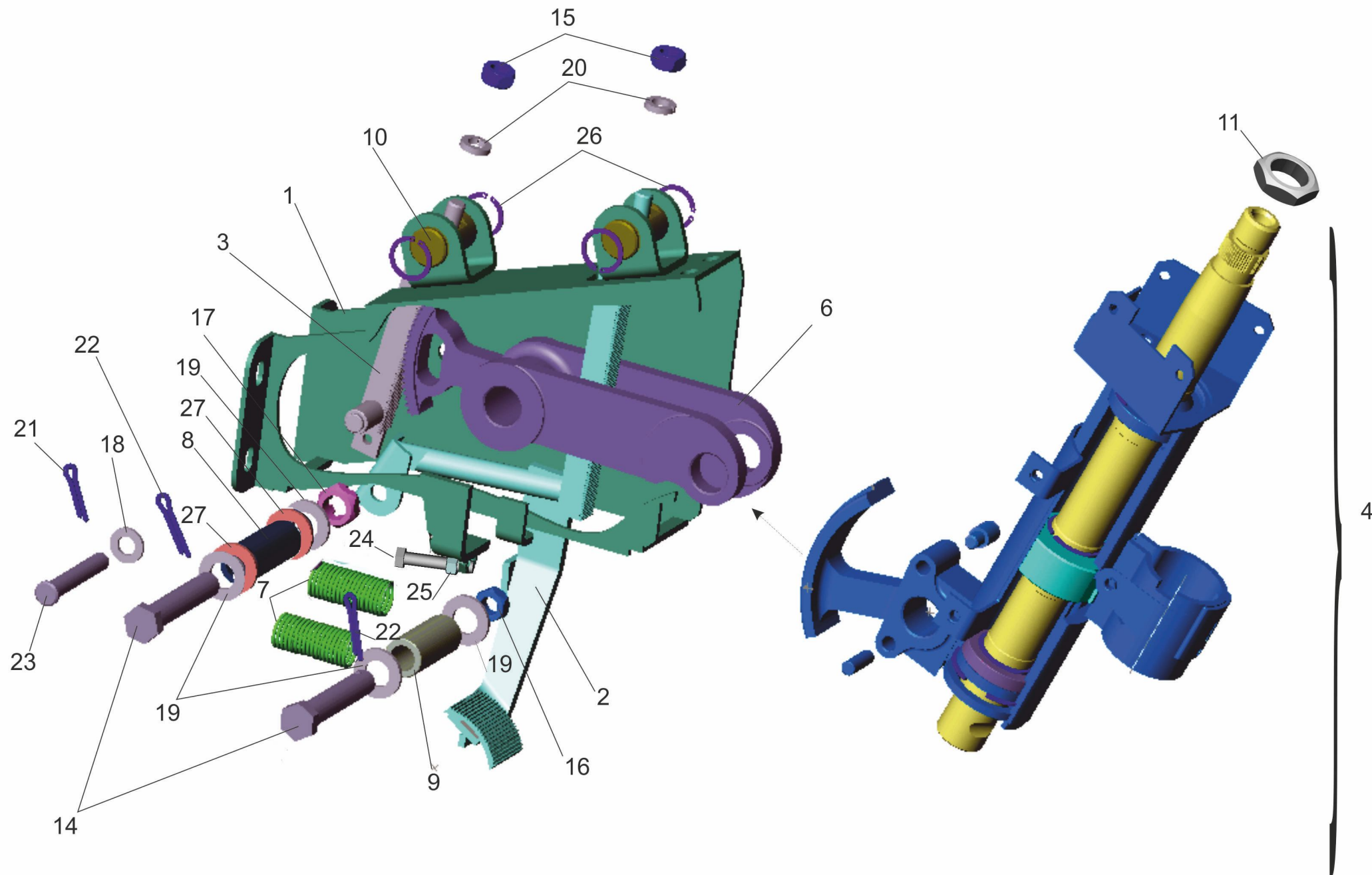
Fig. 153 Arm with a column 5440-3403008
