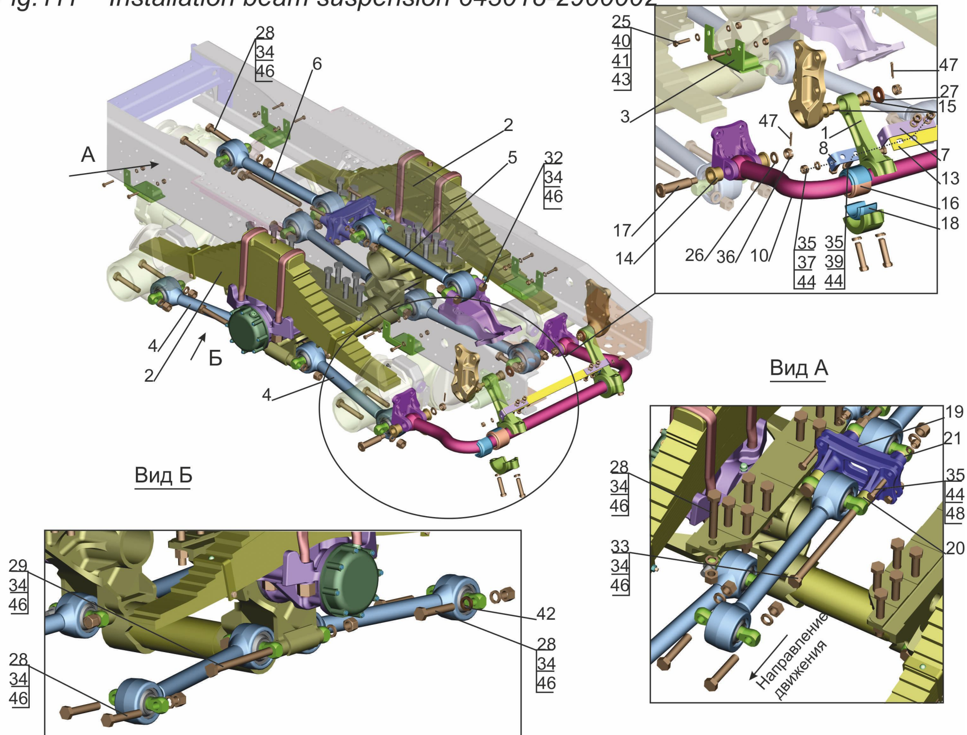
Fig.111 Installation beam suspension 643018-2900002
