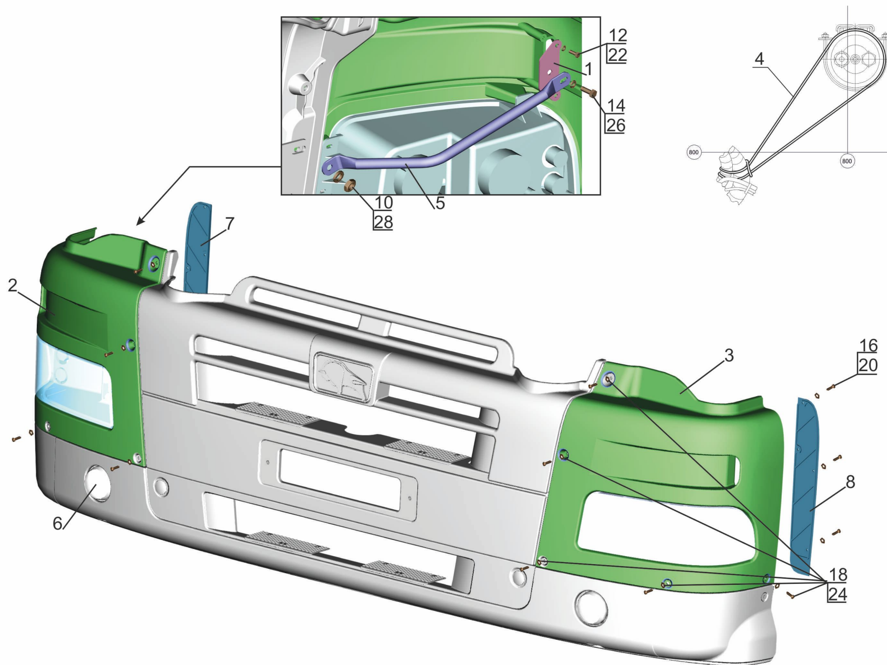
Fig. 99 Installation front bumper 643019-2800005
