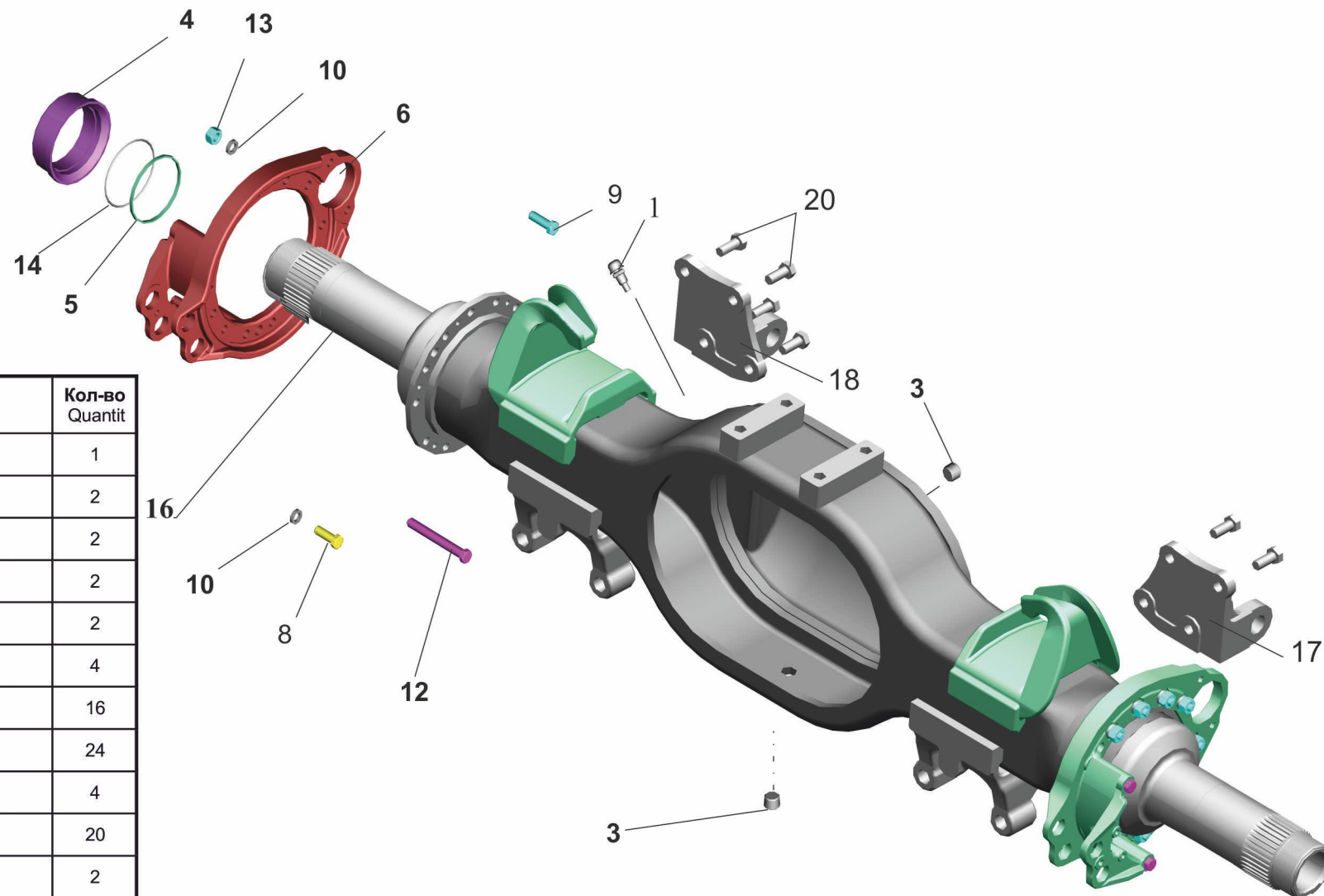
Fig. 66 Rear axle. Axle housing 6501-2401010-030
