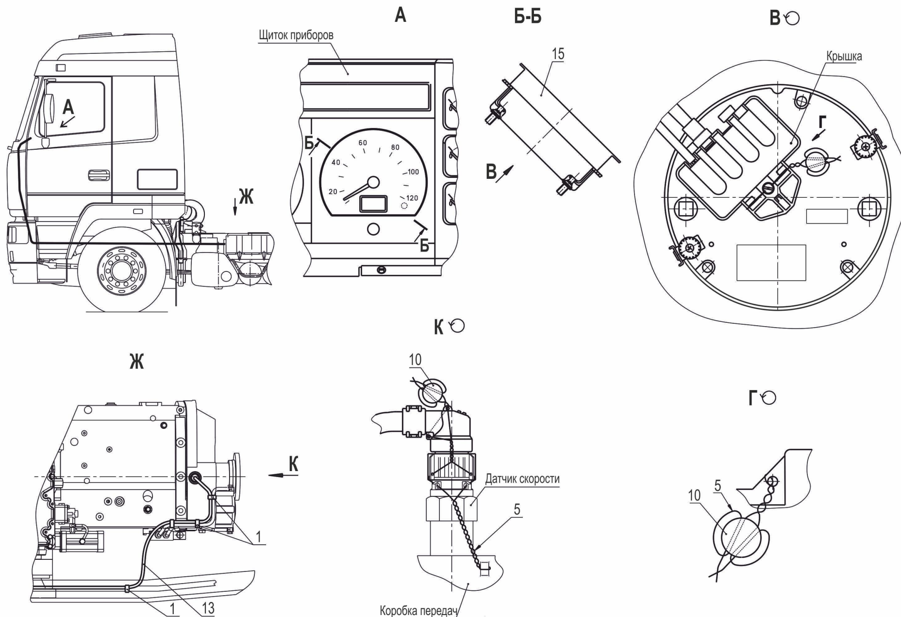
Fig.208 Installation and identification seal of a speedometer 5440-3800004-040
