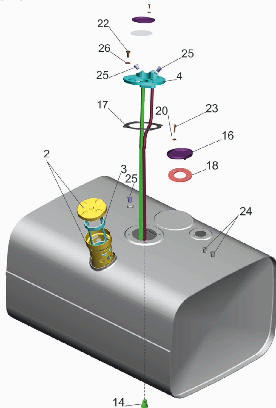
Fig. 14 Tank fuel 437137-1101010
