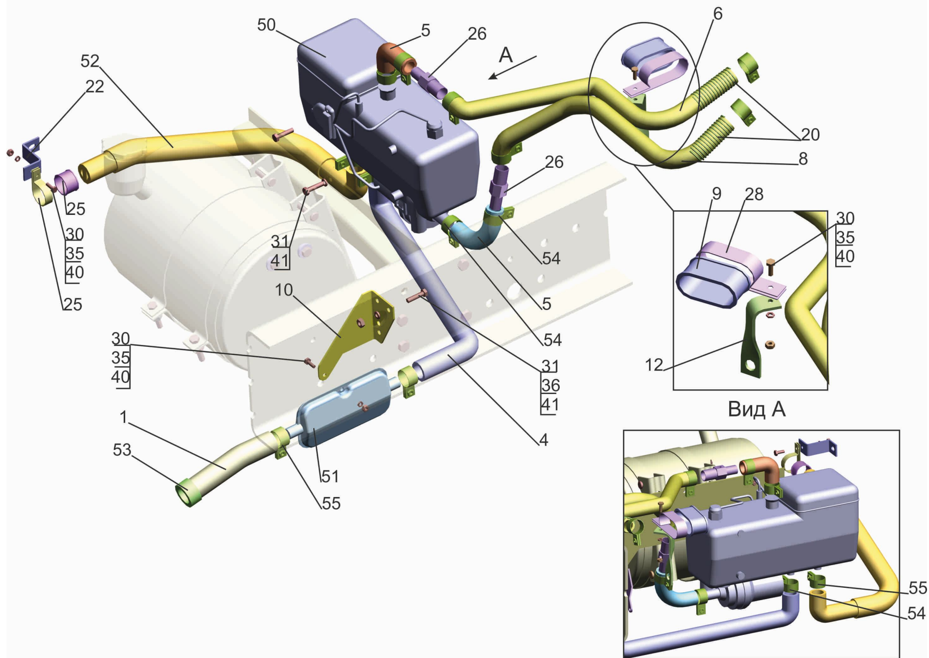
Fig.5 Heater mounting 437041-1015001-001, (-021)
