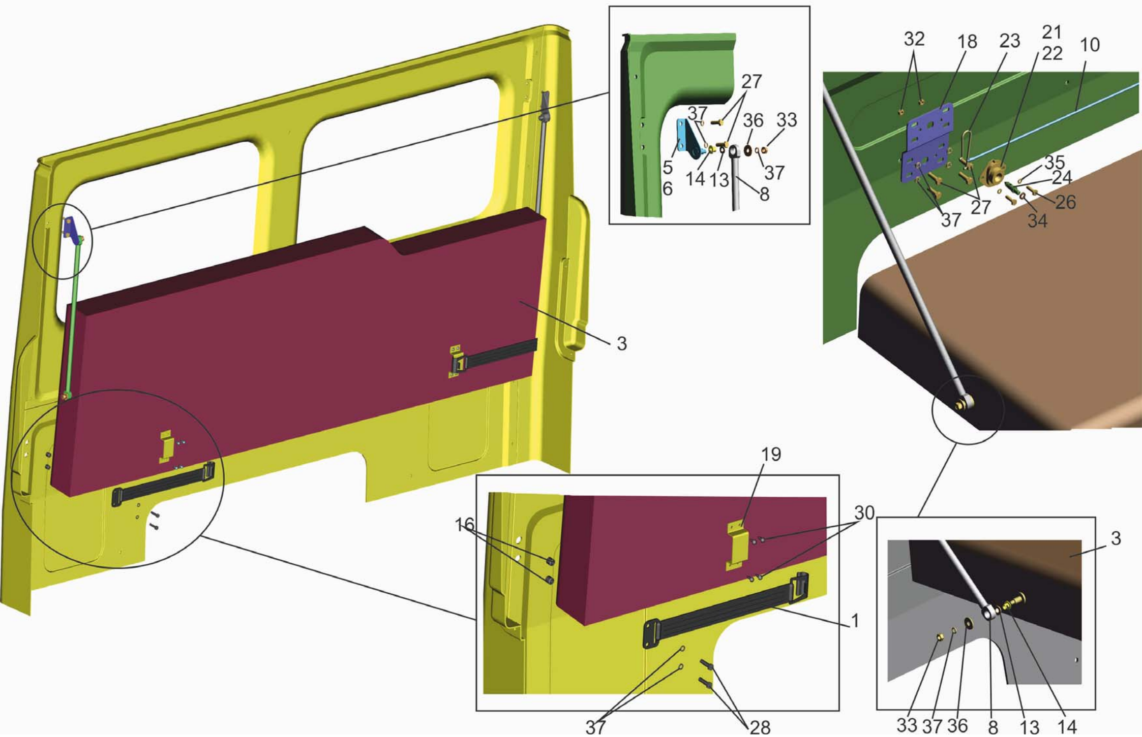
Fig. 238 Installation of a berth 4371-8200010
