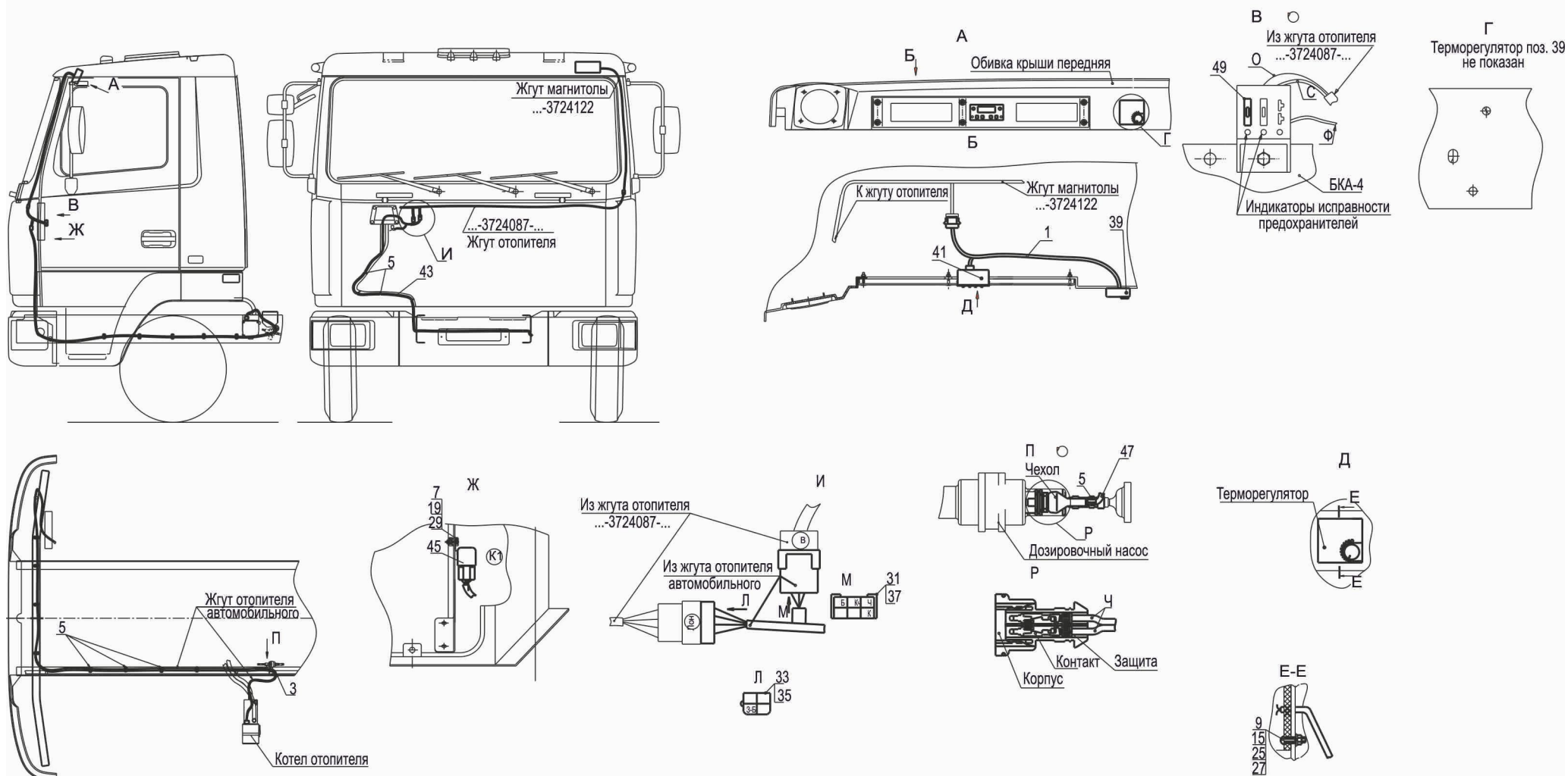
Fig. 156 Mounting of electrical equipment heater 4371W1-3700085-010
