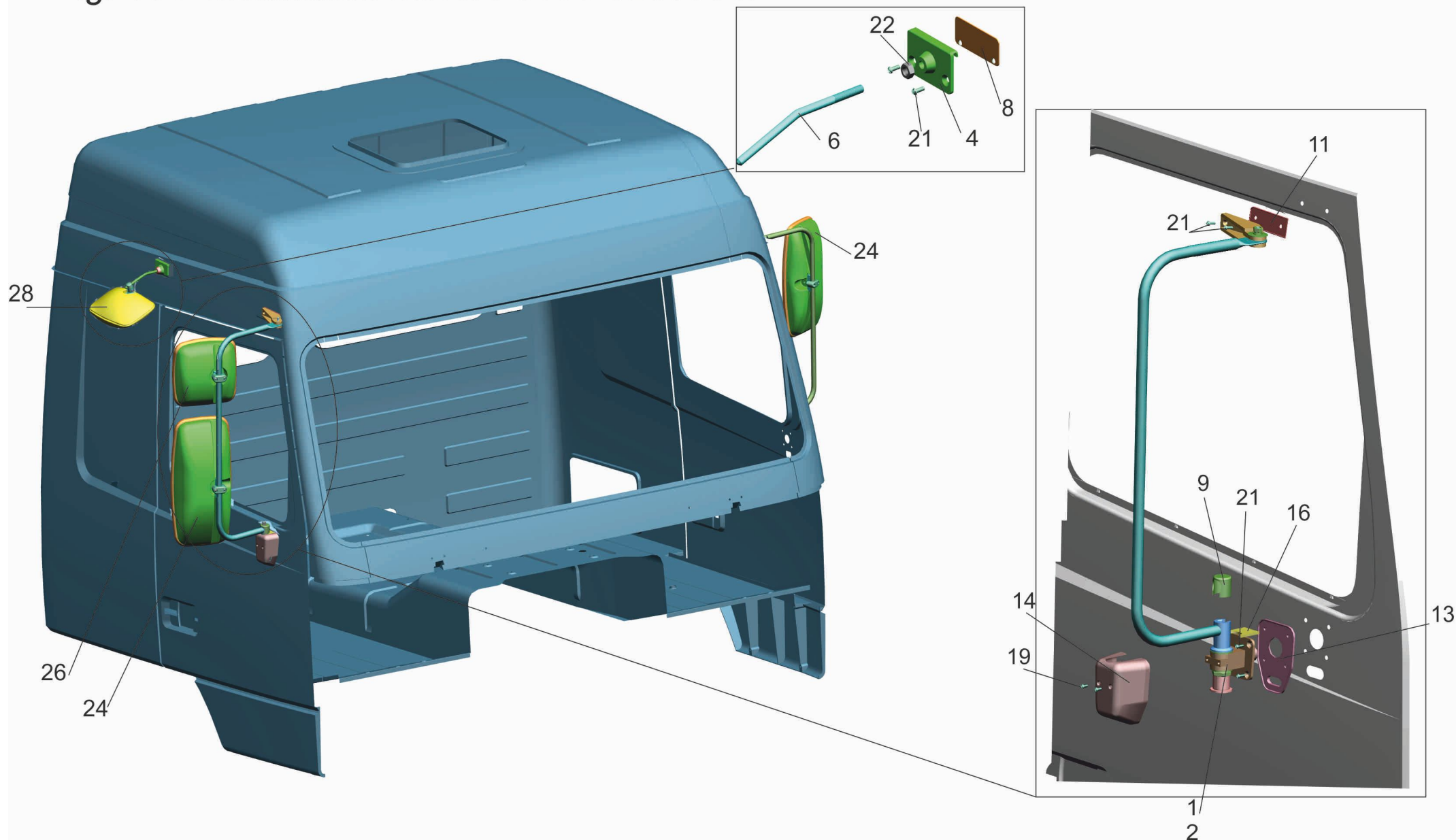
Fig. 194 Installation mirrors 6430-8200005.
