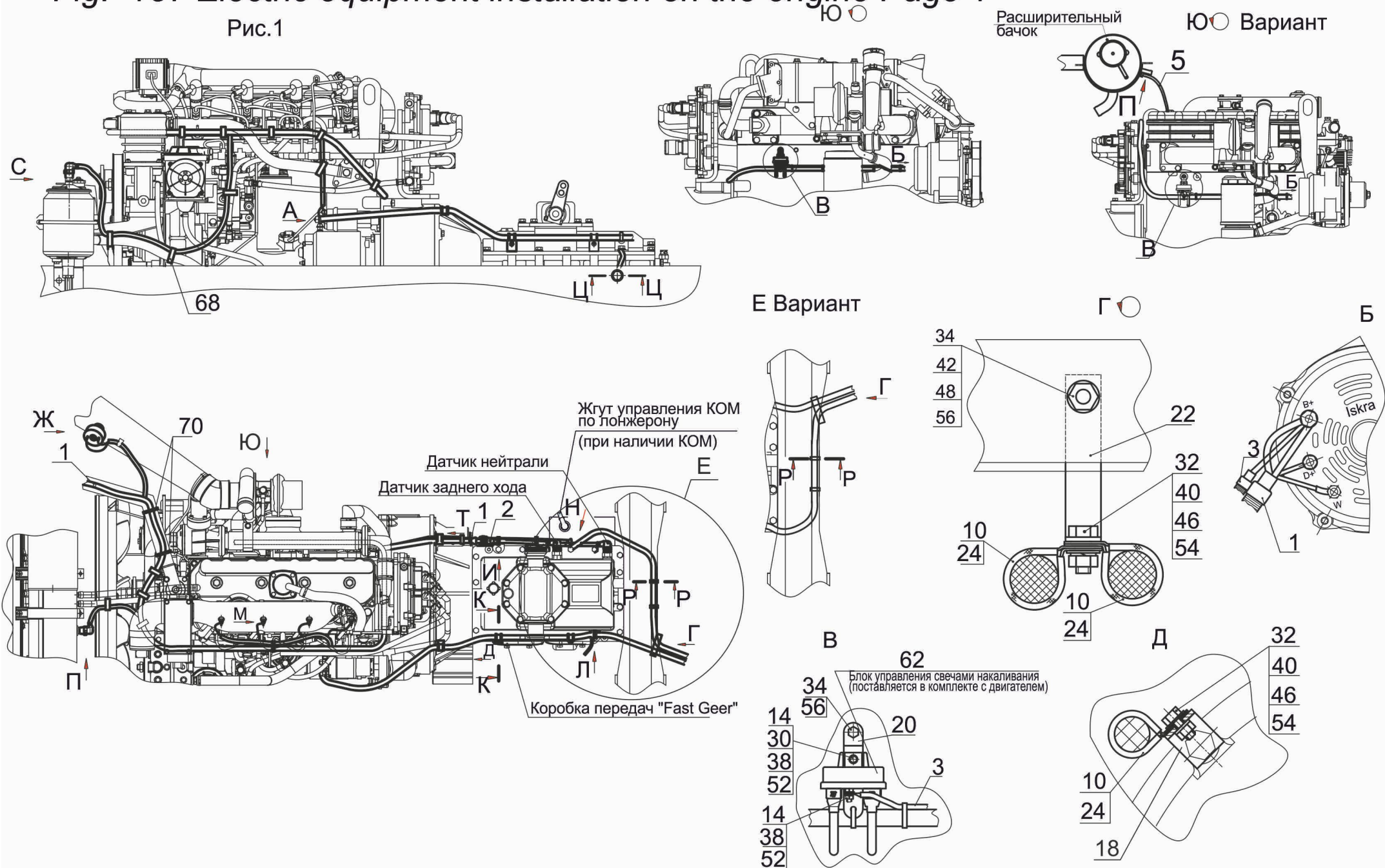
Fig. 157 Electric equipment installation on the engine Page 1
