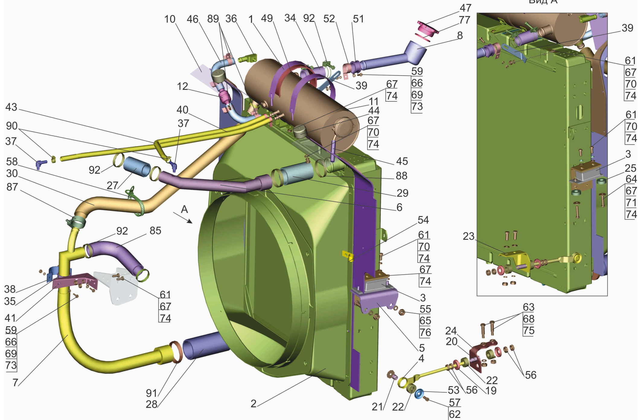
Fig. 25 Installation of cooling system 4371P2-1300005-000
