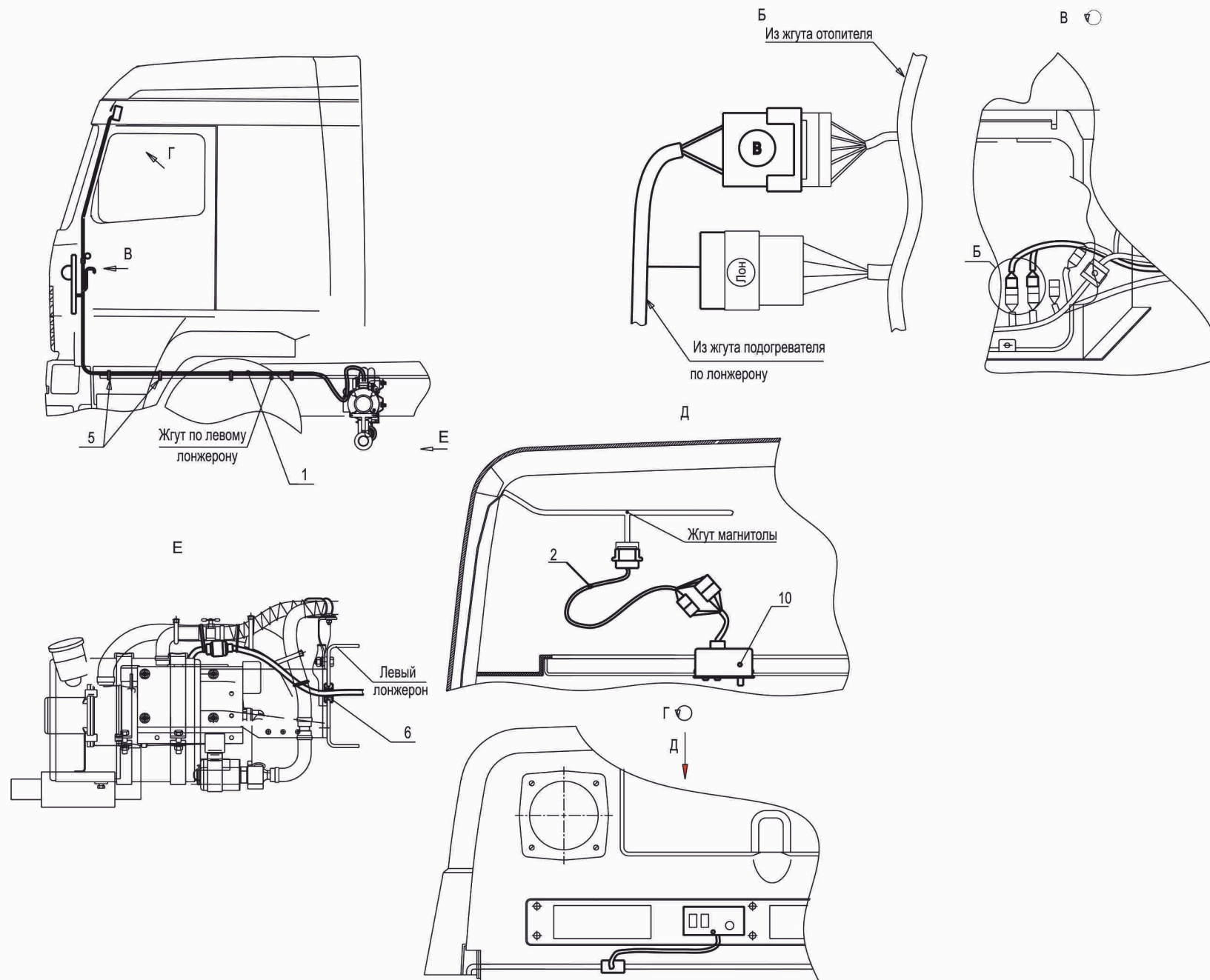
Fig. 155 Mounting of electrical equipment heater 437143-3700085-009
