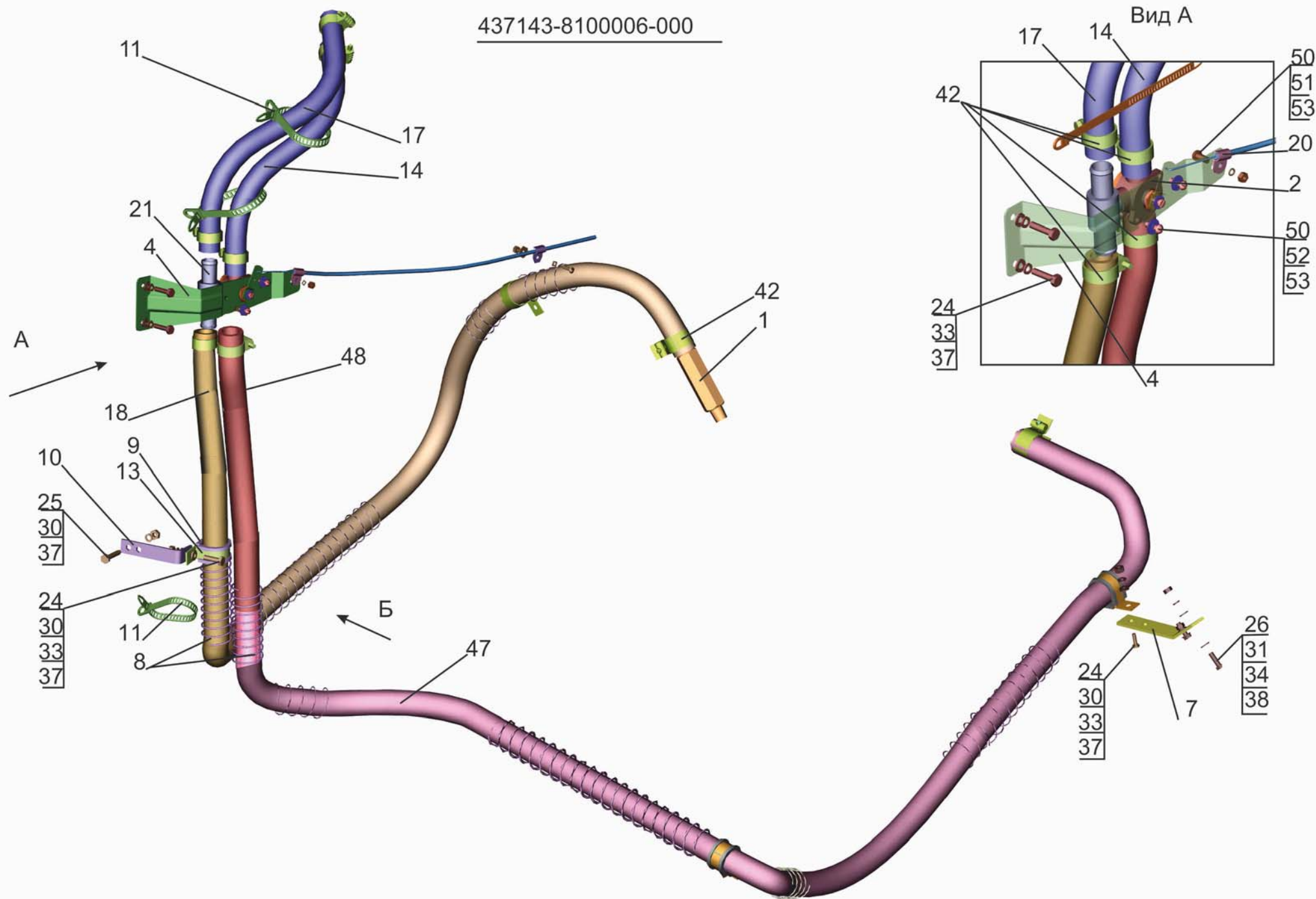
Fig. 236 Installation of heater hoses 437143-8100006-000,(-010) (page 1)
