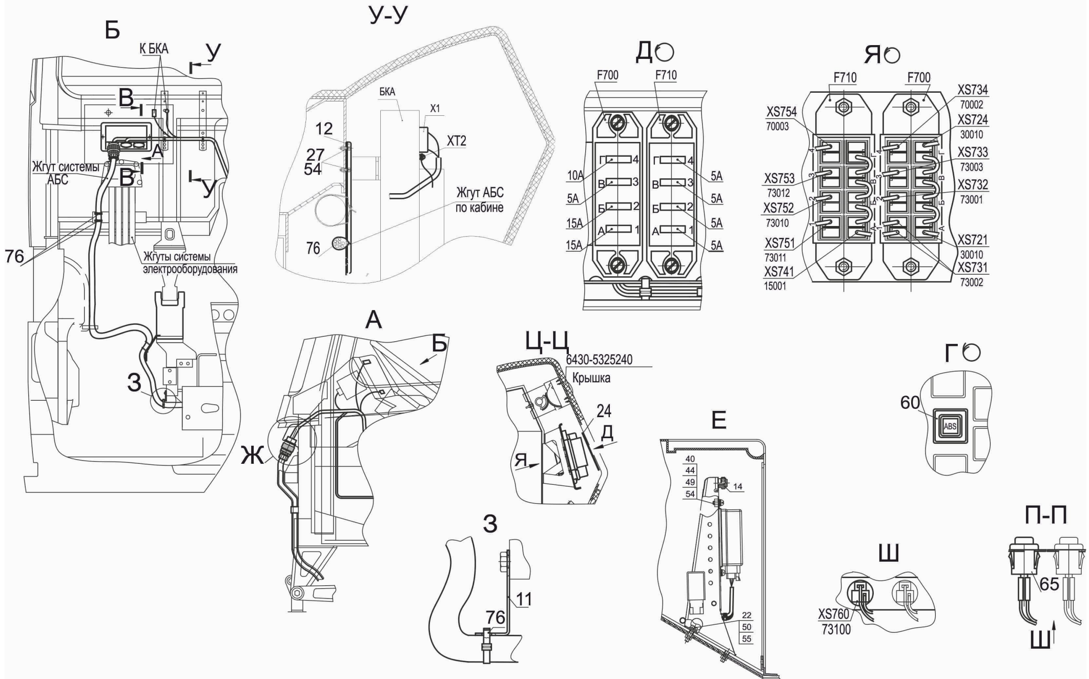
Fig. 174 Setting electrical equipment ABS on a cabin Page 2
