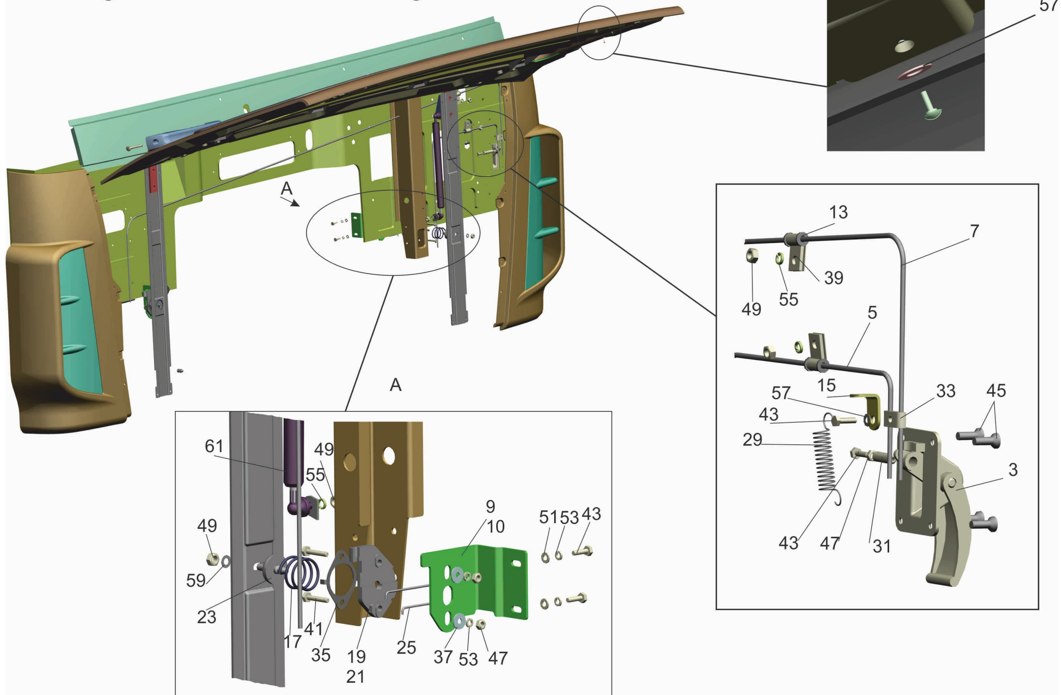
Fig.200 Installation of facing 6431-8400018-000
