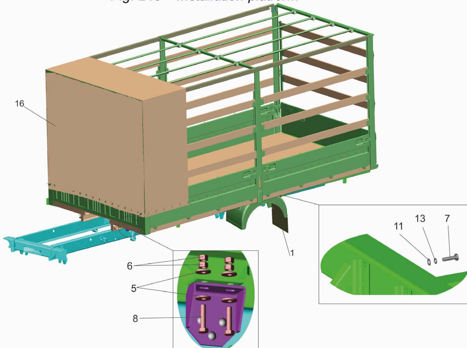
Fig. 243 Installation platform
