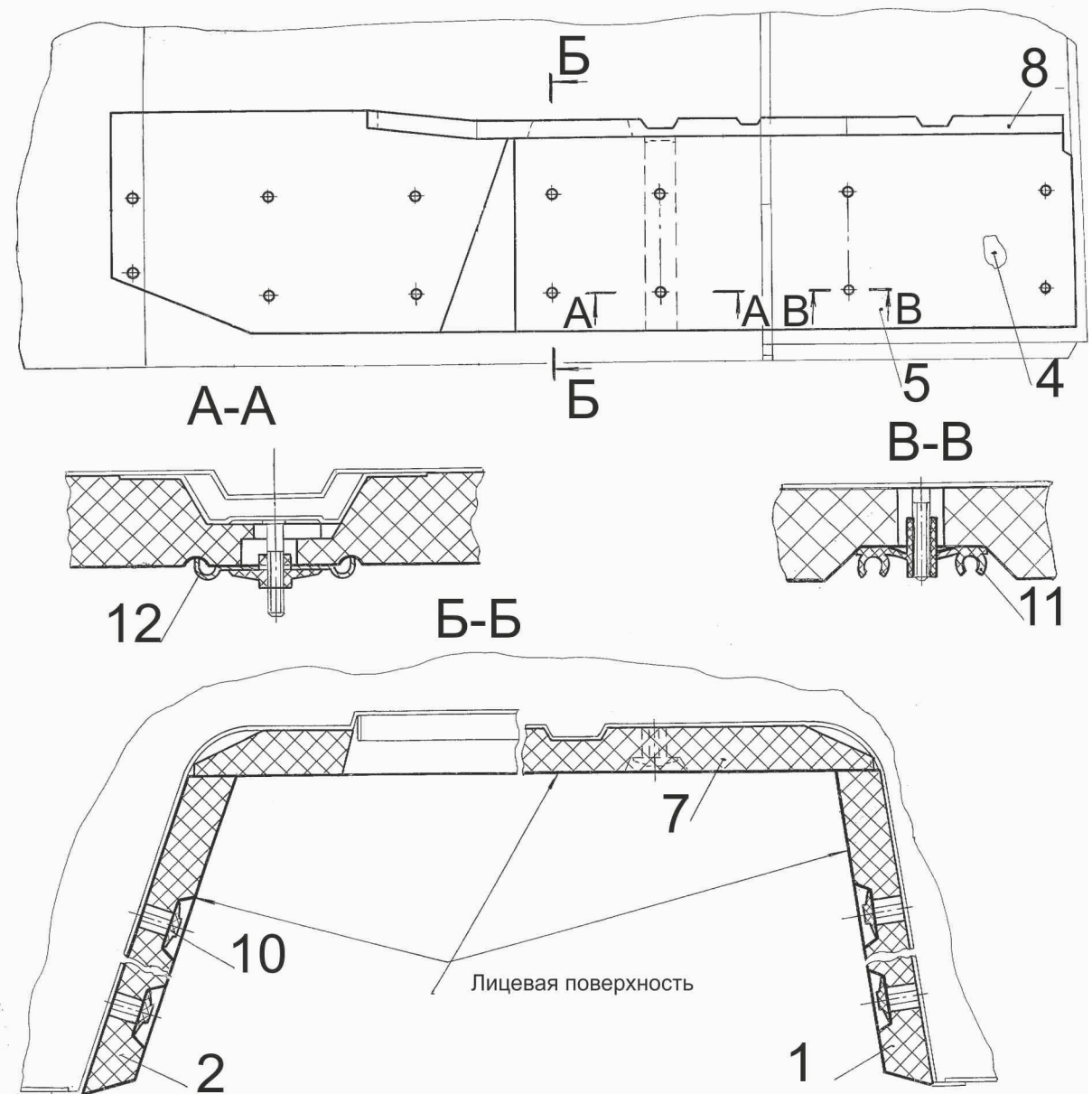
Fig. 203 Installation additional terhmo noise isolations 6418-5000122
