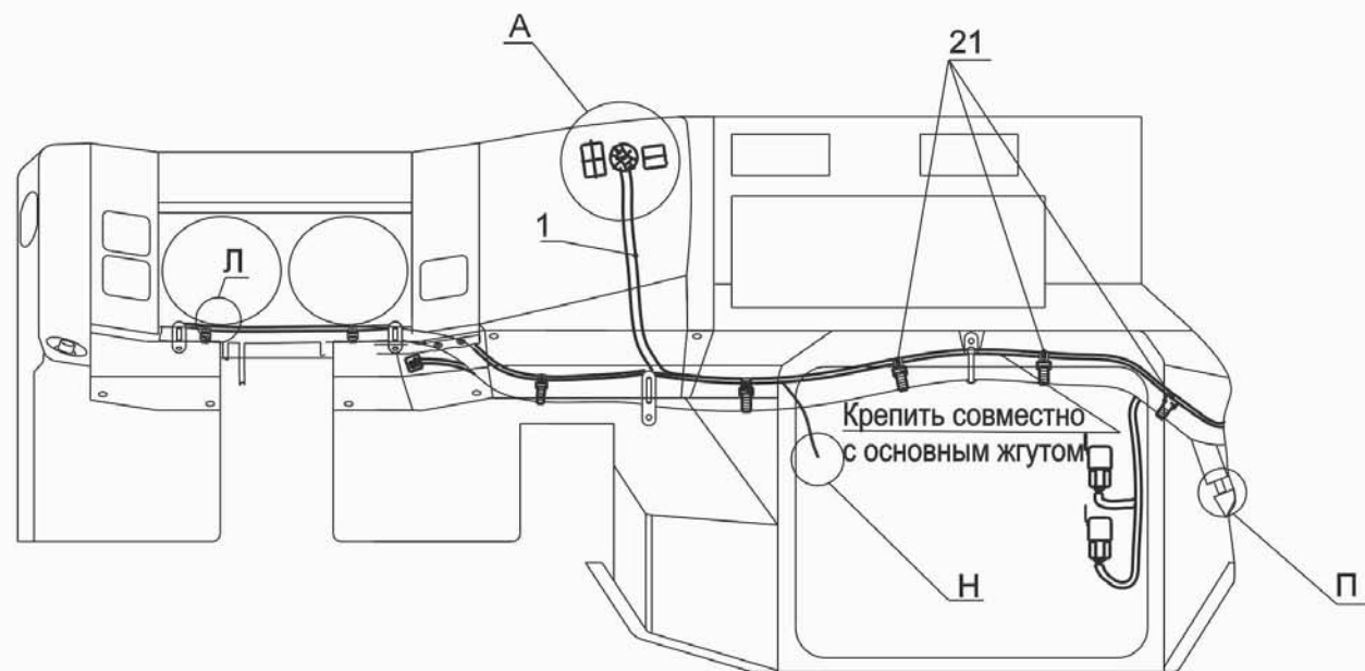
Fig. 234 Installation switch heater 6430-3700100-010
