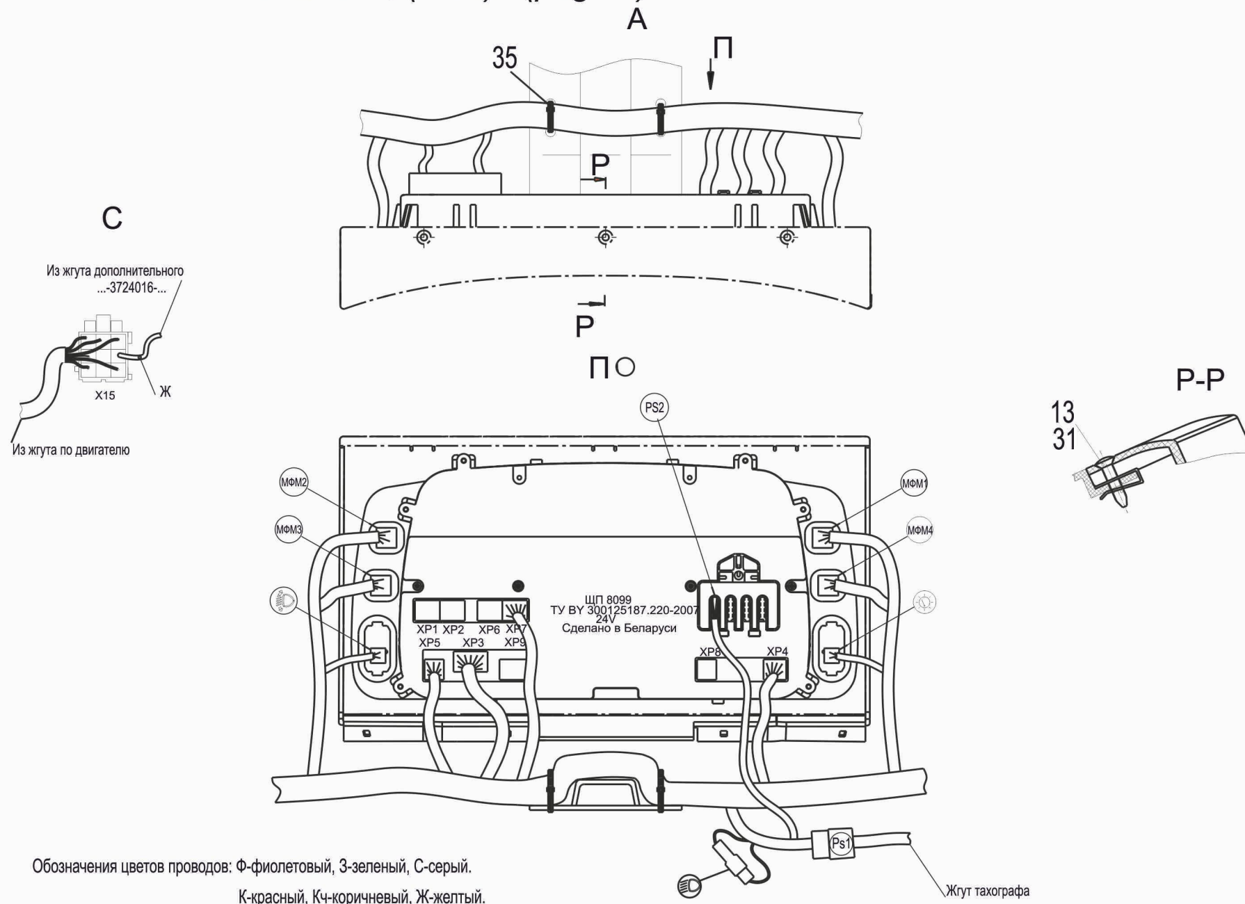
Fig.162 Installation boards devices and switching instrumentation 4371W1-3800001, (-700) (page 2)
