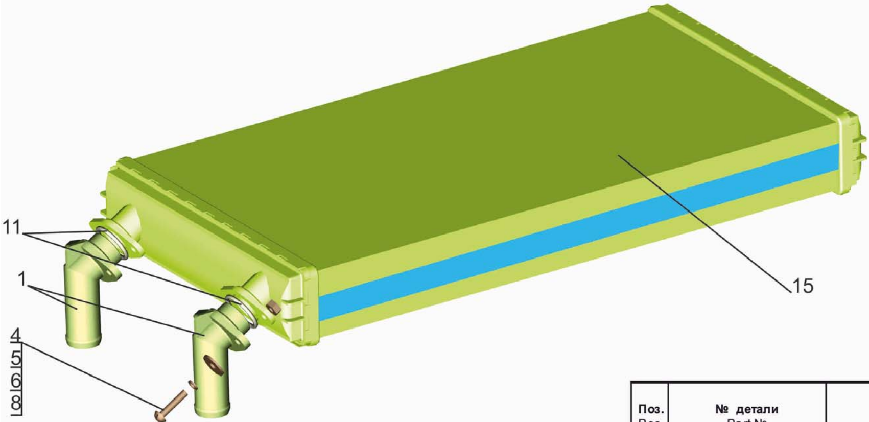
Fig. 232 Radiator of heating 631019-8101060
