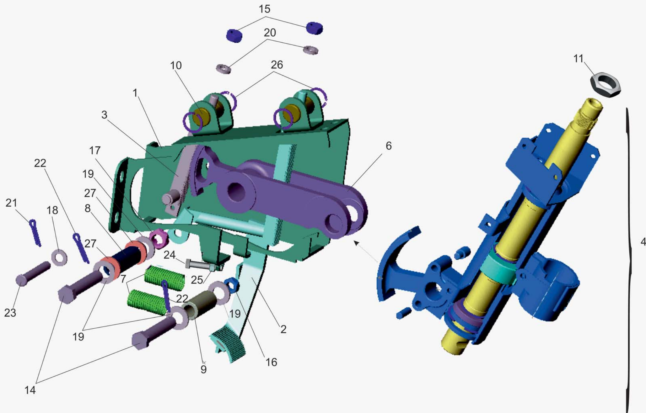
Fig. 118 Arm with a column 5440-3403008
