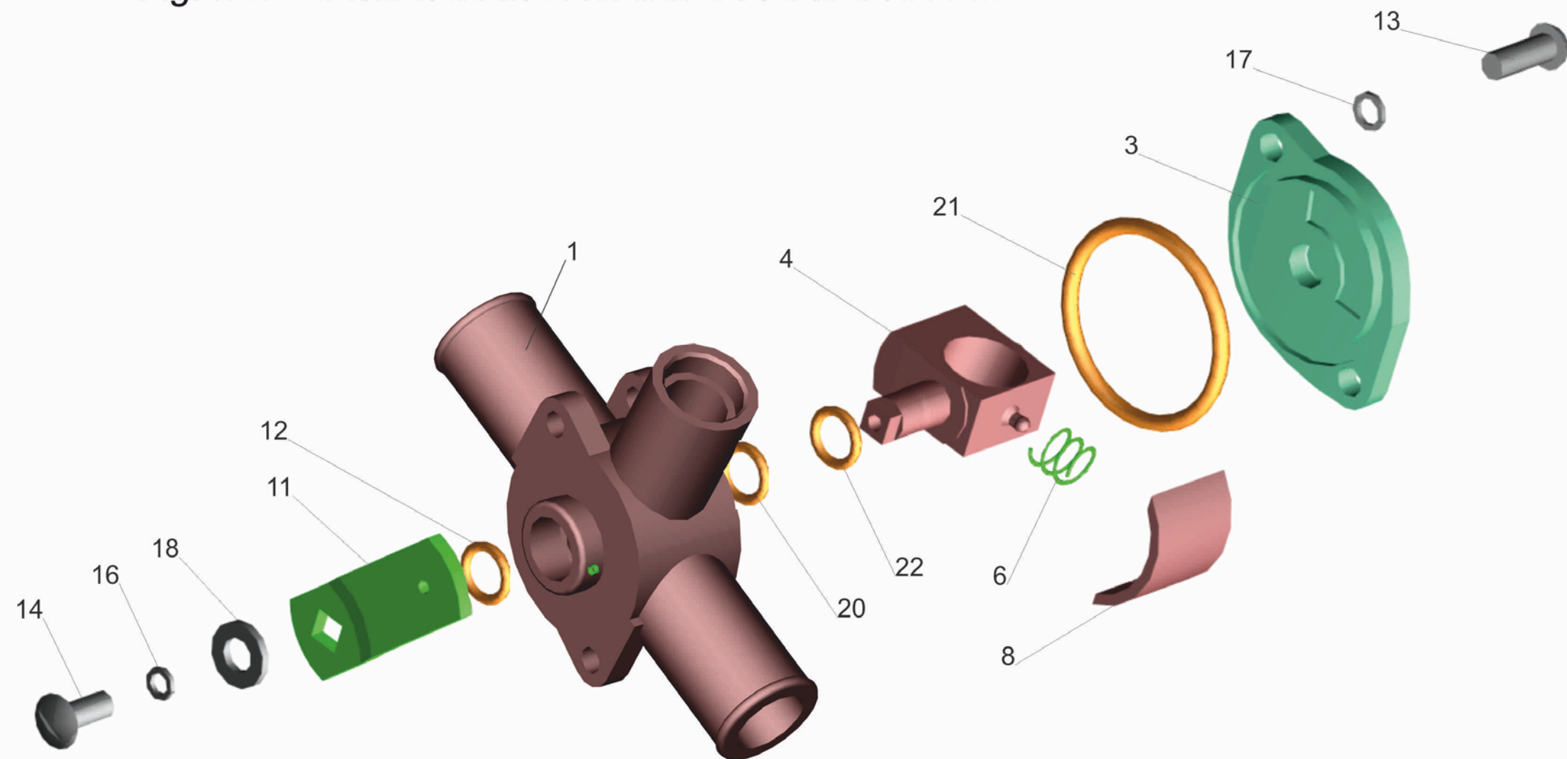
Fig. 237 Control cock of heater 5440A9-8101150
