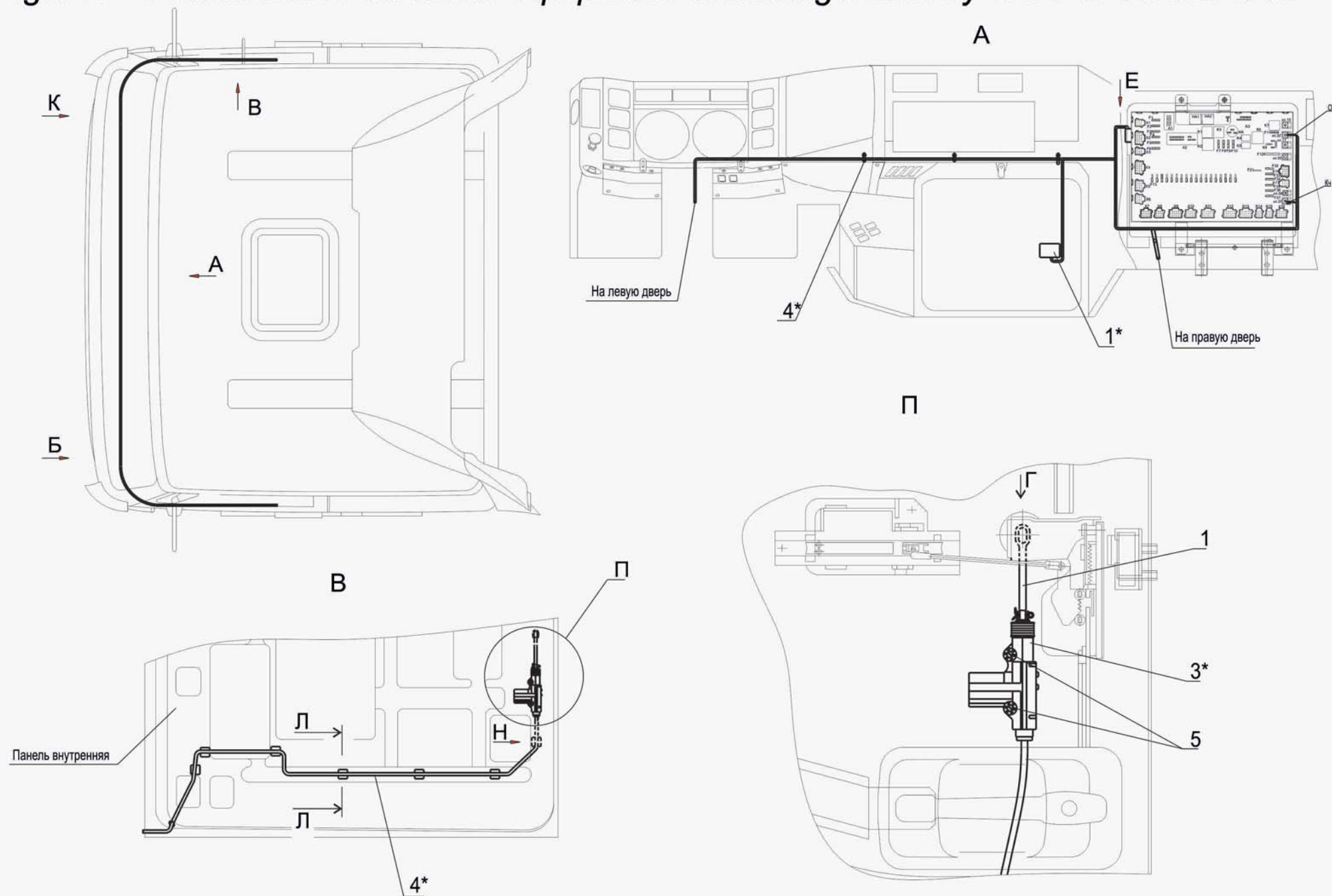
Fig.149 Installation of electrical equipment of management by drive of central lock
