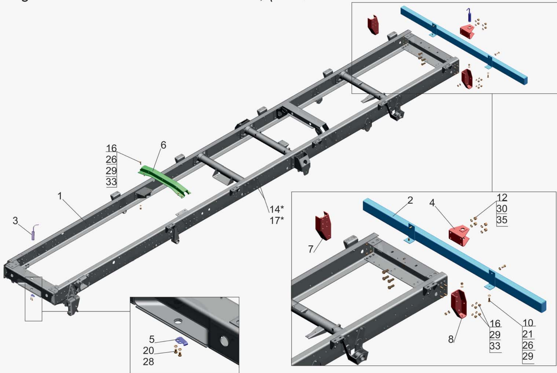
Fig.75 Frame 4371P2-2800010-003, (-013)
