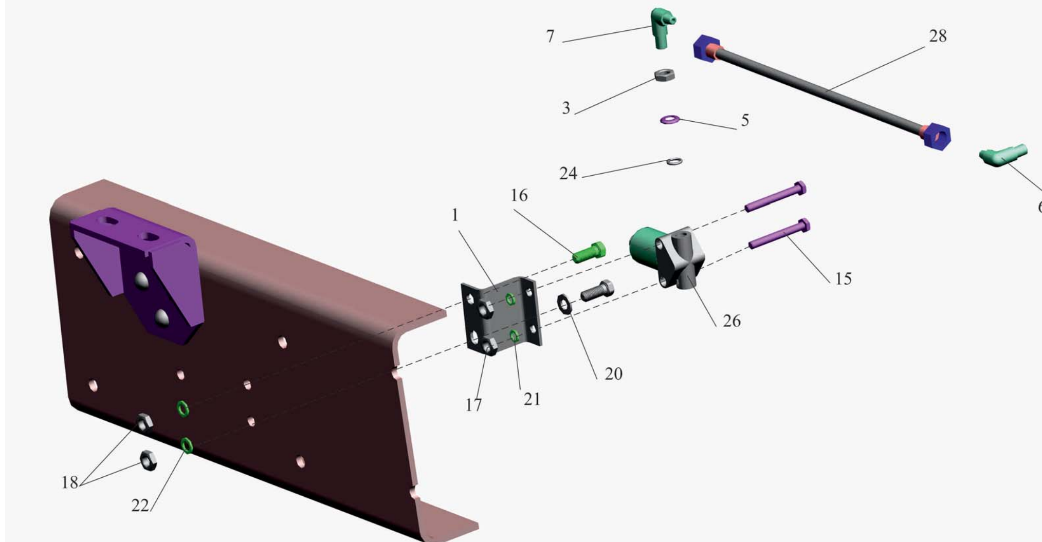
Fig. 73 Mounting of differential lock control linkage 4370-2400024-010
