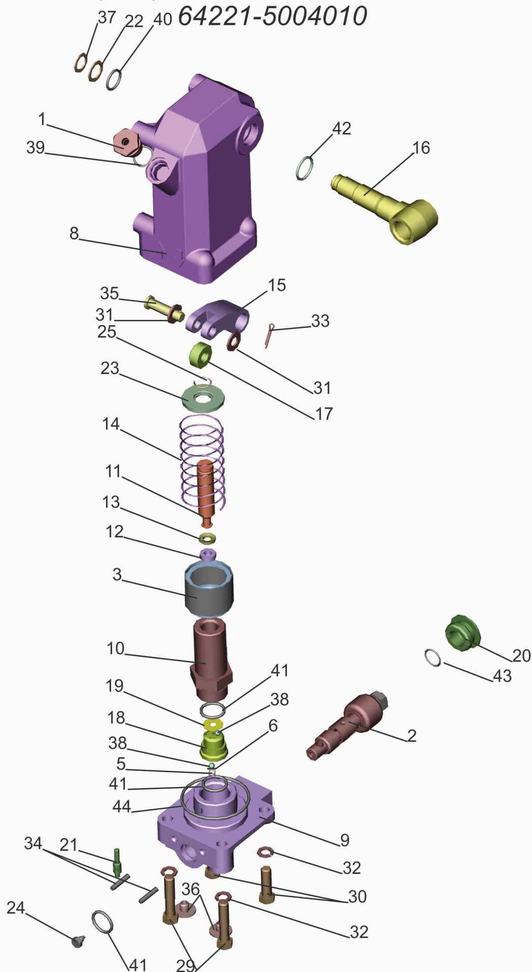
Fig. 210 The pump of the mechanism of rise of a cabin 64221-5004010
