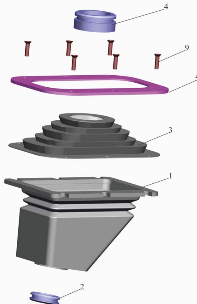
Fig.126 Sealing hatch of cabin 437141-3444256
