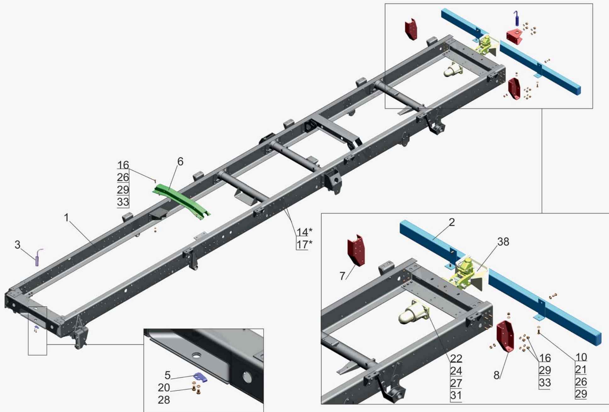
Рис. 74 Рама 4371P2-2800010-002, (-012) Fig.74 Frame 4371P2-2800010-002, (-012)
