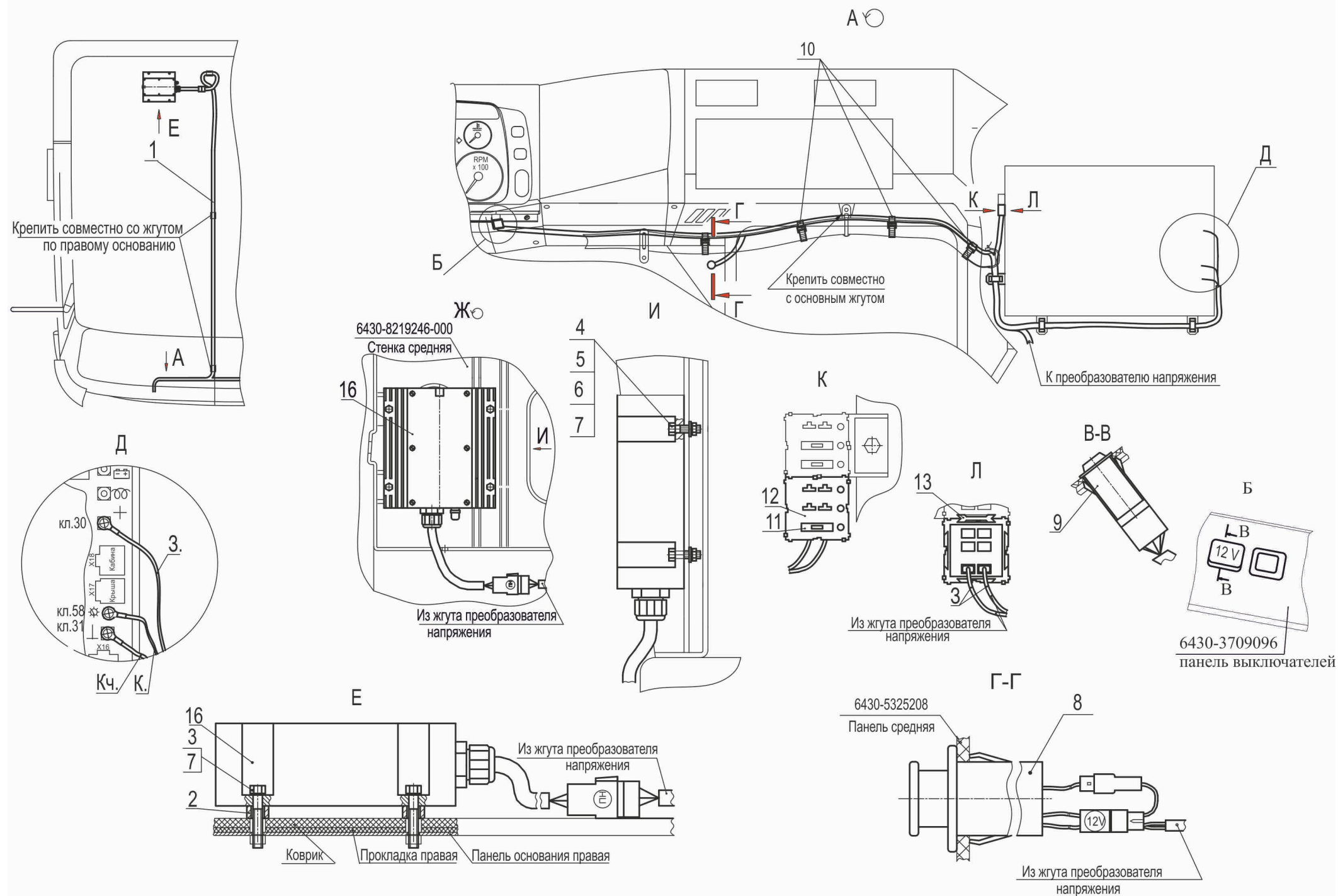
Fig.160 Installation of a voltage changer 6501A8-3700109-000
