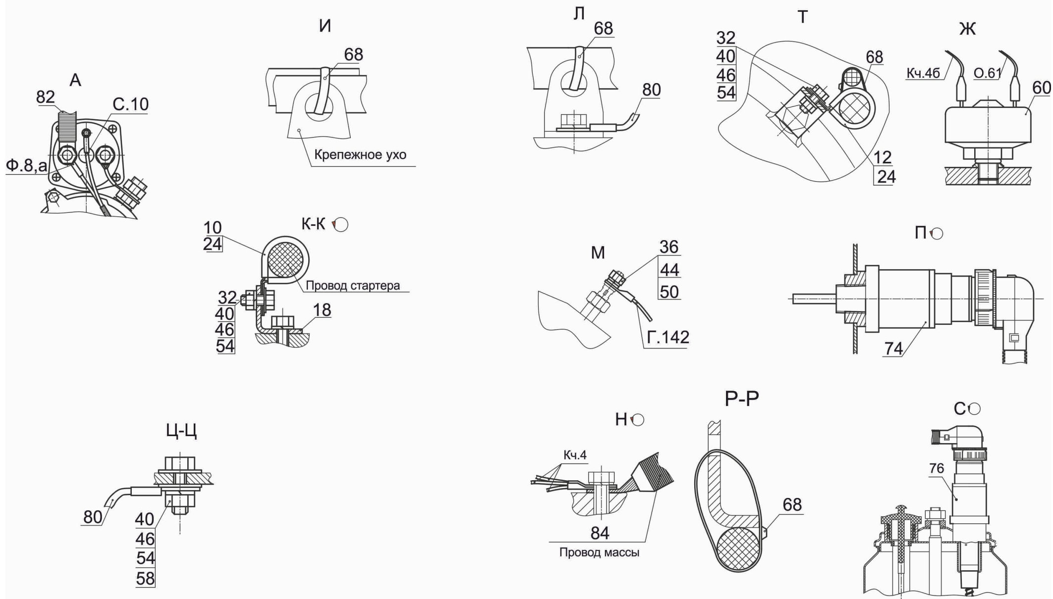
Fig. 157 Electric equipment installation on the engine Page 2
