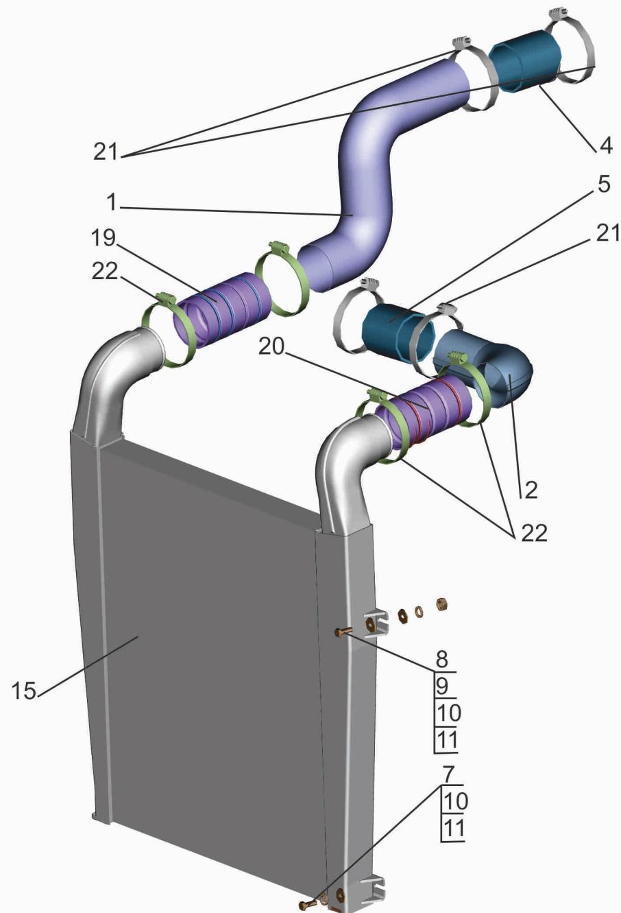
Fig. 29 Installation of a cooling system of air 4371P2-1300040-000
