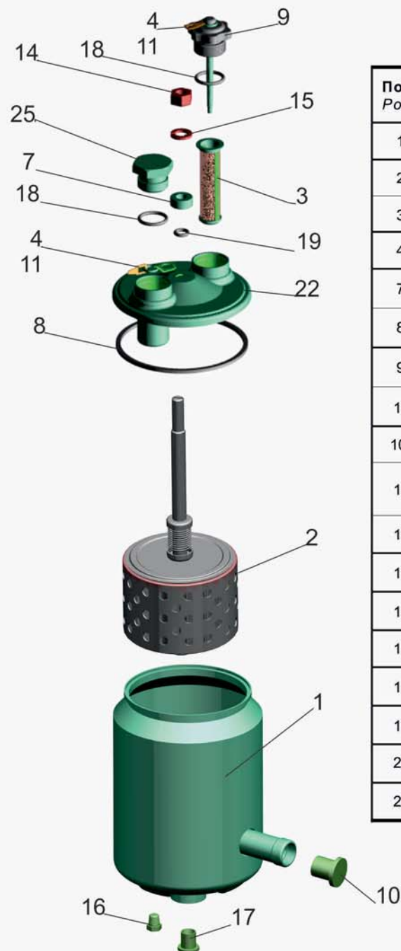
Fig. 121 Oil tank 5336-3410010-10
