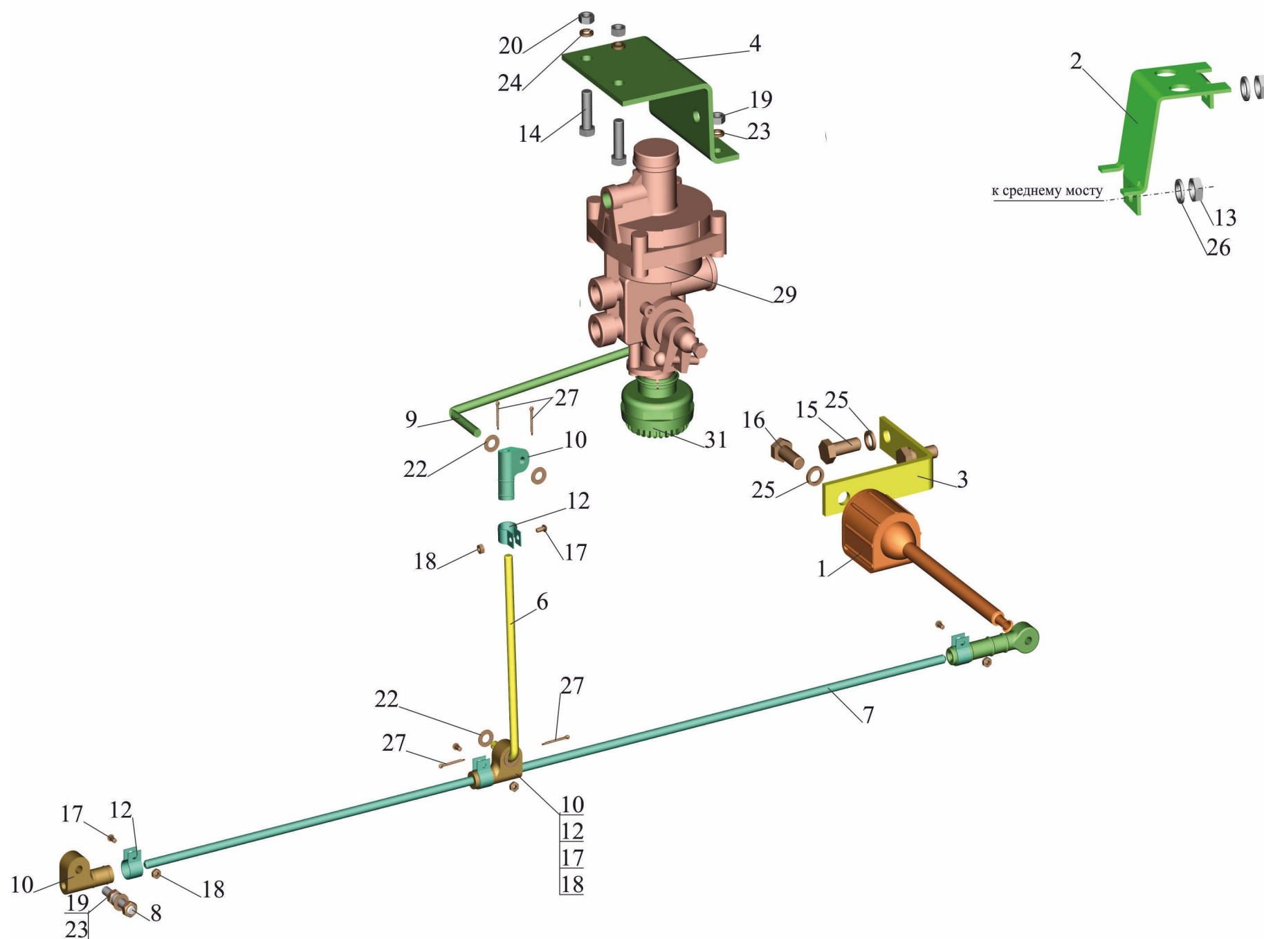
Fig. 177 Mounting of brake force regulator
