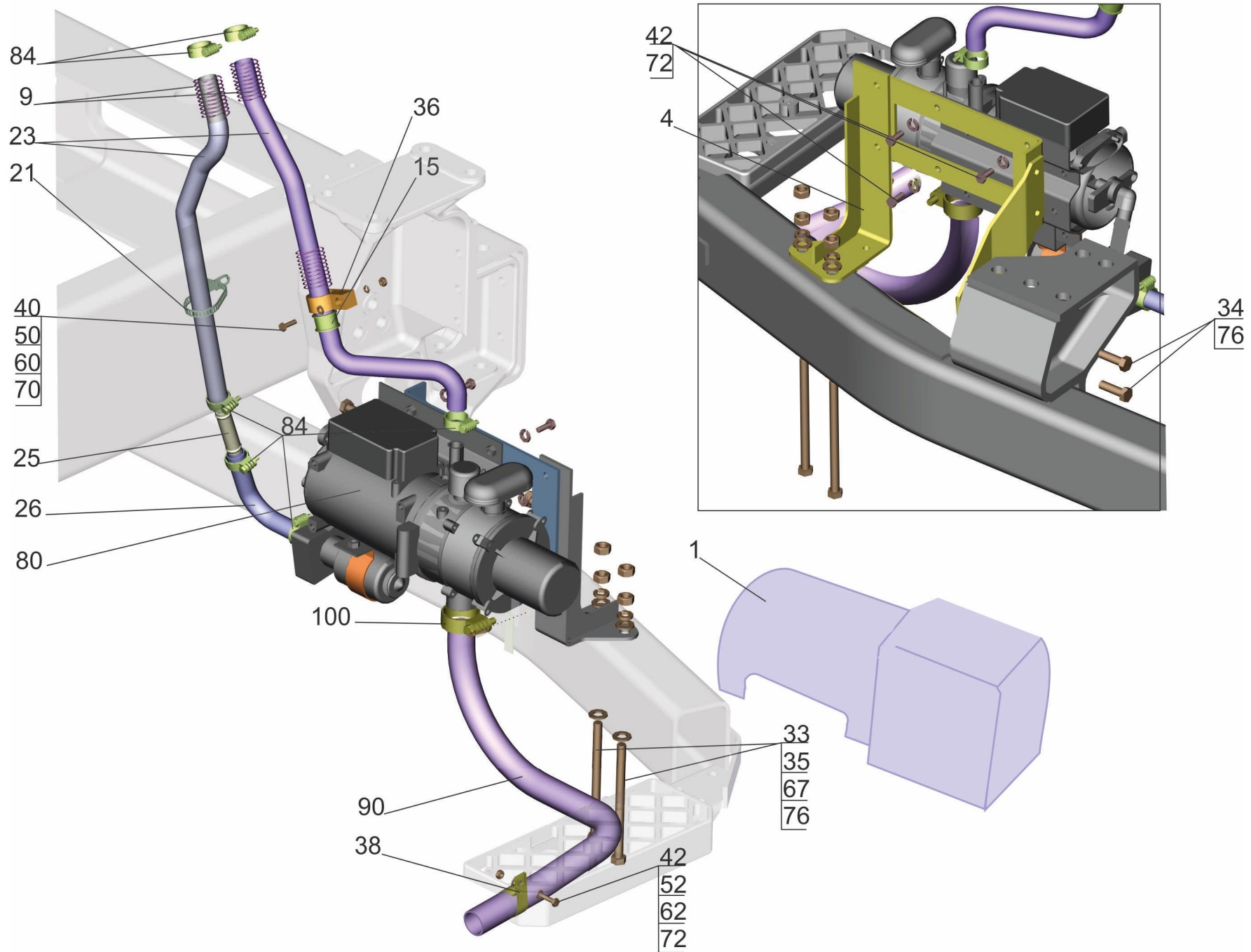
Fig. 9 Heater mounting
