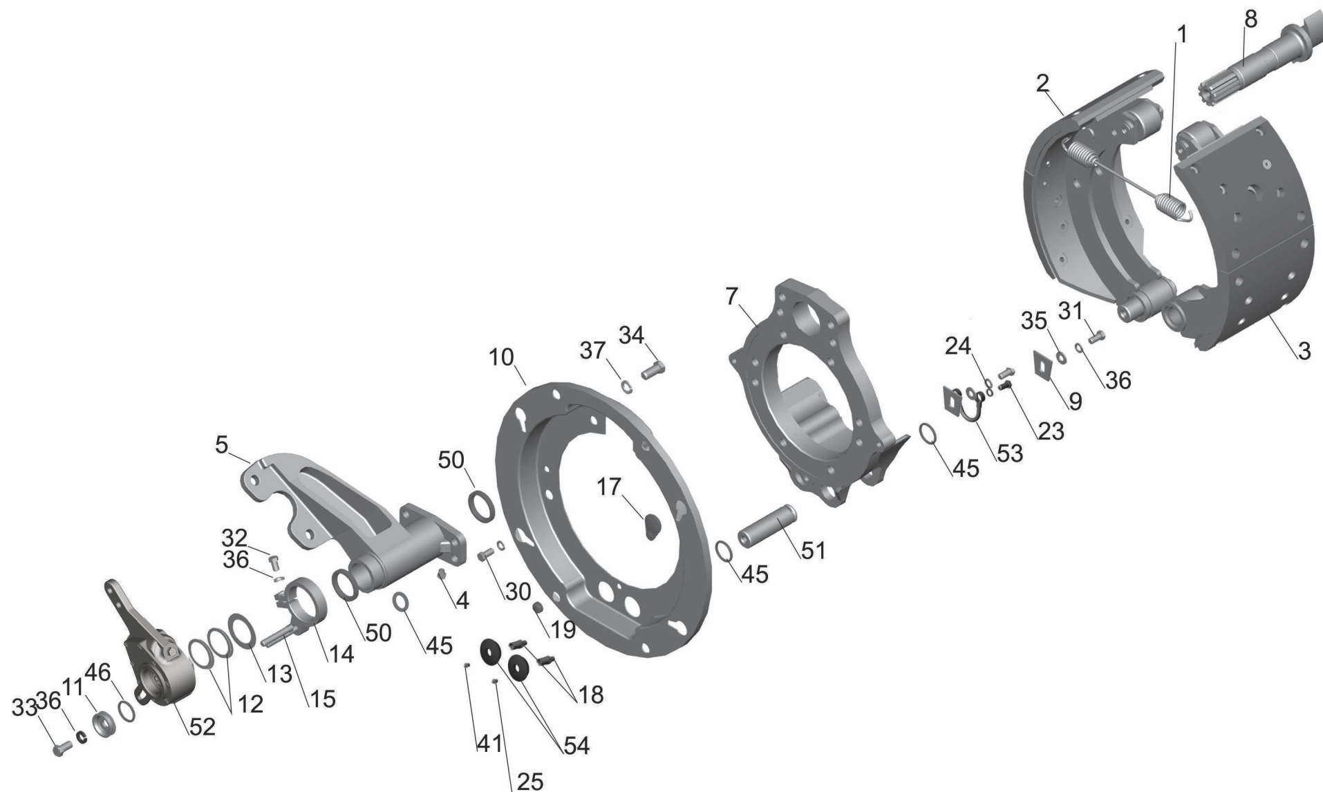
Fig. 132 Front brake 5440-3501004 (5440-3501005)
