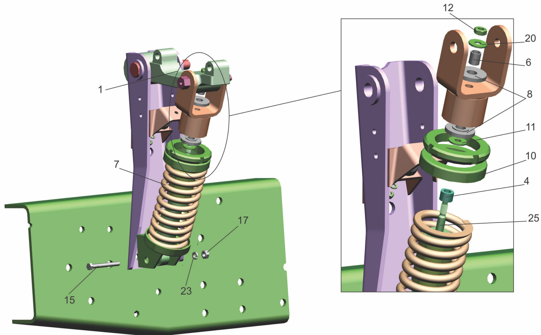
Fig. 231 Rear springing 6430-5001800-011
