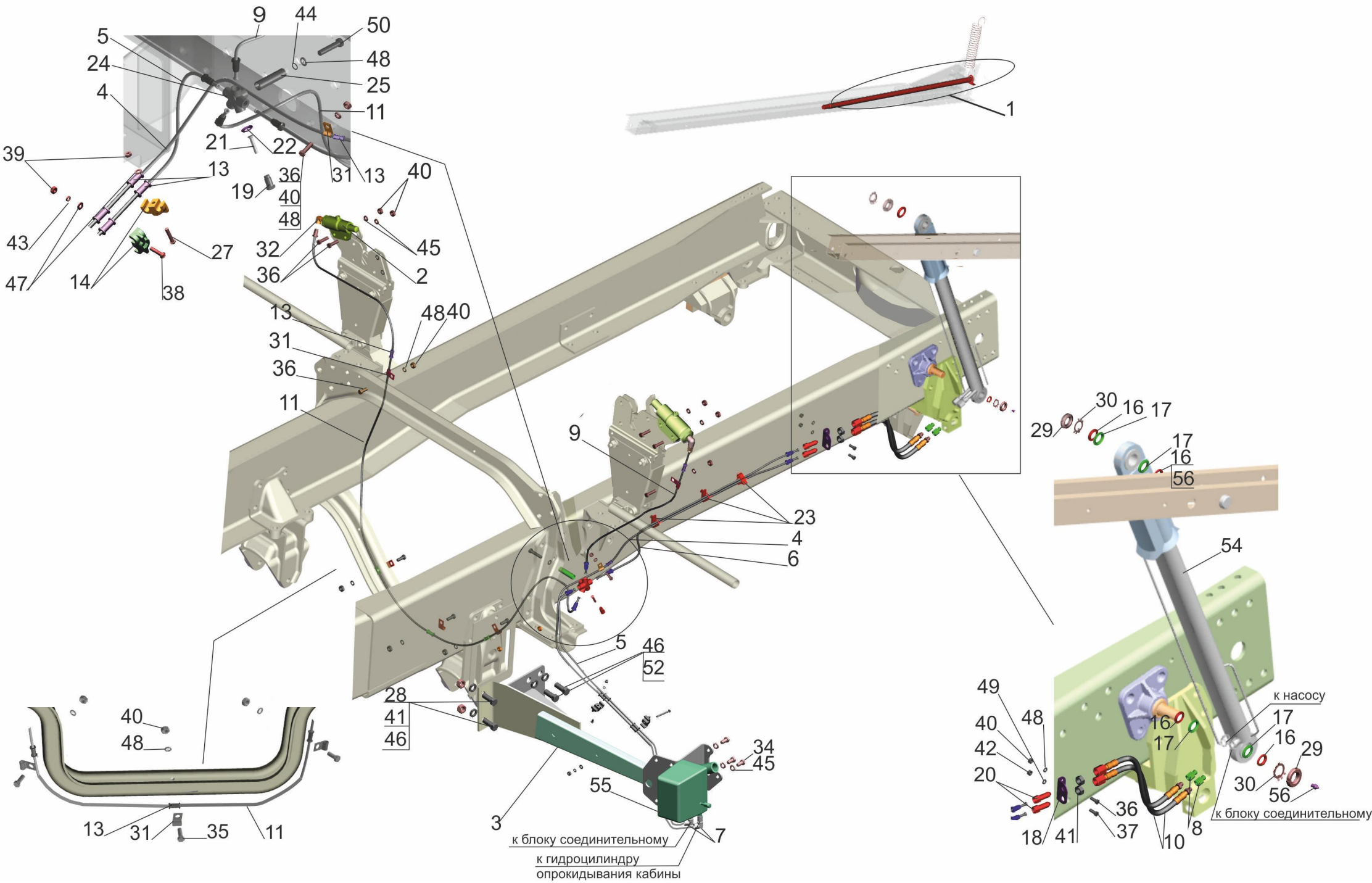
Fig. 277 Installation cab tilting mechanism 6501B9-5000040-011
