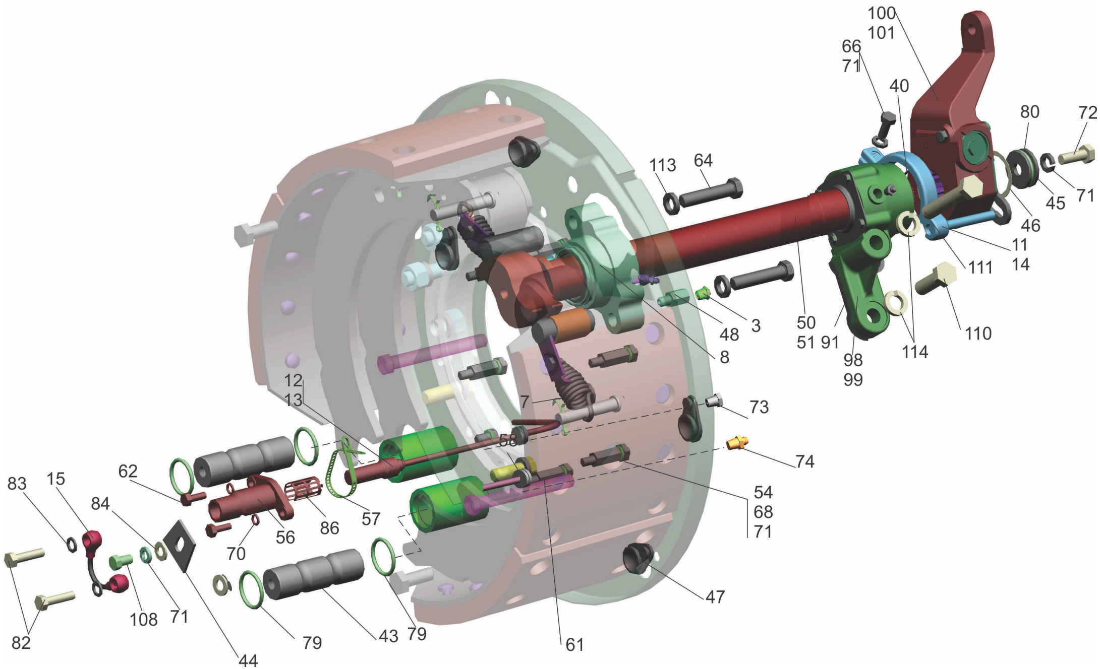
Fig.62 Rear axle Page 2
