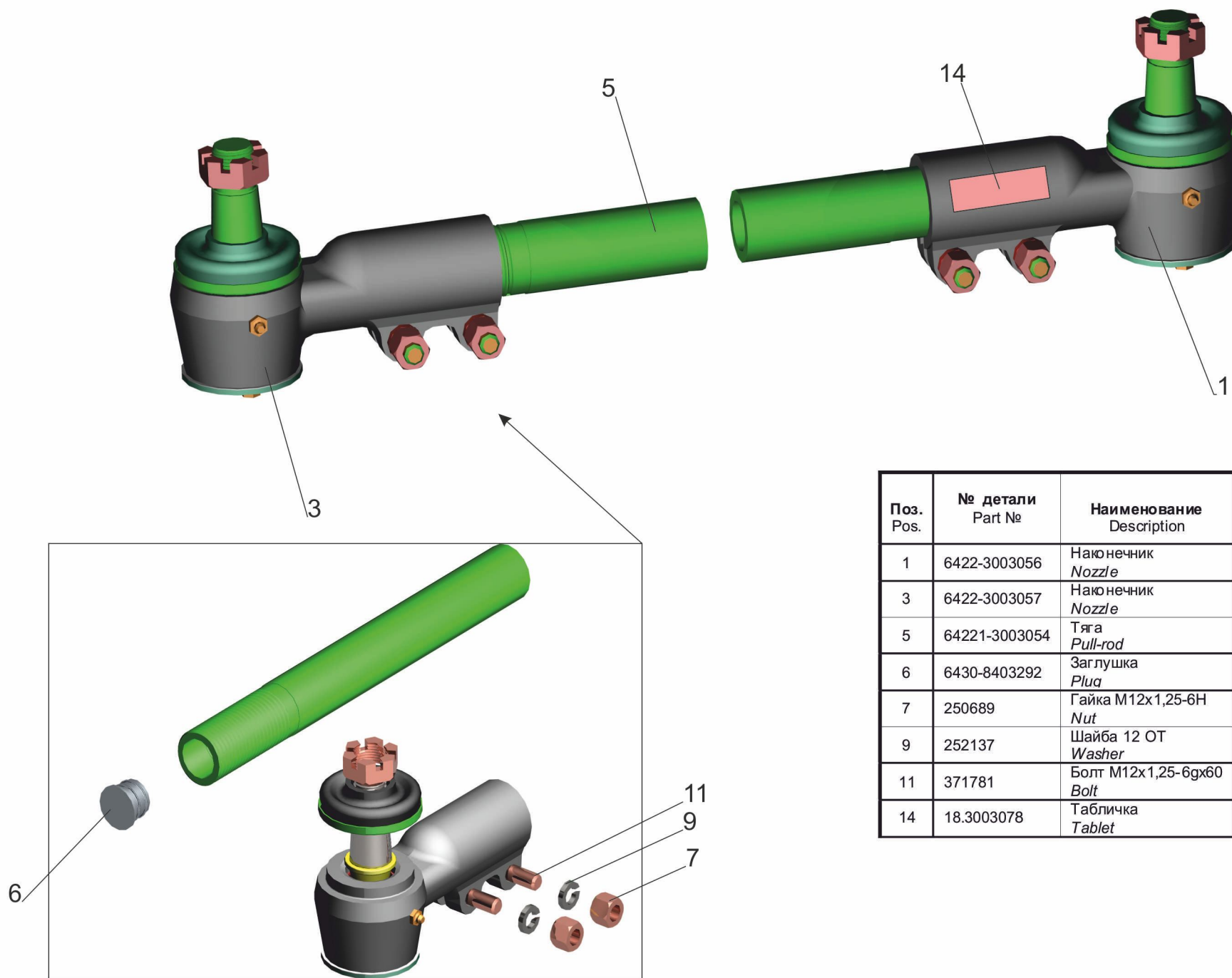
Fig. 125 Pull-rod cross 64221-3003052
