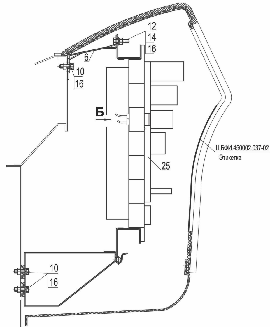
Рис. 206 Установка БКА-N4 6430A9-3700110-000 Fig.206 Installation of switchgear unit 6430A9-3700110-000
