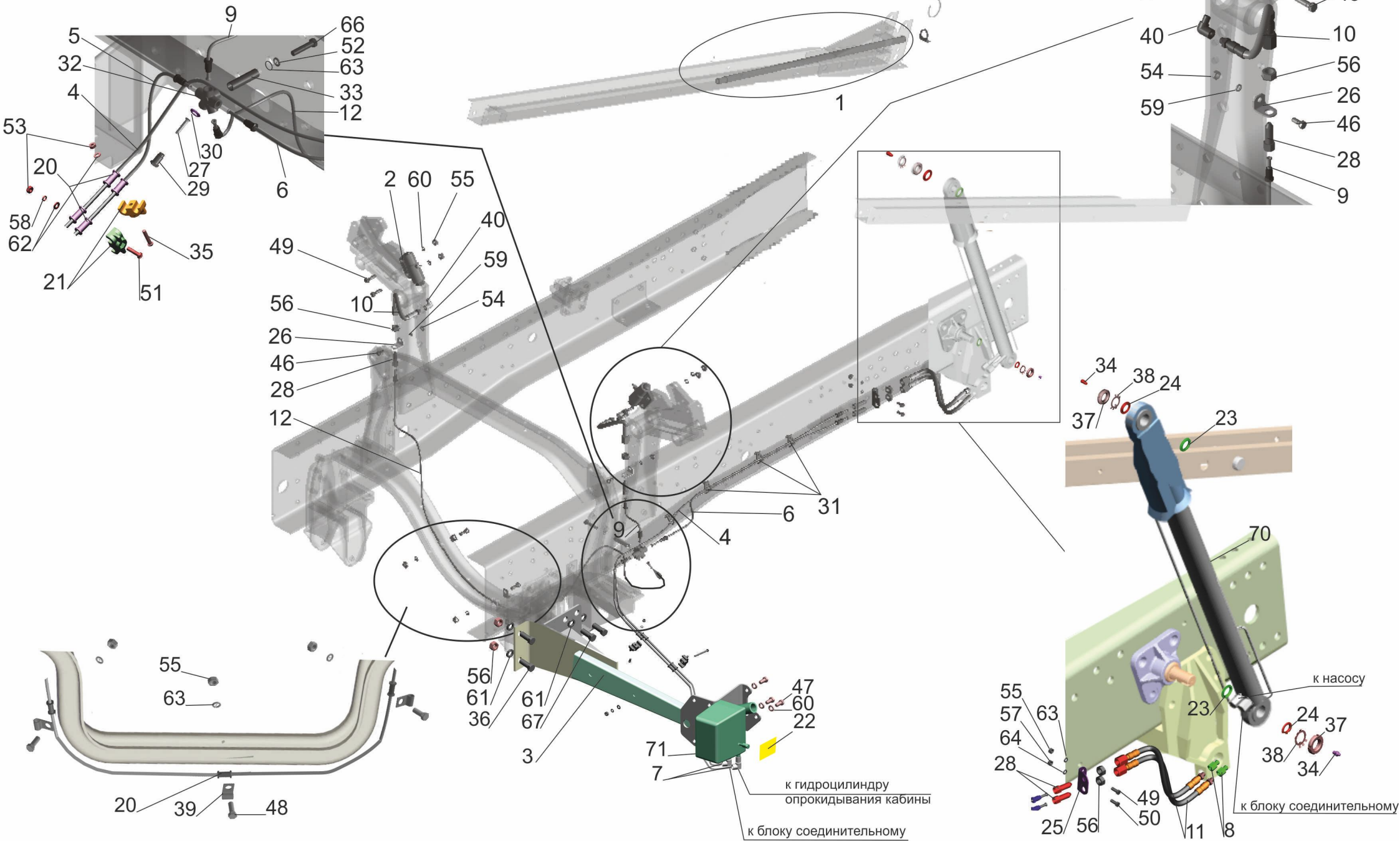
Fig. 278 Installation cab tilting mechanism 6312B5-5000040-000
