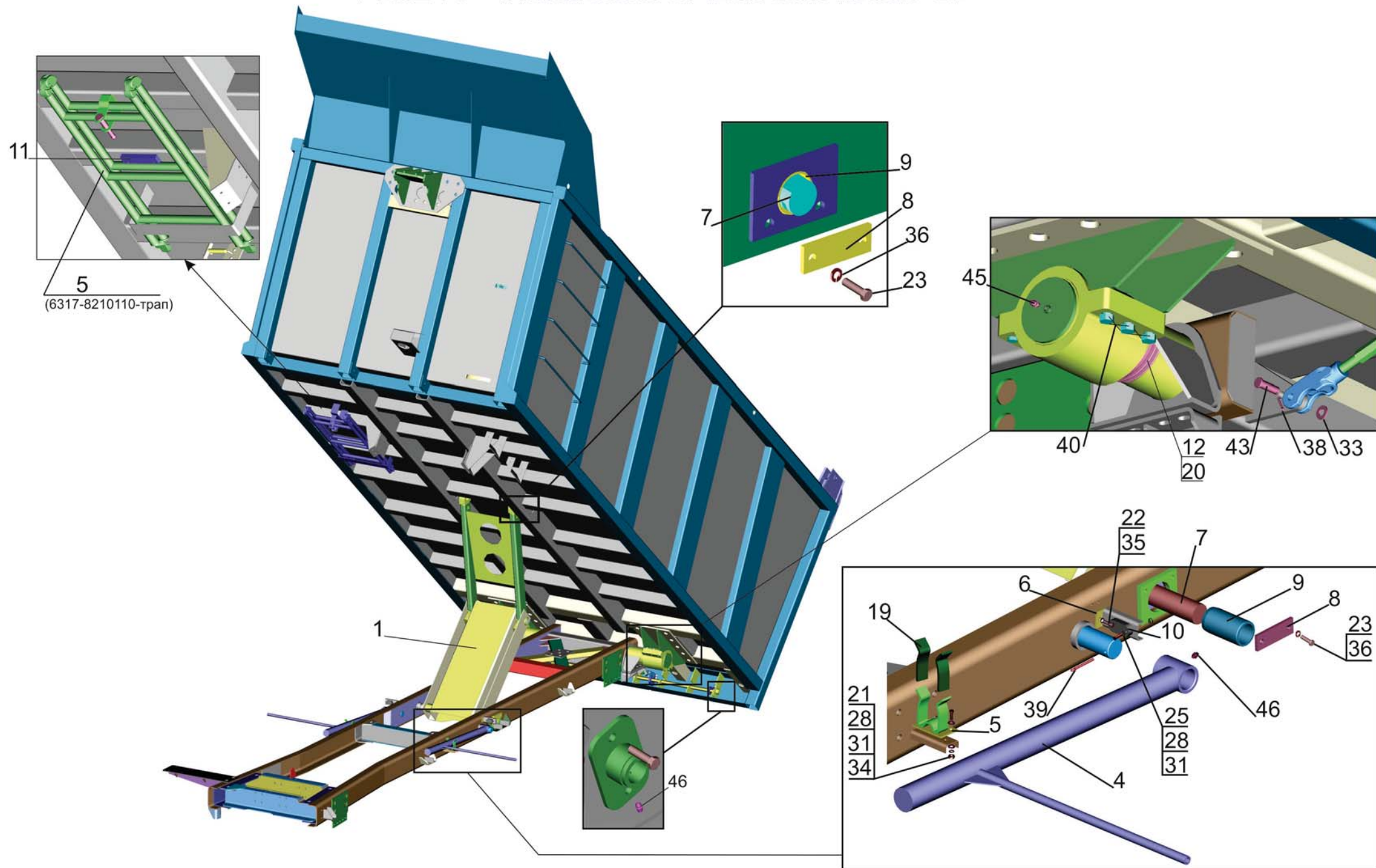
Fig.248 Installation of platform (page 2)
