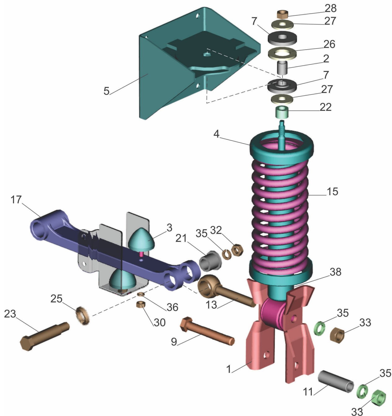
Fig. 230a Cab rear springing 6501-5001802-010
