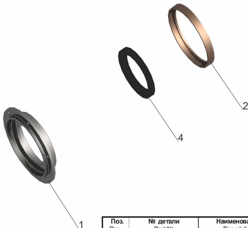
Fig. 131 Cover 54326-3103034-001
