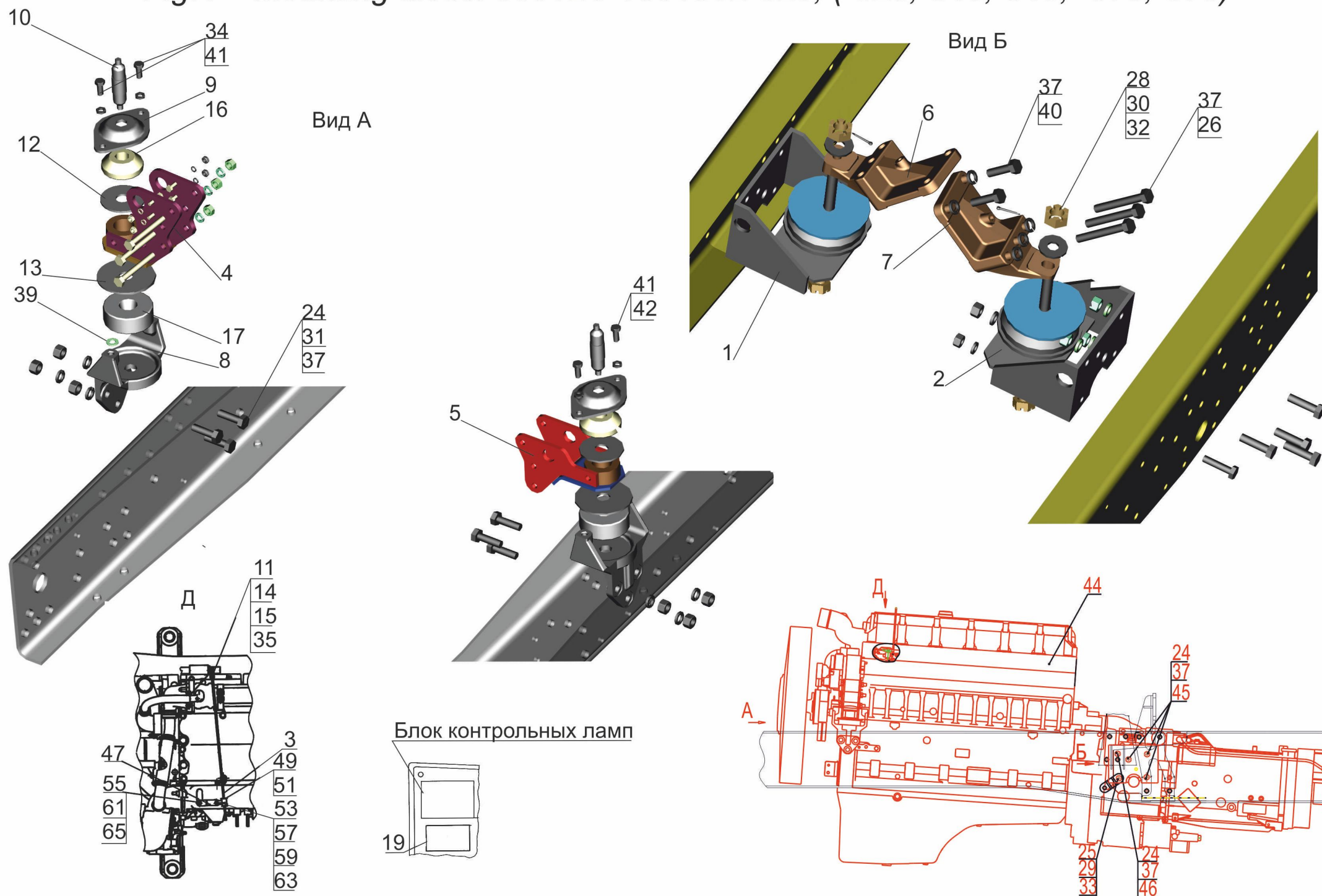
Fig.4 Mounting diesel 6501B9-1001002-320, (-325,-340,-345, -370,-375)
