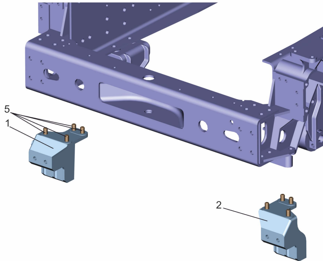
Fig. 109 Installation of buffer stop 6430B9-2800032-000
