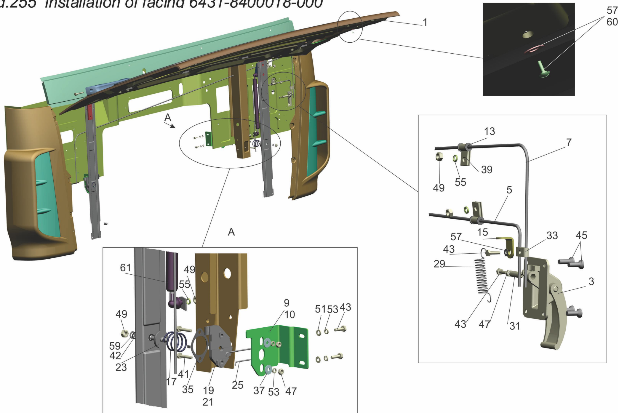
Fig.255 Installation of facing 6431-8400018-000
