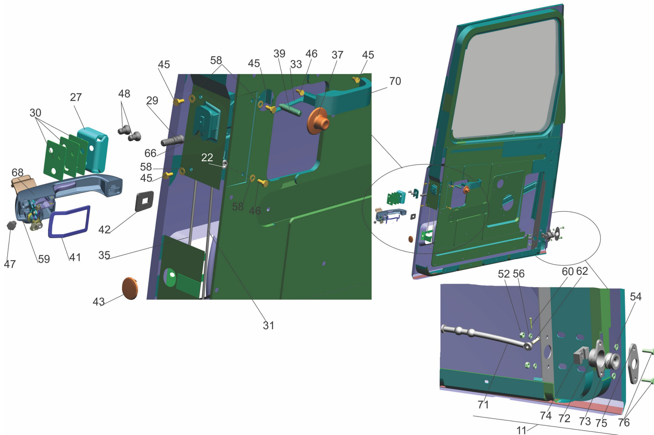
Fig. 248 Installation of door armature 6430-6100010, 6430-6100011 (page 1)
