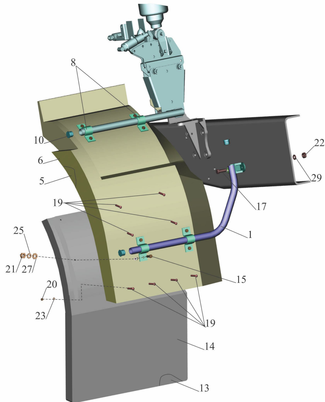
Fig. 322 Installation of mudguard 6501-8400030-011
