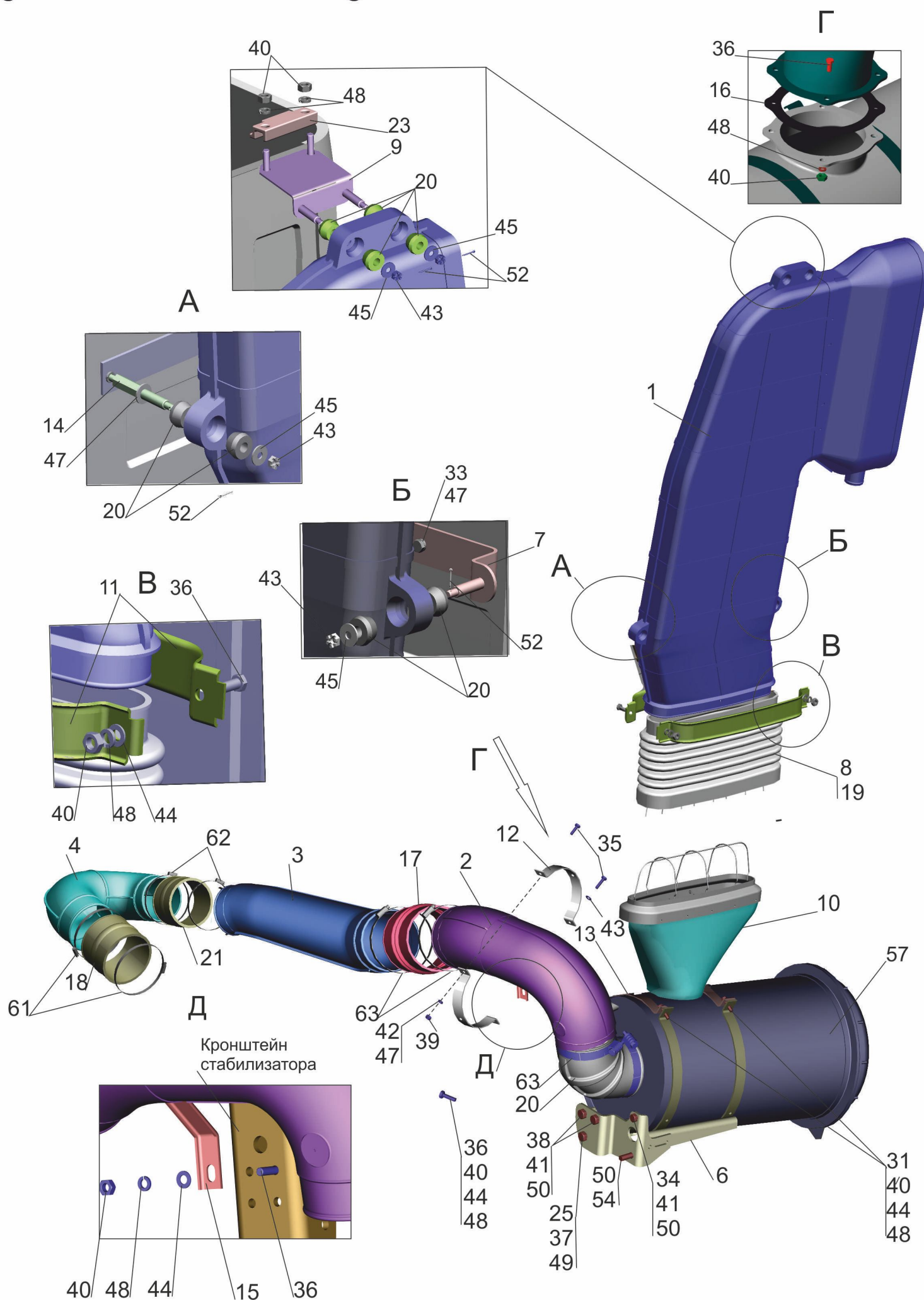
Fig. 27 Air filter mounting 6501B9-1109002-060
