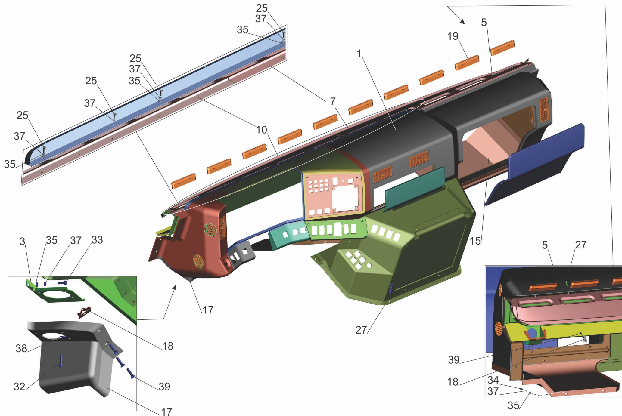
Fig. 245 Installing of instrument panel 6430-5300014-020.
