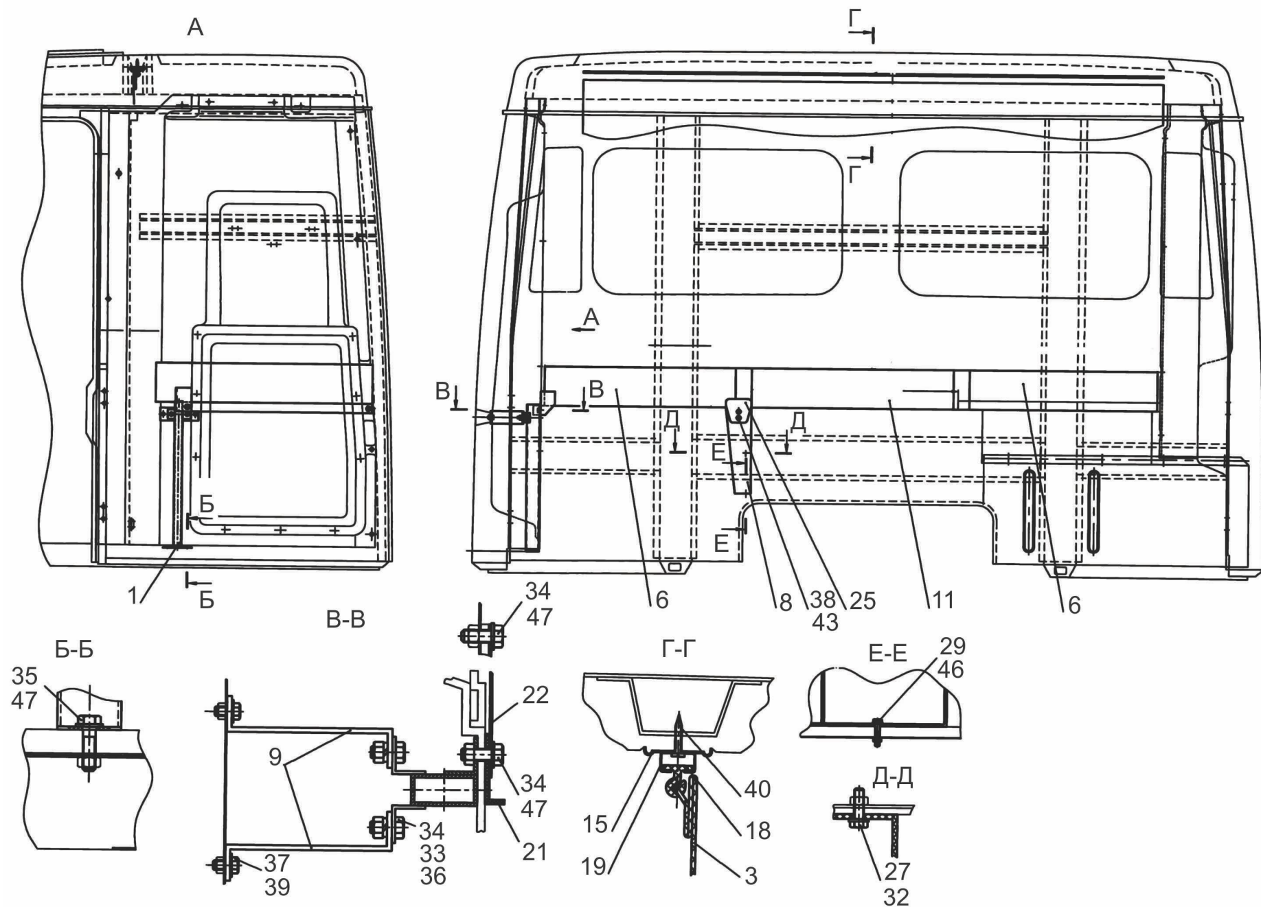
Fig. 275 Installation of a berths 5440-8200010
