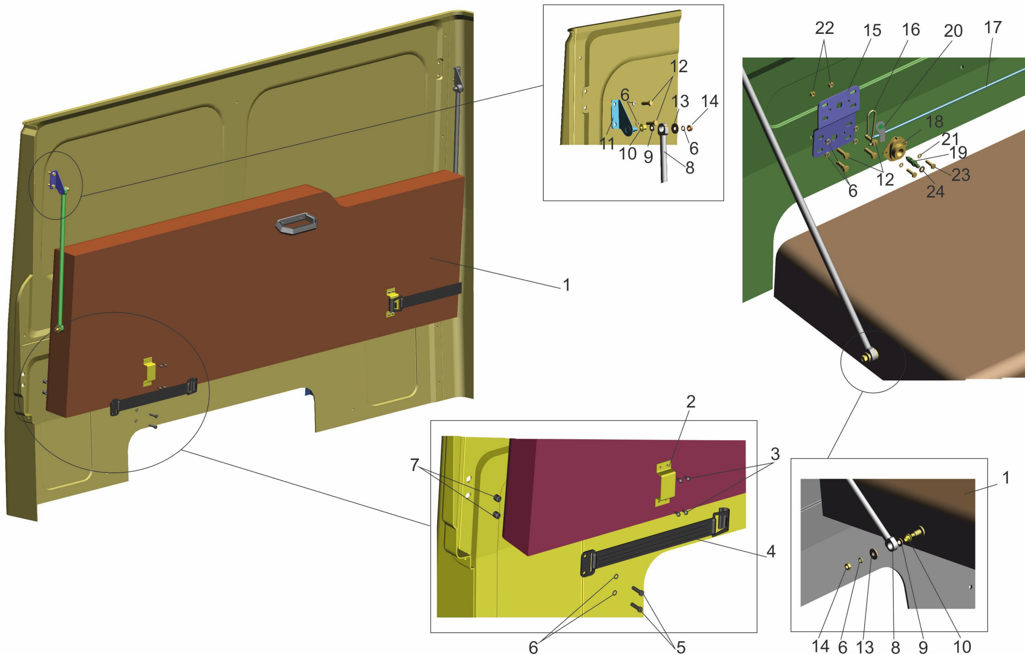
Fig. 312 Installation of a berth 6501-8200010
