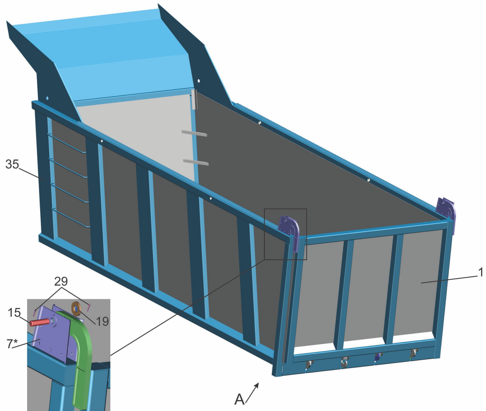
Fig.325 Platform
