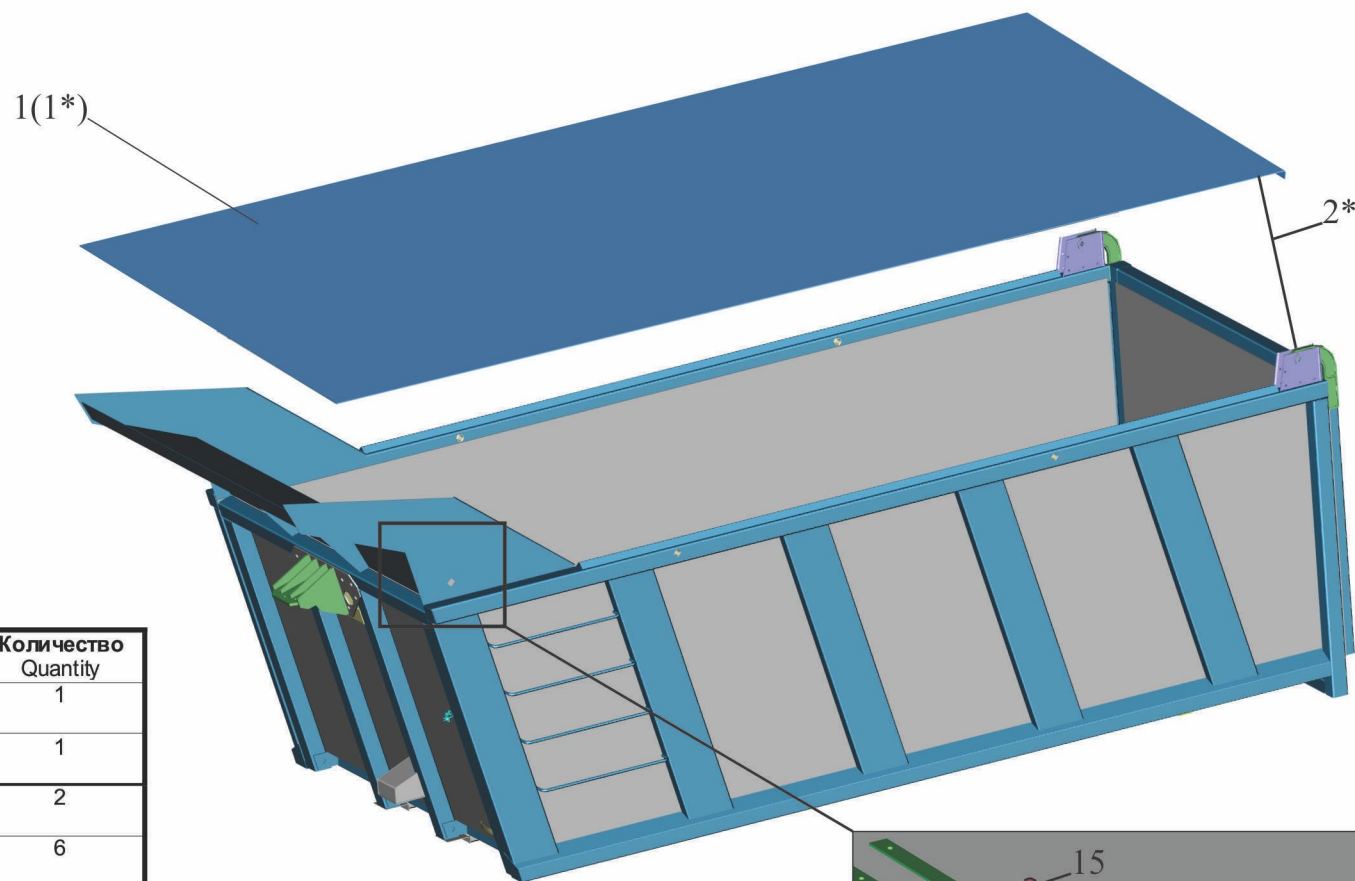
Fig. 326 Installation of canopy 651608-8500004
