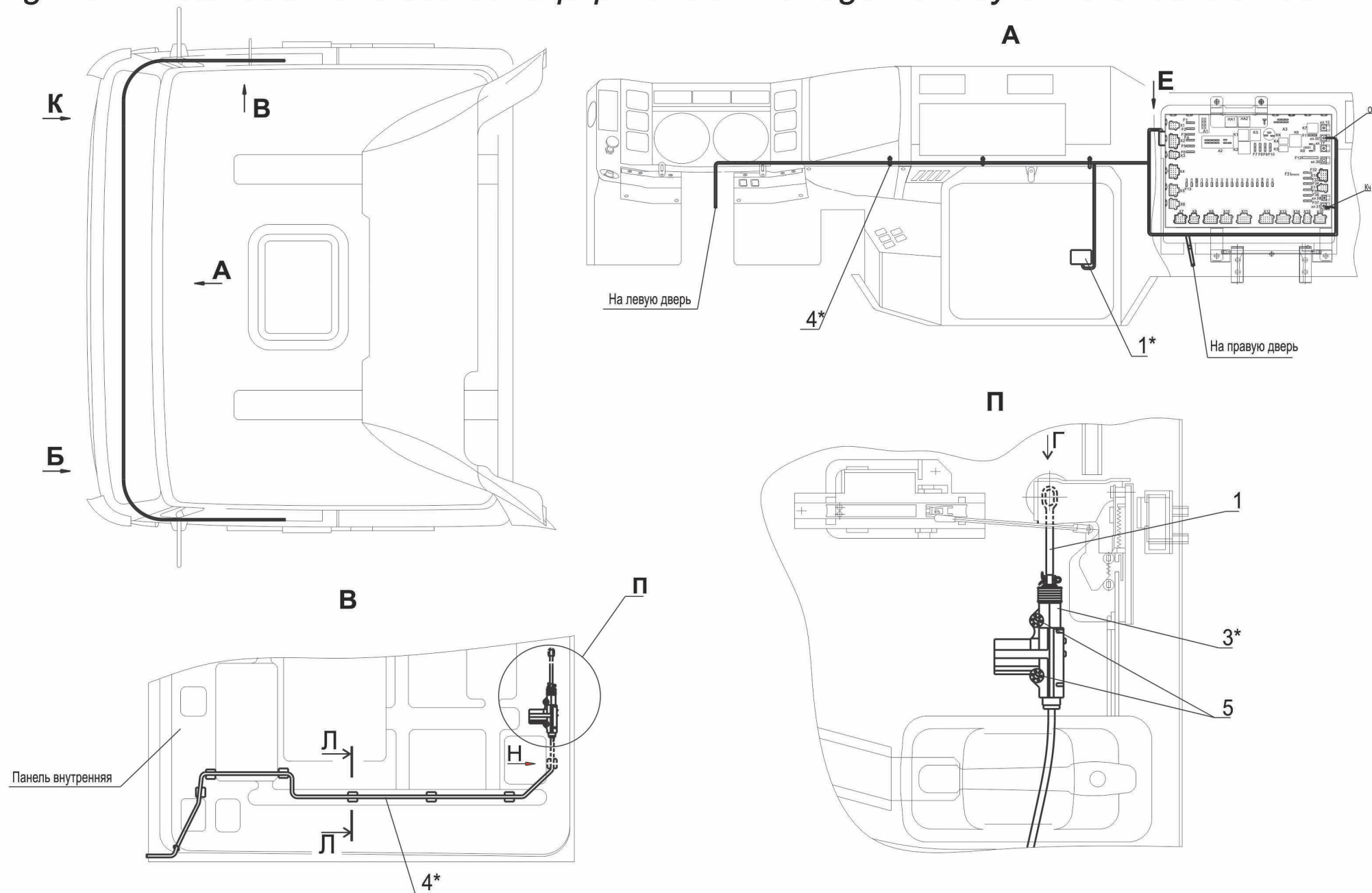
Fig. 192 Installation of electrical equipment of management by drive of central lock
