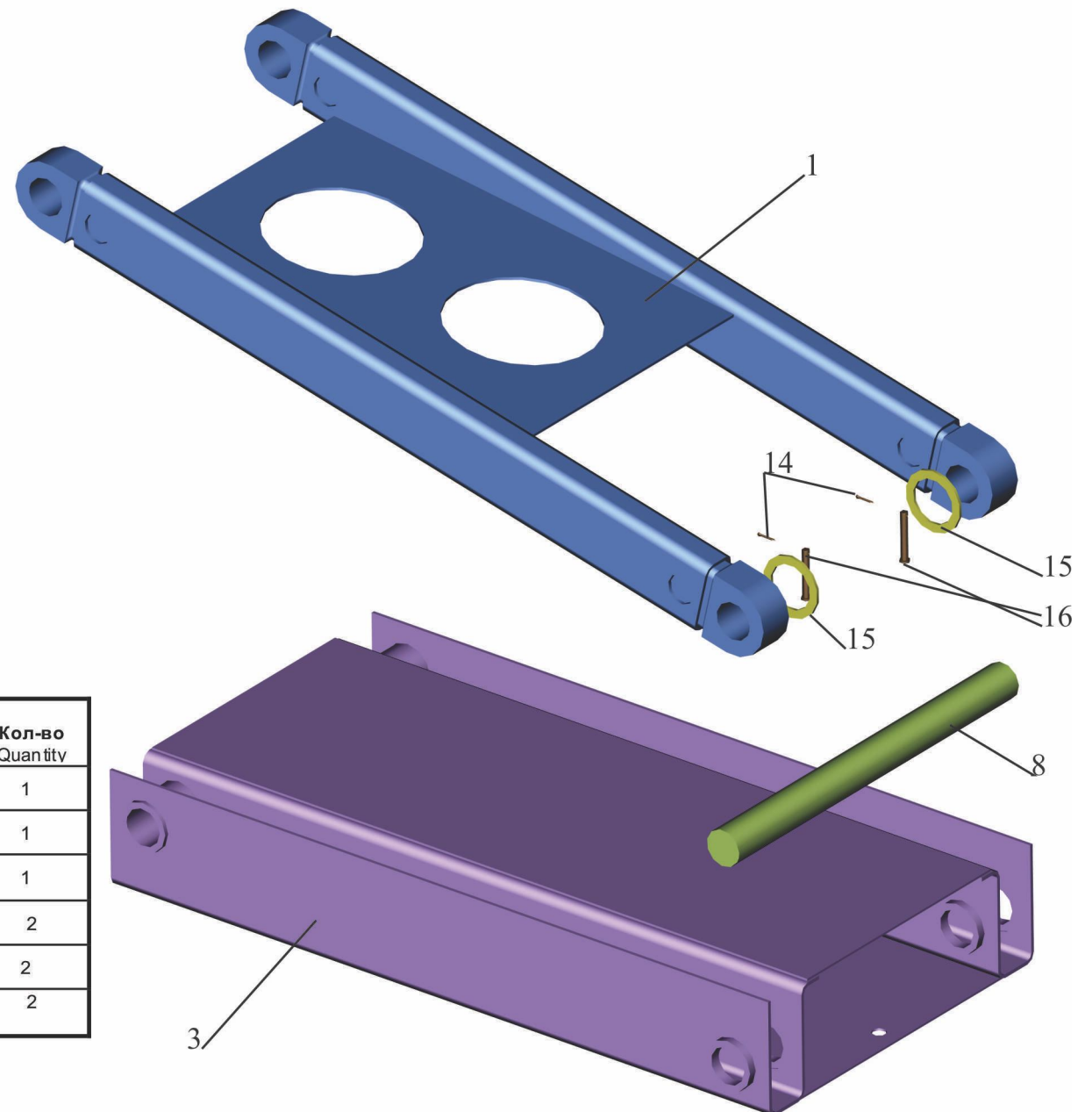
Fig.324 Limited frame 650136-2815011
