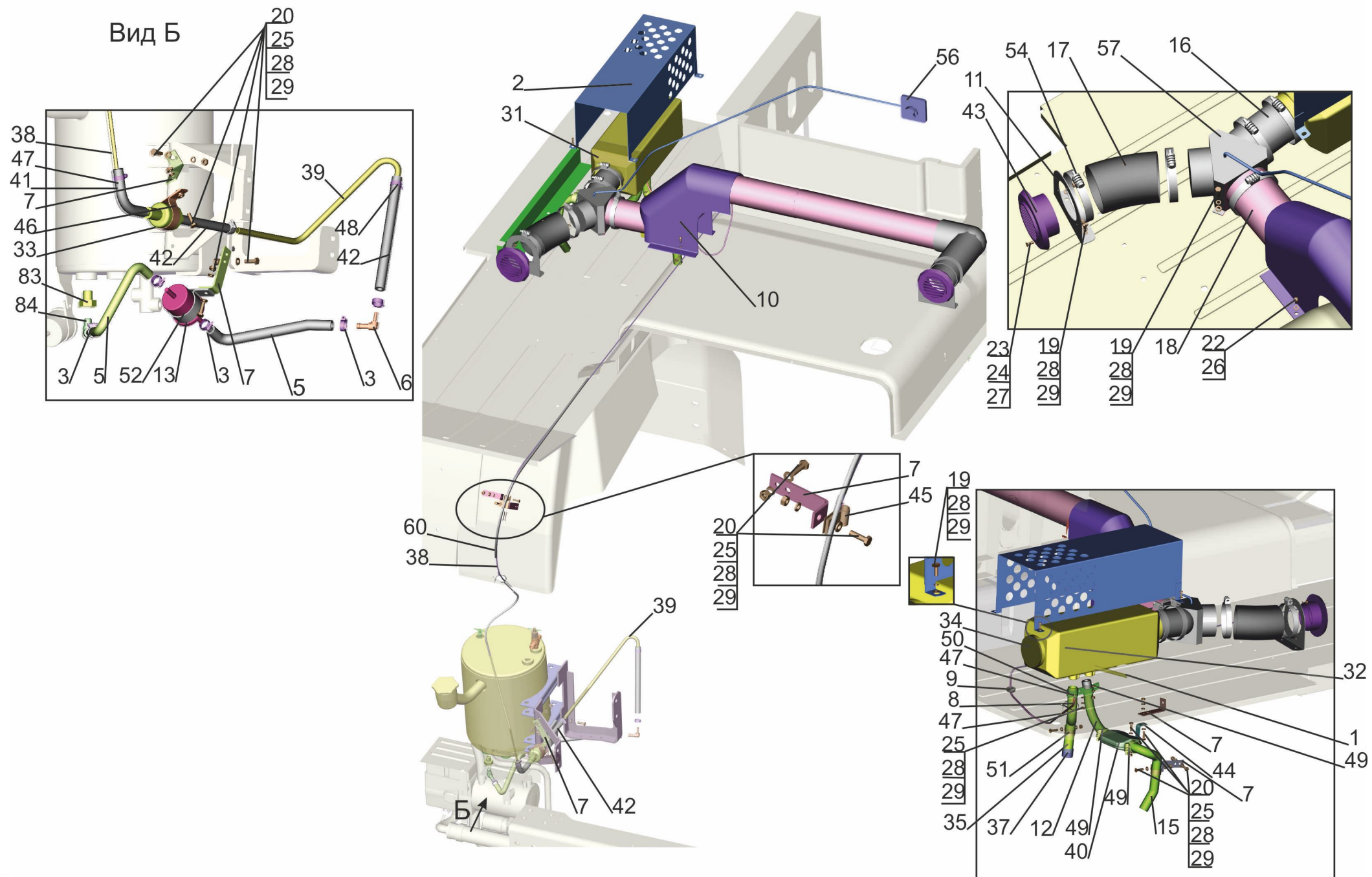
Fig. 295 Installation of the independent air heater 6430-8100002
