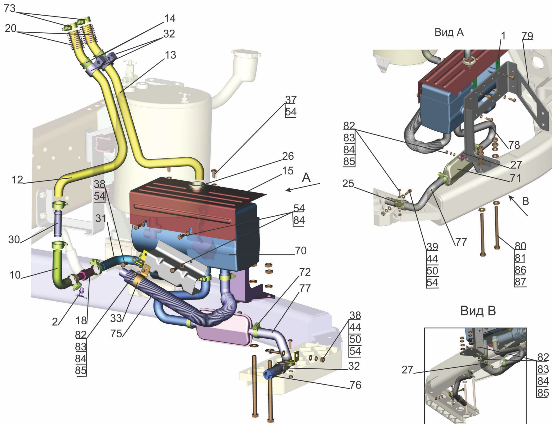
Fig. 8 Heater mounting 555035-1015001-010
