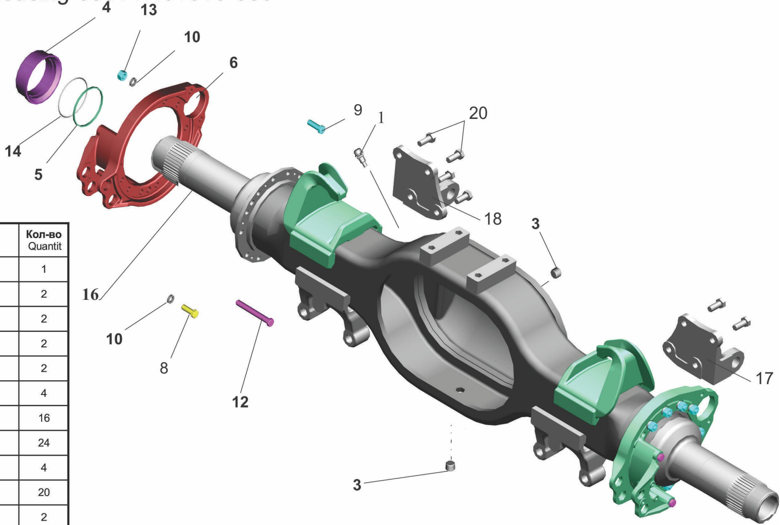
Fig. 70 Rear axle. Axle housing 6501-2401010-030
