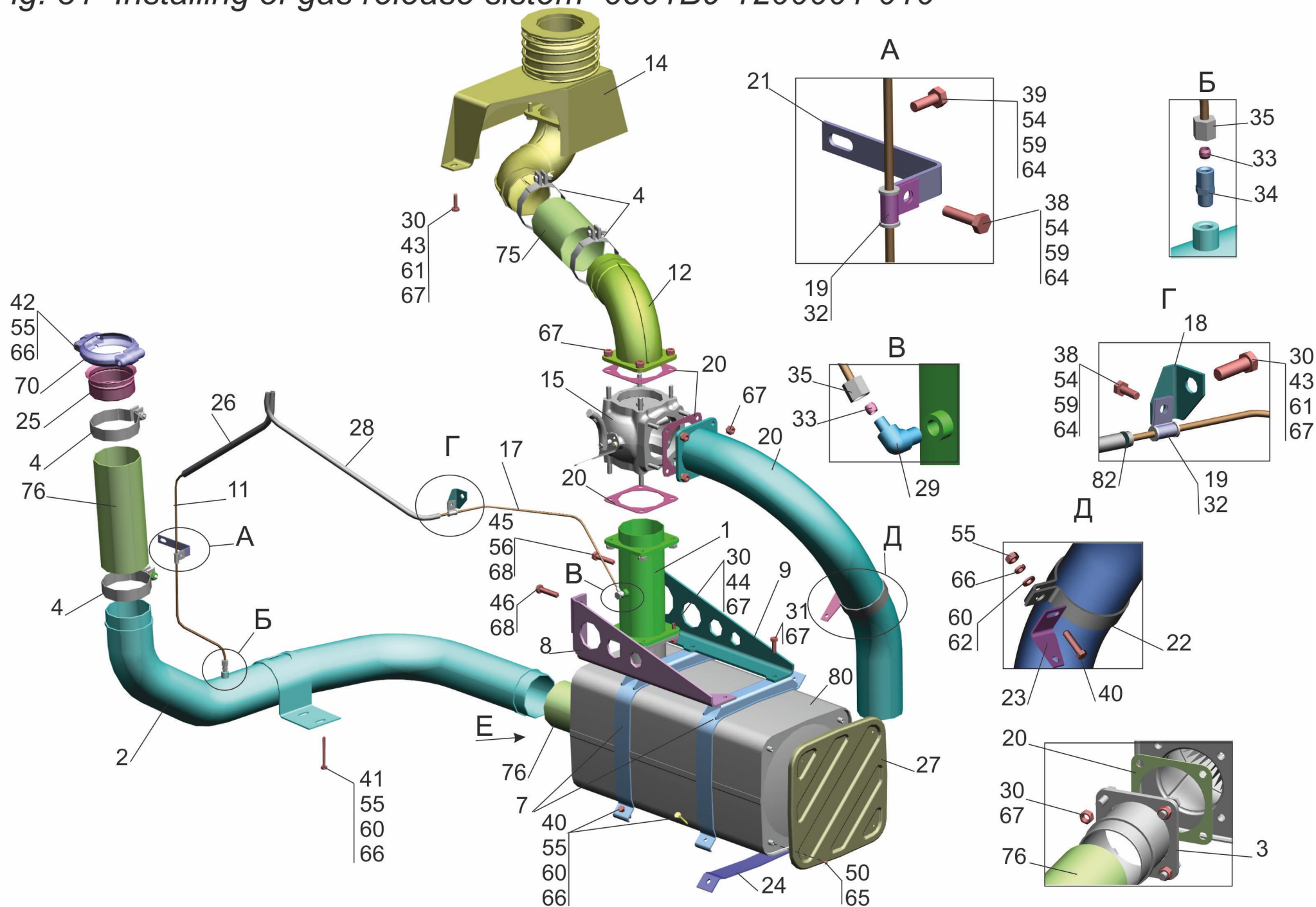
Fig. 31 Installing of gas release sistem 6501B9-1200001-010
