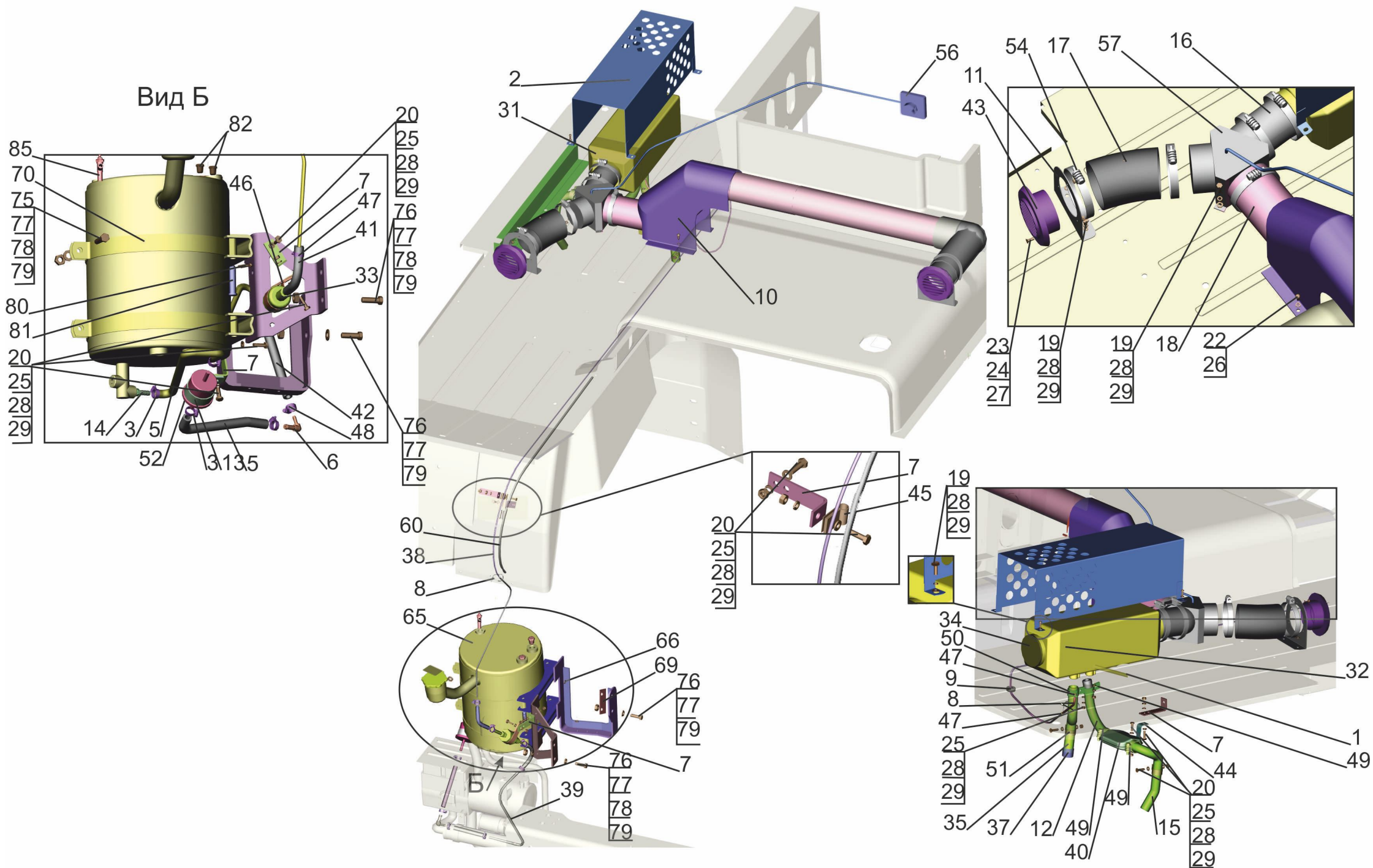
Fig. 297 Installation of the independent air heater 6430-8100002-010
