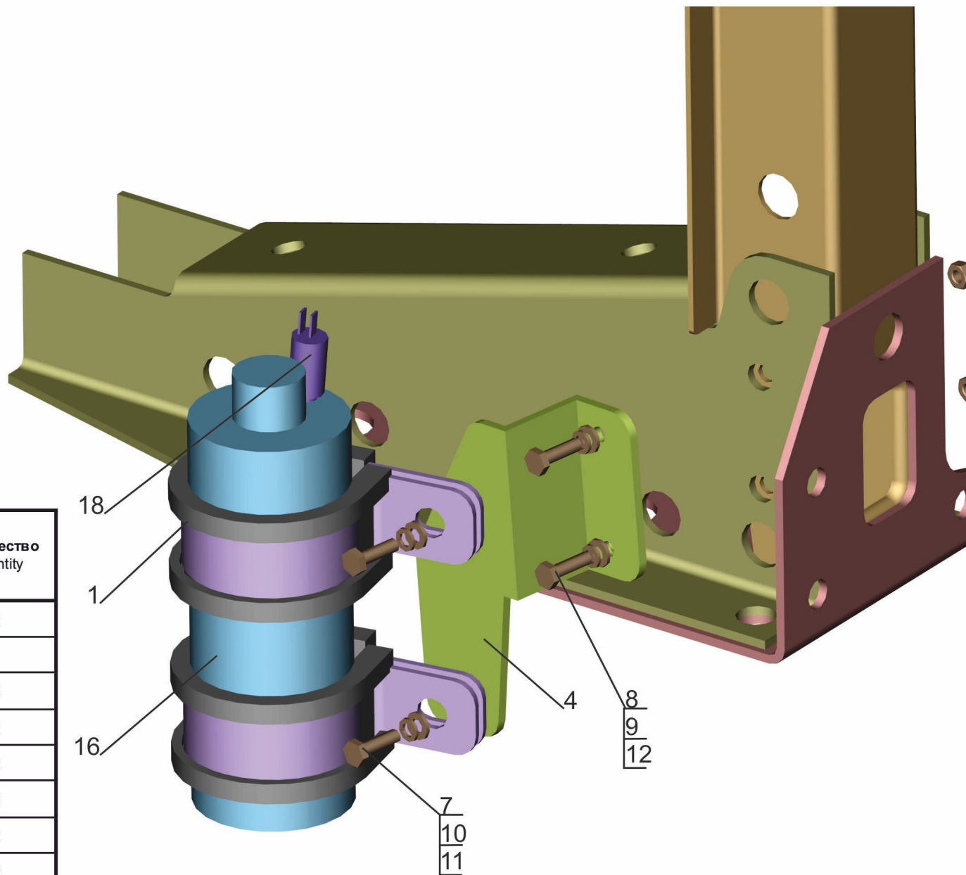
Fig. 308 Installation of receiver-drier 544020-8100036
