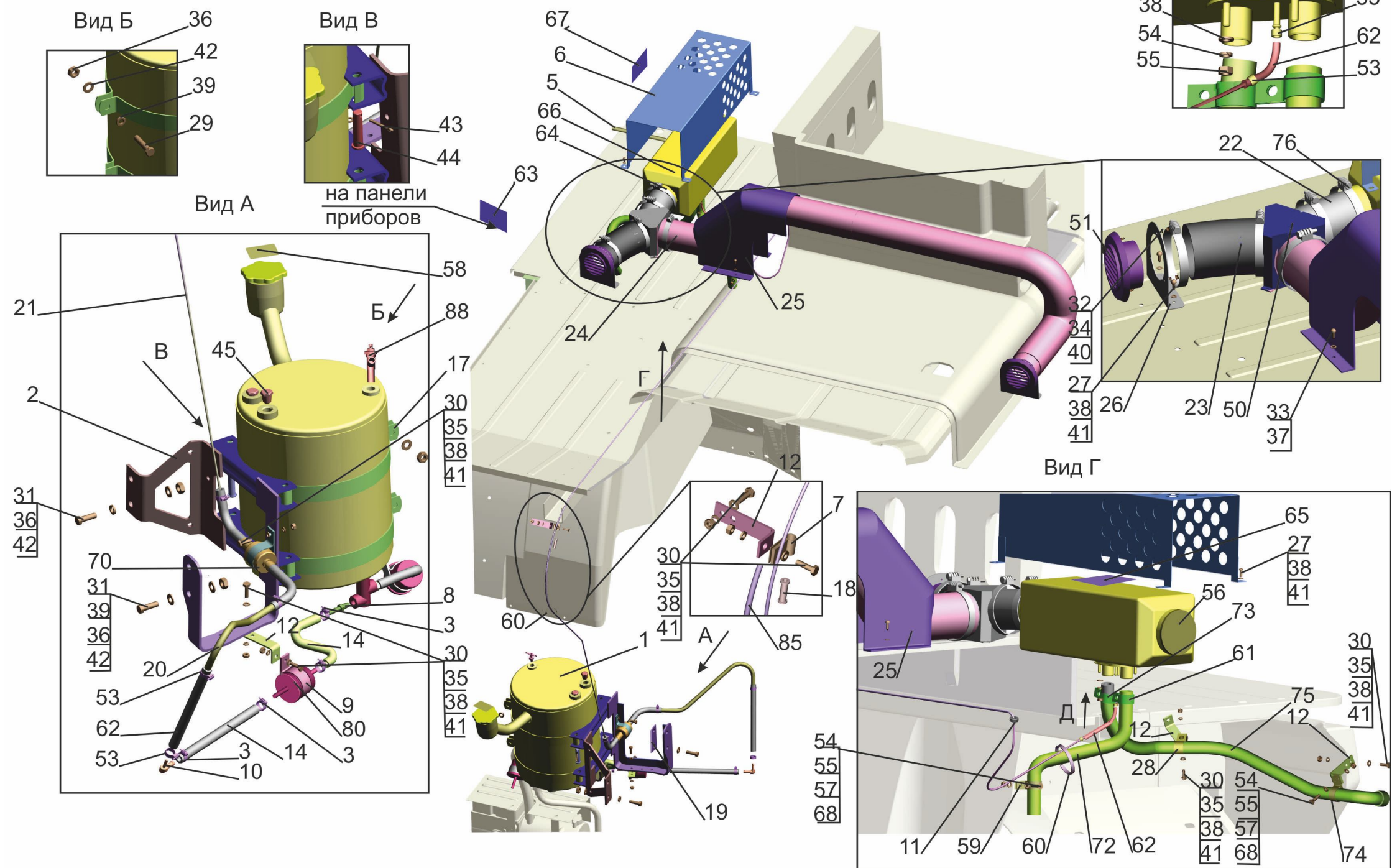
Fig. 298 Installation of the independent air heater 6430-8100002-011
