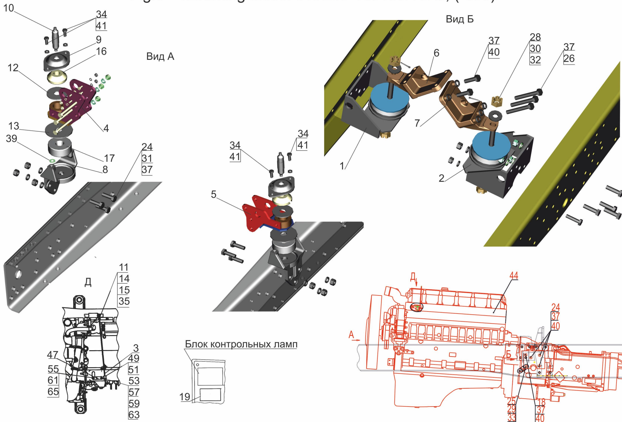
Fig.3 Mounting diesel 6430В9-1001002-020, (-030)
