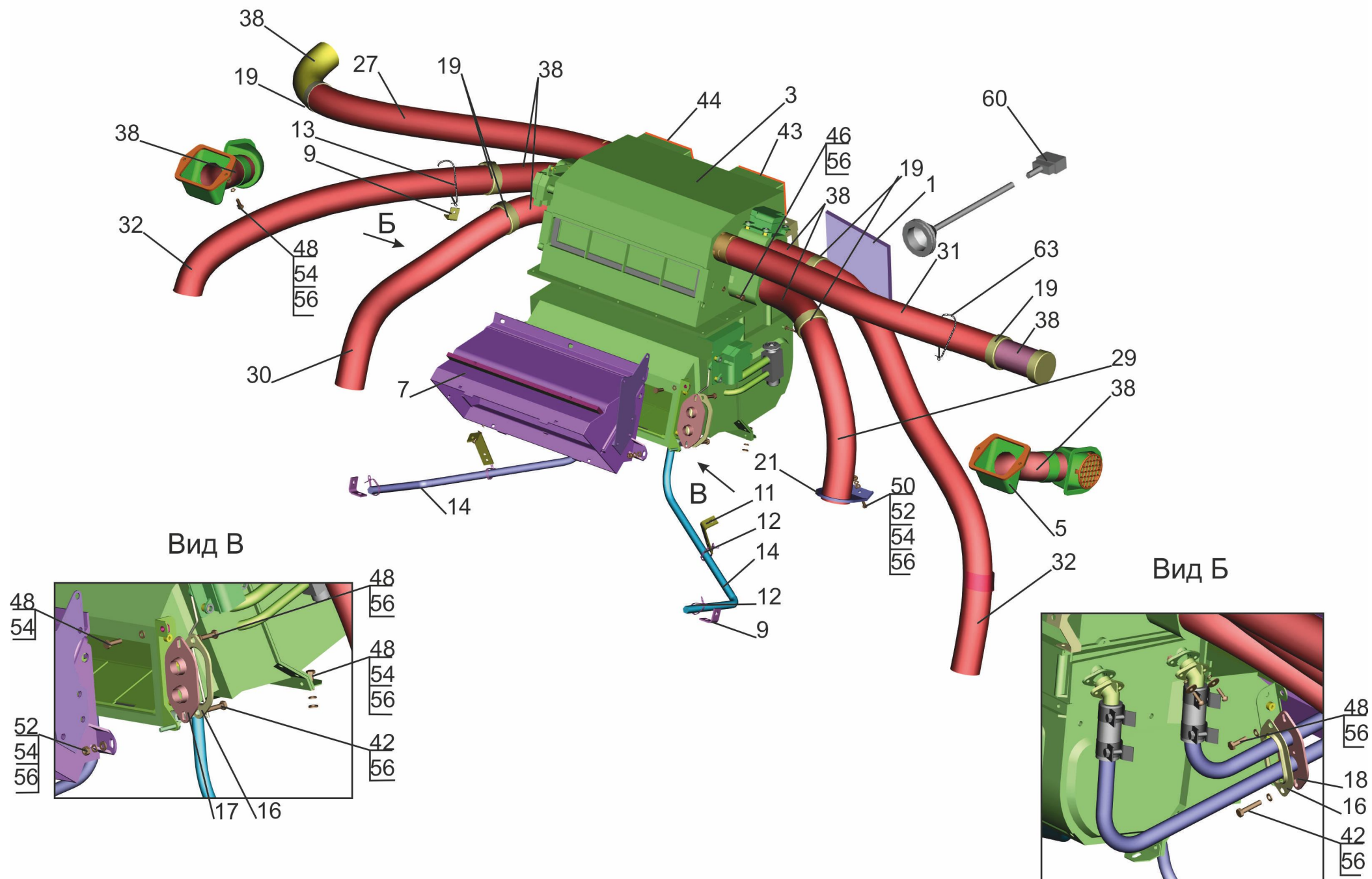
Fig. 282 Installation of heater 631019-8100001-010
