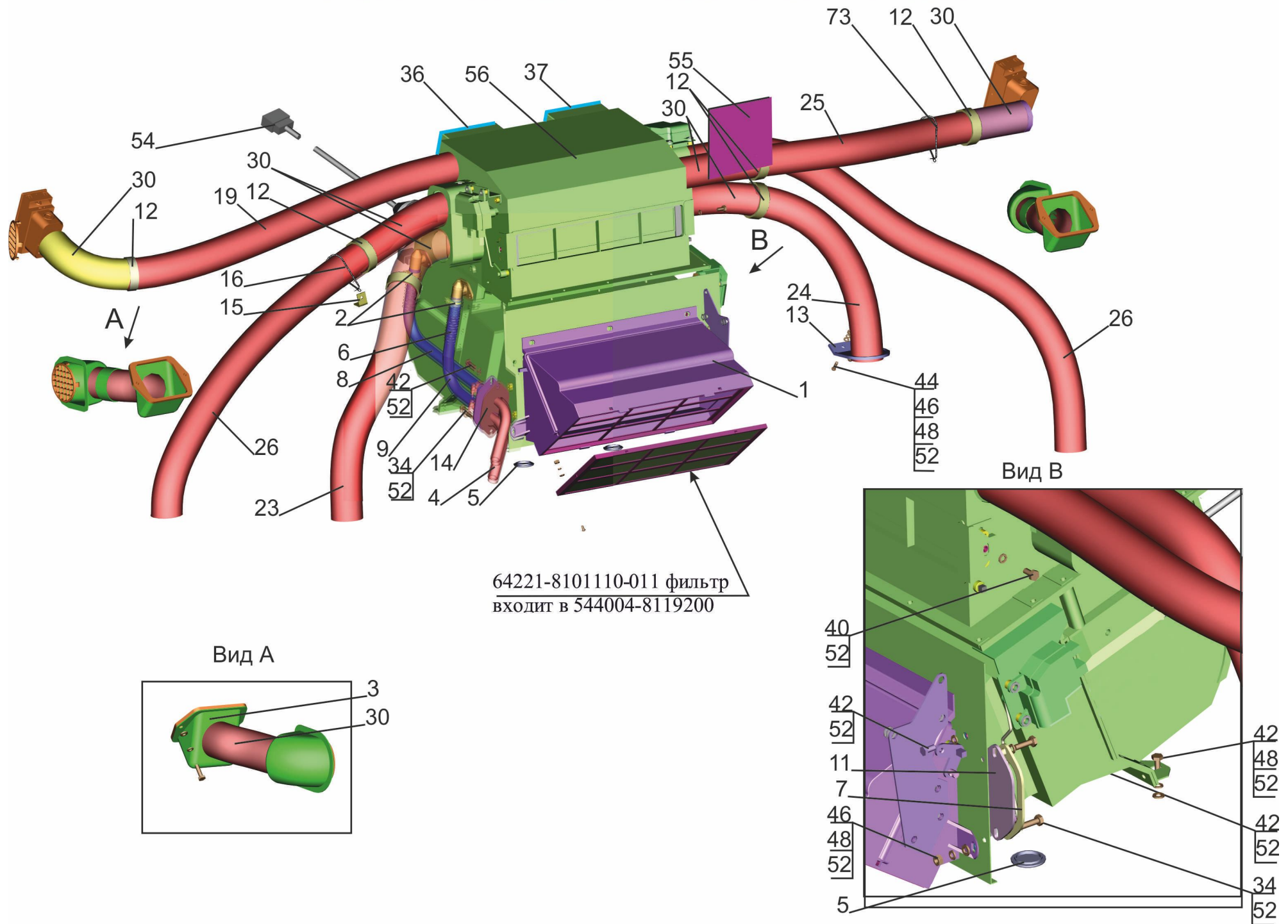
Fig. 283 Installation of heater 643008-8100001
