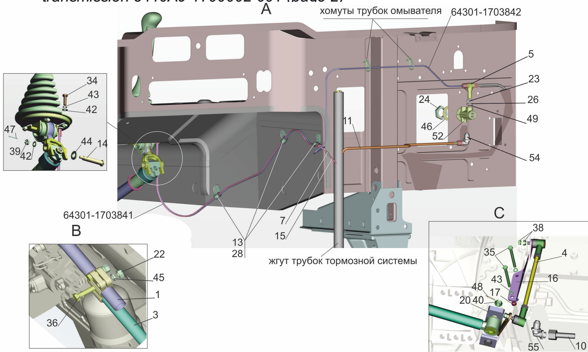
Fig. 48 Installation of drive of control of gear box and dual high transmission 5440A9-1700002-001 (page 2)
