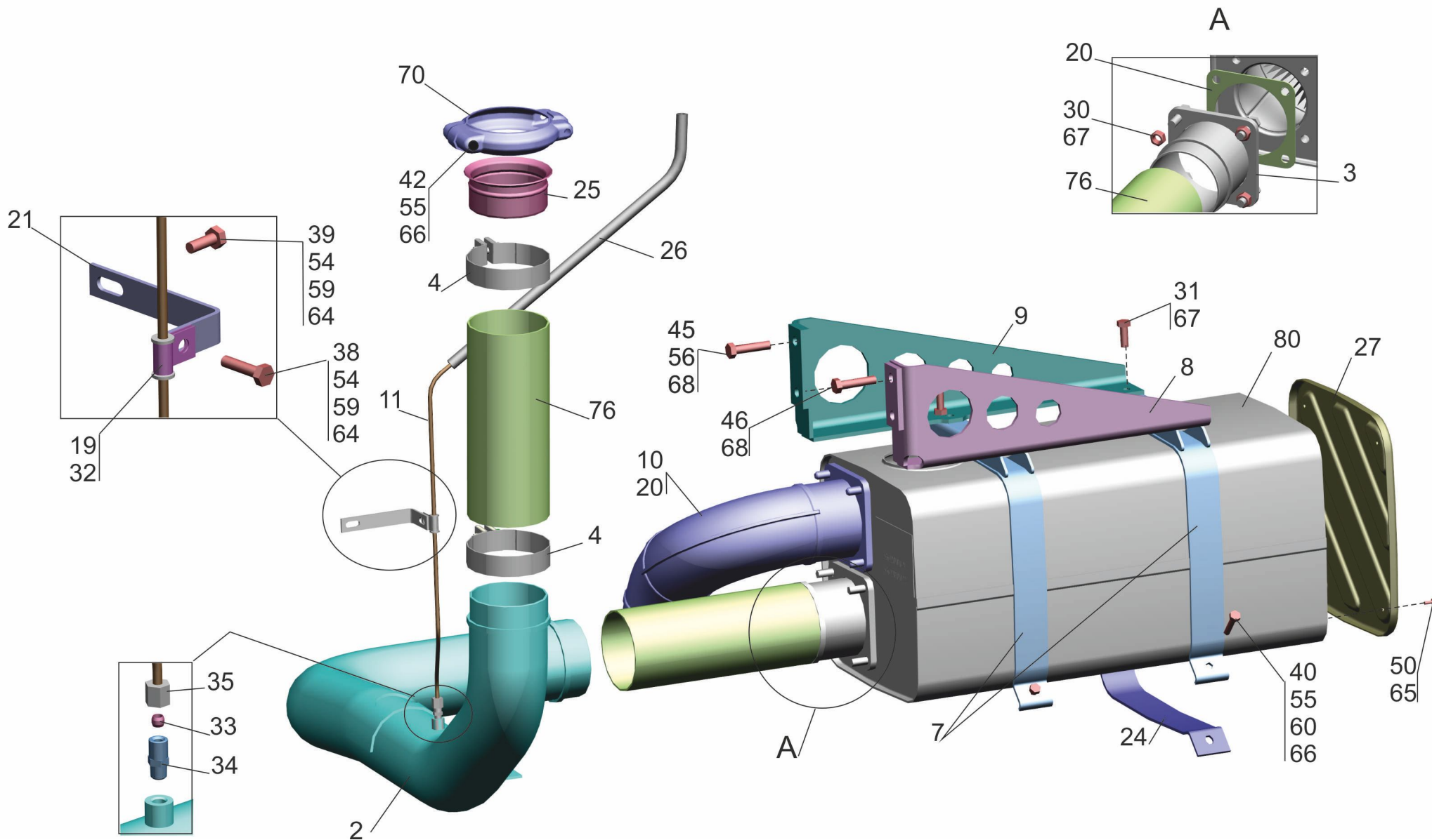
Fig. 32 Installing of gas release sistem 6501B9-1200001-020
