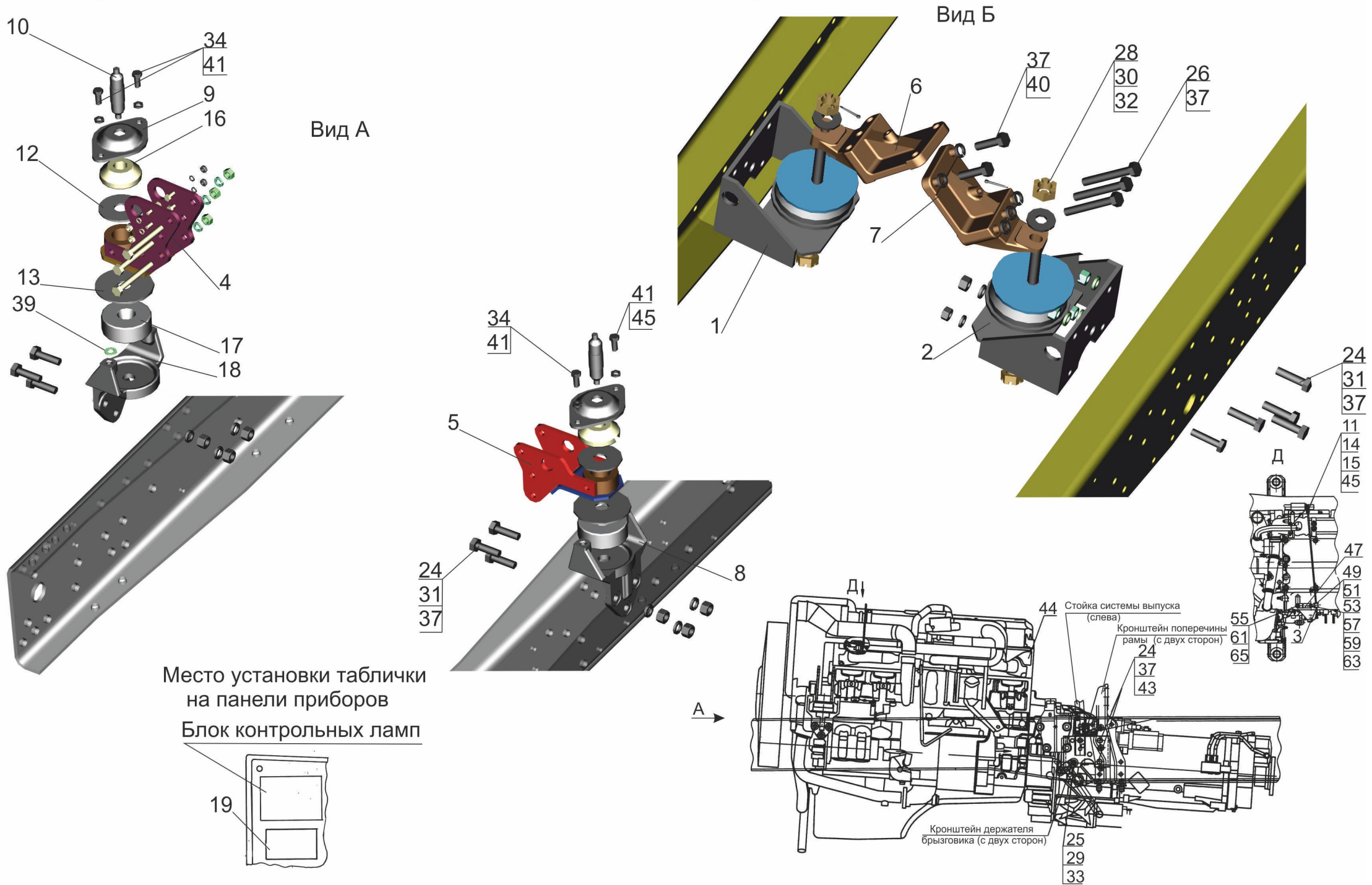
Рис.2 Крепление двигателя 6501B9-1001002-330, (-335,-350,-355, -360,-365, -380,-385) Fig.2 Mounting diesel 6501B9-1001002-330, (-335,-350,-355, -360,-365, -380,-385)
