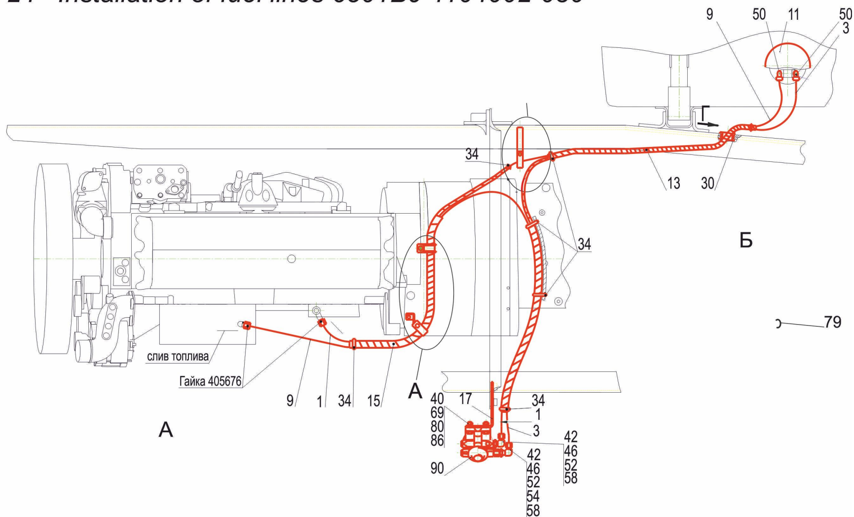
Fig. 24 Installation of fuel lines 6501B9-1104002-030
