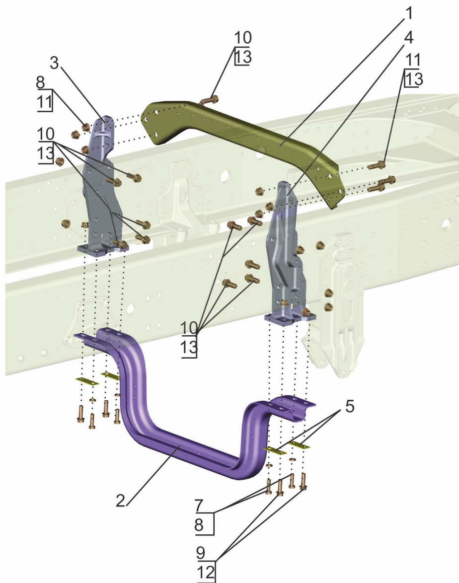
Рис.106 Установка пояса поперечин 6501B9-2800060-040 Fig.106 Installation of a belt of cross member 6501B9-2800060-040
