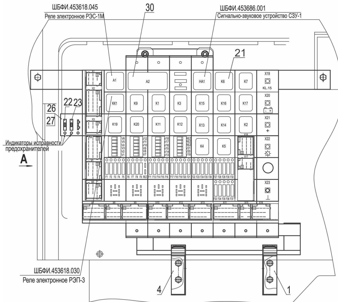
Рис. 206 Установка БКА-N4 6430A9-3700110-000 Fig.206 Installation of switchgear unit 6430A9-3700110-000
