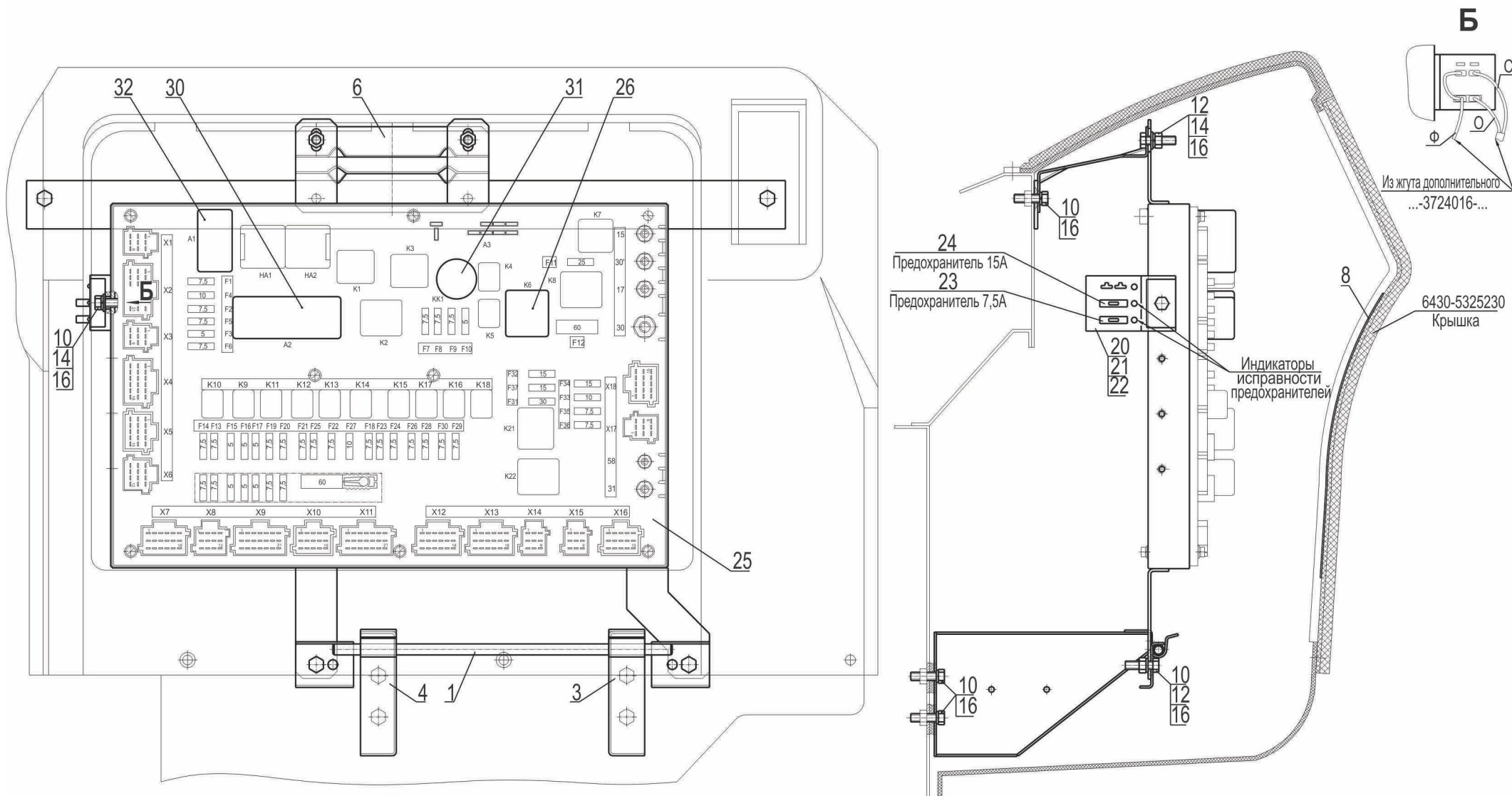
Рис.207 Установка БКА-N4 6430A9-3700110-001, (-701) Fig.207 Installation of switchgear unit 6430A9-3700110-001, (-701)
