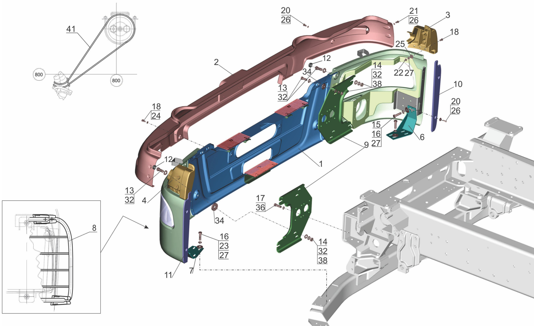
Fig. 97 Installation front bumper 6516V8-2800003-000
