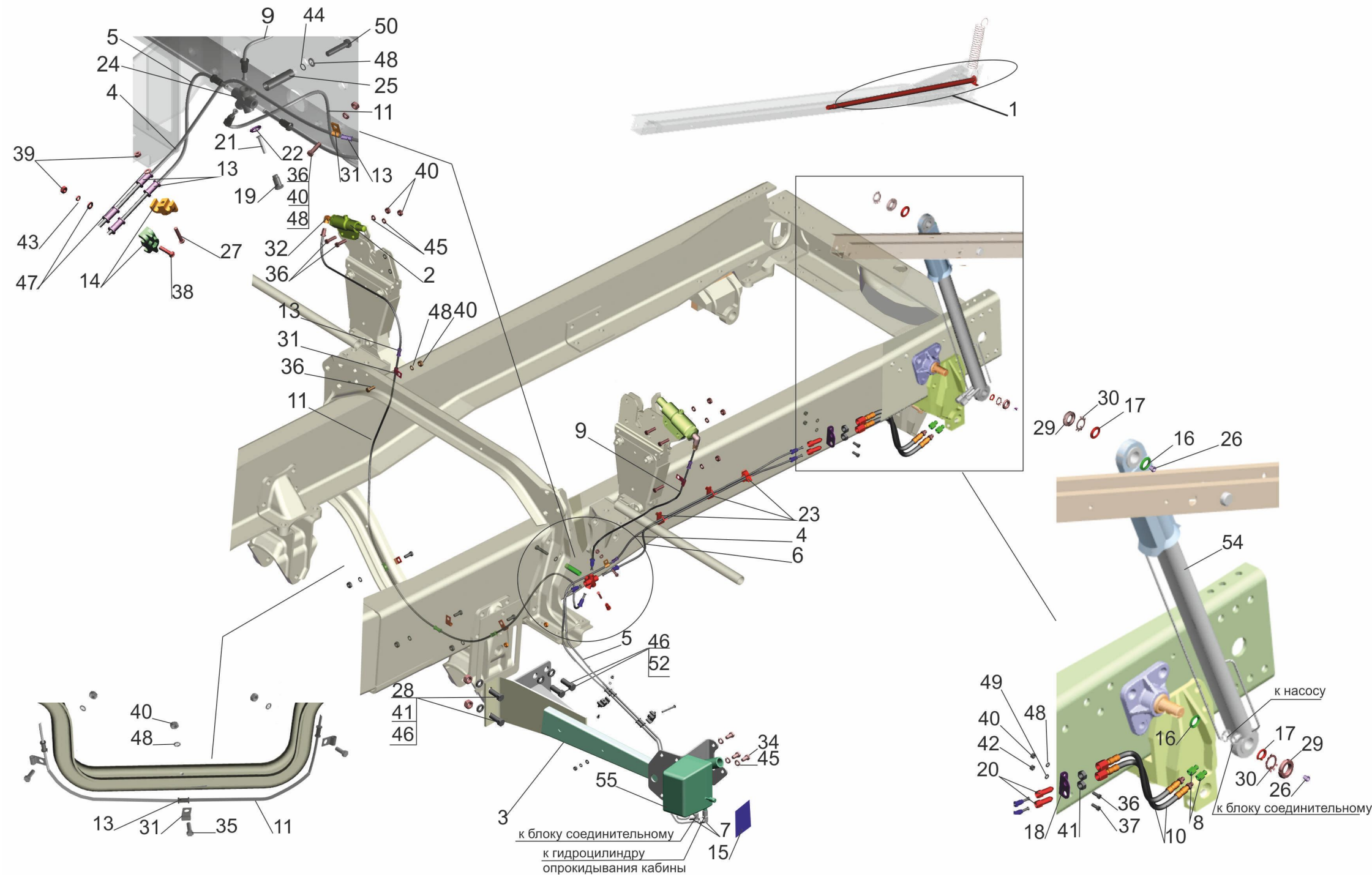
Fig. 276 Installation cab tilting mechanism 6501B9-5000040-010
