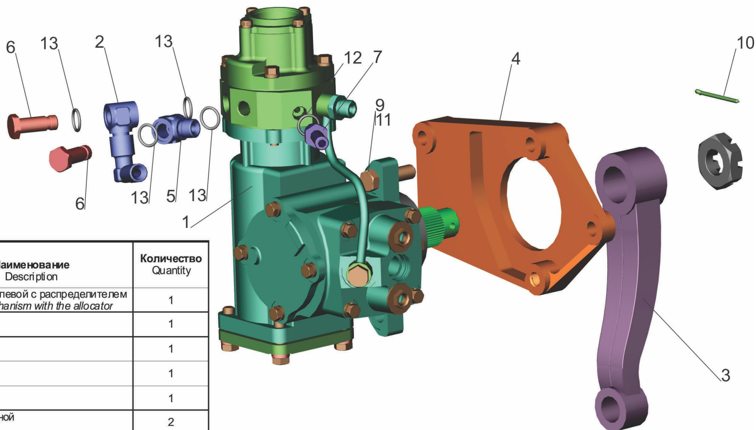
Fig. 148 Steering mechanism with bracket 6418-3400006
