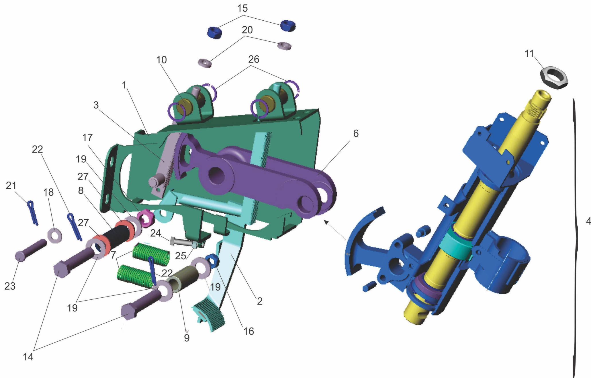
Fig. 158 Arm with a column 5440-3403008
